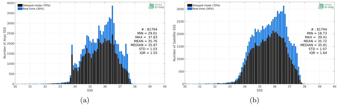
Figure 2: Histograms of SSS from Argo (a) and Aquarius-L3-OR-V5-7DAY-RUNNING-RAIN-MASK-1DEG (b) considering all match-up pairs per bins of 0.1 over the Atlantic Ocean Pi-MEP region and for the full satellite product period.
