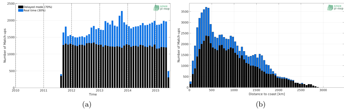
Figure 1: Number of match-ups between Argo and Aquarius-L3-OR-V5-7DAY-RUNNING-RAIN-MASK-1DEG SSS as a function of time (a) and as function of the distance to coast (b) over the Atlantic Ocean Pi-MEP region and for the full satellite product period.
