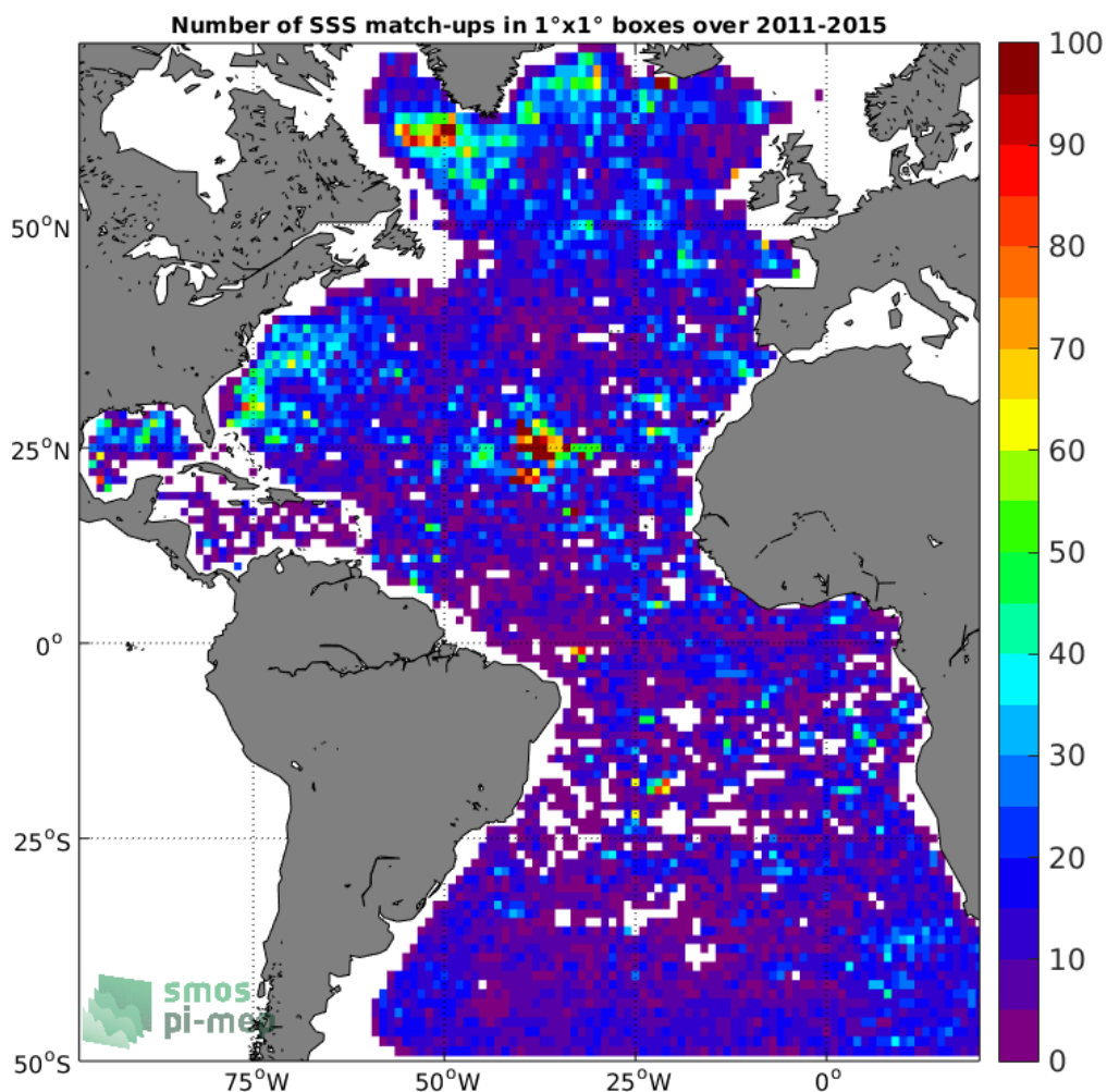
Figure 4: Number of SSS match-ups between Argo SSS and the Aquarius-L3-OR-V5-7DAY-RUNNING-RAIN-MASK-1DEG SSS product for the Atlantic Ocean Pi-MEP region over 1°x1° boxes and for the full satellite product period.
