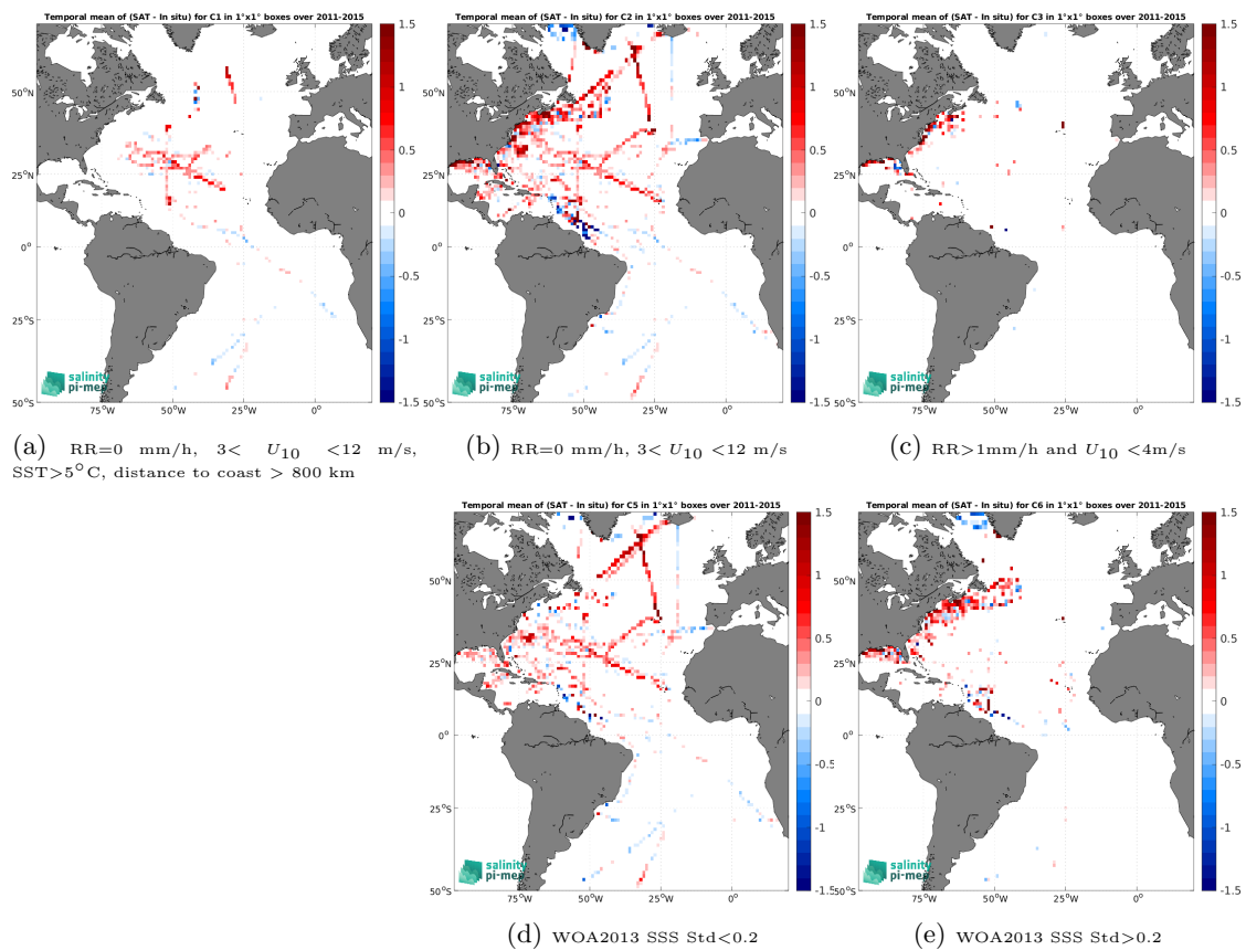
Figure 14: Temporal mean gridded over spatial boxes of size 1^\circ \times 1^\circ of \Delta SSS (Aquarius SSS L3 OR v5 - Monthly (NASA-GSFC) - TSG (SAMOS)) for 5 different subdatasets corresponding to:RR=0 mm/h, 3 < U_{10} < 12 m/s, SST >5^\circ\text{C} , distance to coast > 800 km (a), RR=0 mm/h, 3 < U_{10} < 12 m/s (b), RR >1 mm/h and U_{10} < 4 m/s (c), WOA2013 SSS Std <0.2 (d), WOA2013 SSS Std >0.2 (e).
