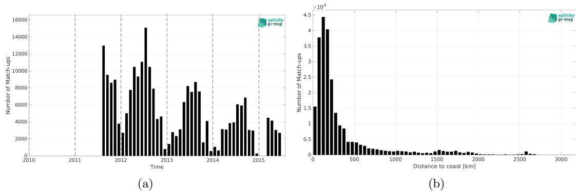
Figure 2: Number of match-ups between TSG (SAMOS) and Aquarius SSS L3 OR v5 - Monthly (NASA-GSFC) SSS as a function of time (a) and as function of the distance to coast (b) over the Atlantic Ocean Pi-MEP region and for the full satellite product period.
