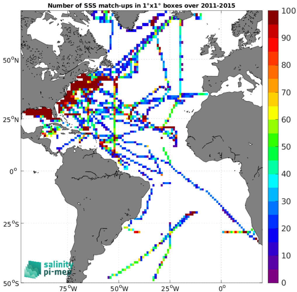
Figure 5: Number of SSS match-ups between TSG (SAMOS) SSS and the Aquarius SSS L3 OR v5 - Monthly (NASA-GSFC) SSS product for the Atlantic Ocean Pi-MEP region over 1^\circ \times 1^\circ boxes and for the full satellite product period.
