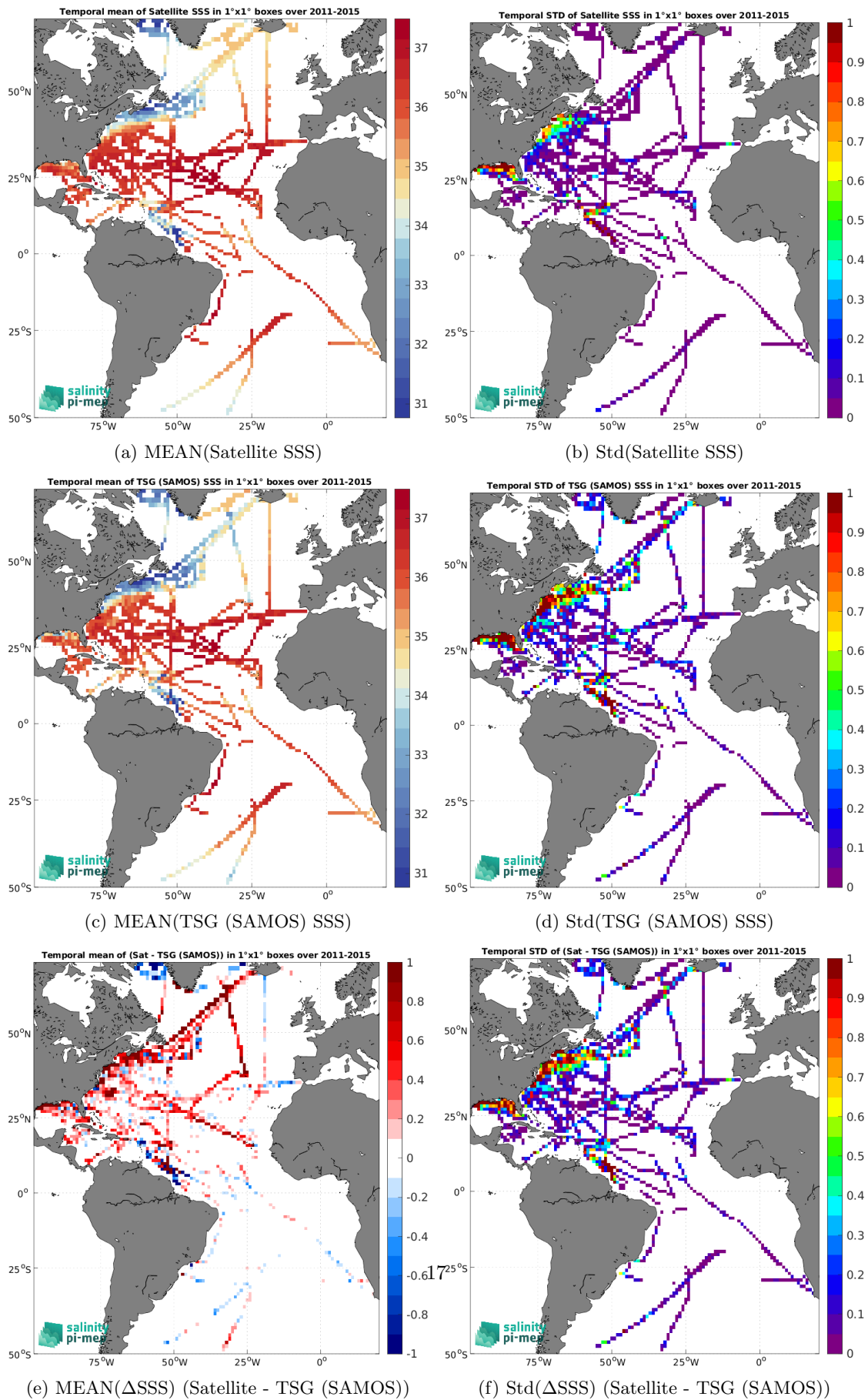
Figure 7: Temporal mean (left) and Std (right) of SSS from Aquarius SSS L3 OR v5 - Monthly (NASA-GSFC) (top), TSG (SAMOS) (middle), and of \Delta SSS (Satellite - TSG (SAMOS)). Only match-up pairs are used to generate these maps.
