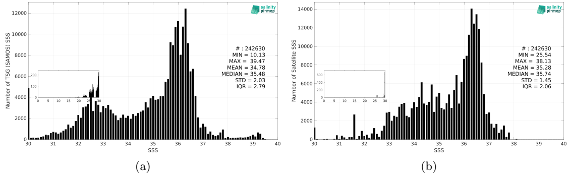
Figure 3: Histograms of SSS from TSG (SAMOS) (a) and Aquarius SSS L3 OR v5 - Monthly (NASA-GSFC) (b) considering all match-up pairs per bins of 0.1 over the Atlantic Ocean Pi-MEP region and for the full satellite product period.
