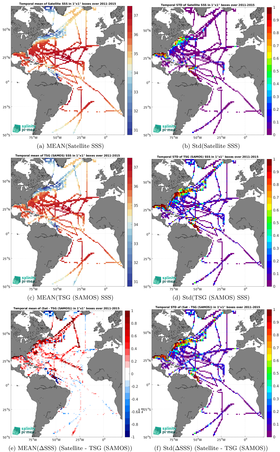
Figure 6: Temporal mean (left) and Std (right) of SSS from Aquarius SSS L3 OR v5 - Monthly (NASA-GSFC) (top), TSG (SAMOS) (middle), and of \Delta SSS (Satellite - TSG (SAMOS)). Only match-up pairs are used to generate these maps.
