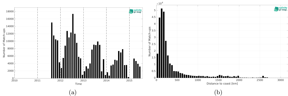
Figure 1: Number of match-ups between TSG (SAMOS) and Aquarius SSS L3 OR v5 - Monthly (NASA-GSFC) SSS as a function of time (a) and as function of the distance to coast (b) over the Atlantic Ocean Pi-MEP region and for the full satellite product period.
