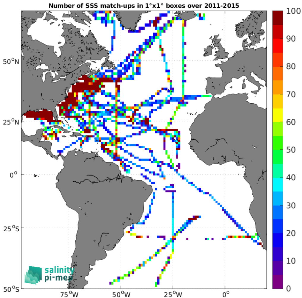
Figure 4: Number of SSS match-ups between TSG (SAMOS) SSS and the Aquarius SSS L3 OR v5 - Monthly (NASA-GSFC) SSS product for the Atlantic Ocean Pi-MEP region over 1^\circ \times 1^\circ boxes and for the full satellite product period.
