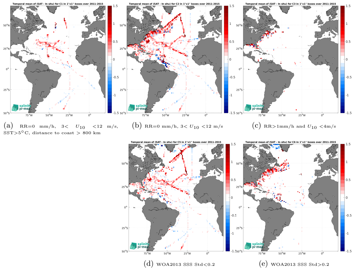
Figure 12: Temporal mean gridded over spatial boxes of size 1^\circ \times 1^\circ of \Delta SSS (Aquarius SSS L3 OR v5 - Monthly (NASA-GSFC) - TSG (SAMOS)) for 5 different subdatasets corresponding to:RR=0 mm/h, 3 < U_{10} < 12 m/s, SST >5^\circ\text{C} , distance to coast > 800 km (a), RR=0 mm/h, 3 < U_{10} < 12 m/s (b), RR >1 mm/h and U_{10} < 4 m/s (c), WOA2013 SSS Std <0.2 (d), WOA2013 SSS Std >0.2 (e).
