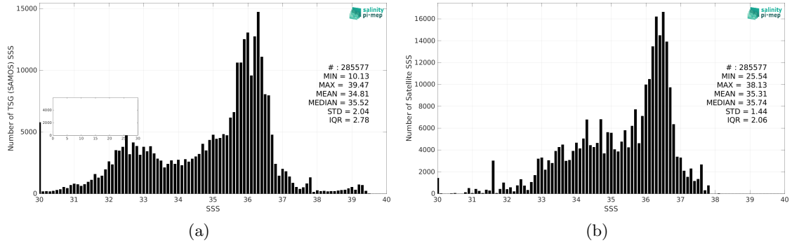
Figure 2: Histograms of SSS from TSG (SAMOS) (a) and Aquarius SSS L3 OR v5 - Monthly (NASA-GSFC) (b) considering all match-up pairs per bins of 0.1 over the Atlantic Ocean Pi-MEP region and for the full satellite product period.
