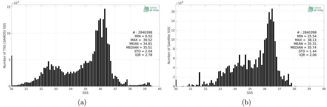
Figure 2: Histograms of SSS from TSG (SAMOS) (a) and Aquarius SSS L3 OR v5 - Monthly (NASA-GSFC) (b) considering all match-up pairs per bins of 0.1 over the Atlantic Ocean Pi-MEP region and for the full satellite product period.
