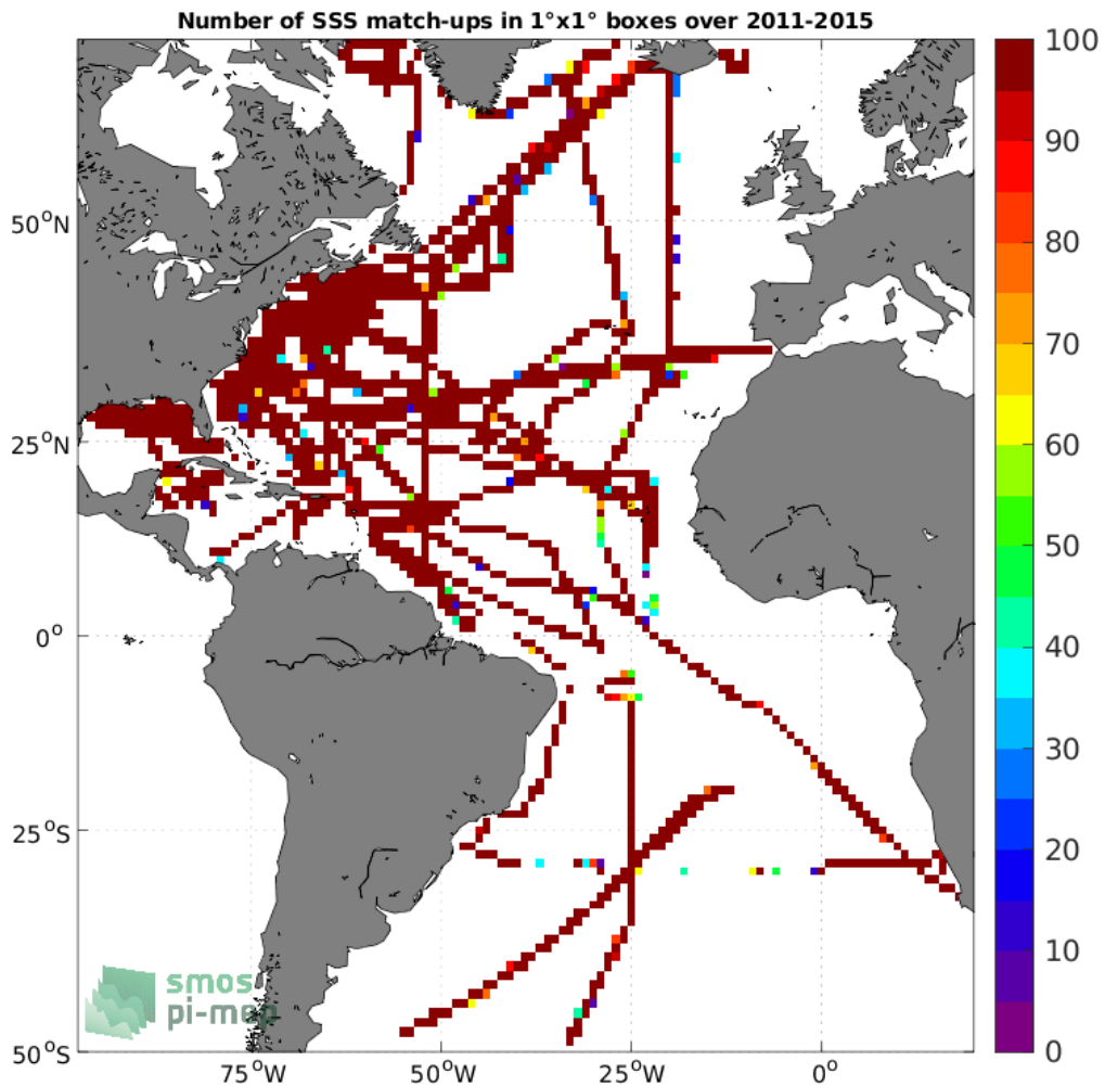
Figure 4: Number of SSS match-ups between TSG (SAMOS) SSS and the Aquarius SSS L3 OR v5 - Monthly (NASA-GSFC) SSS product for the Atlantic Ocean Pi-MEP region over 1°x1° boxes and for the full satellite product period.
