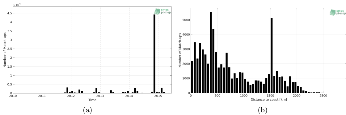
Figure 1: Number of match-ups between TSG-POLARSTERN and Aquarius-L3-OR-V5-MONTHLY-1DEG SSS as a function of time (a) and as function of the distance to coast (b) over the Atlantic Ocean Pi-MEP region and for the full satellite product period.
