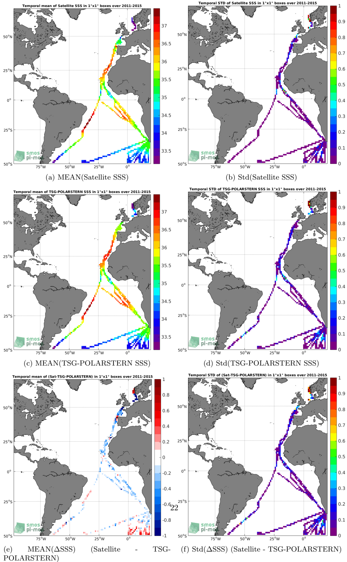
Figure 6: Temporal mean (left) and Std (right) of SSS from Aquarius-L3-OR-V5-MONTHLY-1DEG (top), TSG-POLARSTERN (middle), and of \Delta SSS (Satellite - TSG-POLARSTERN). Only match-up pairs are used to generate these maps.
