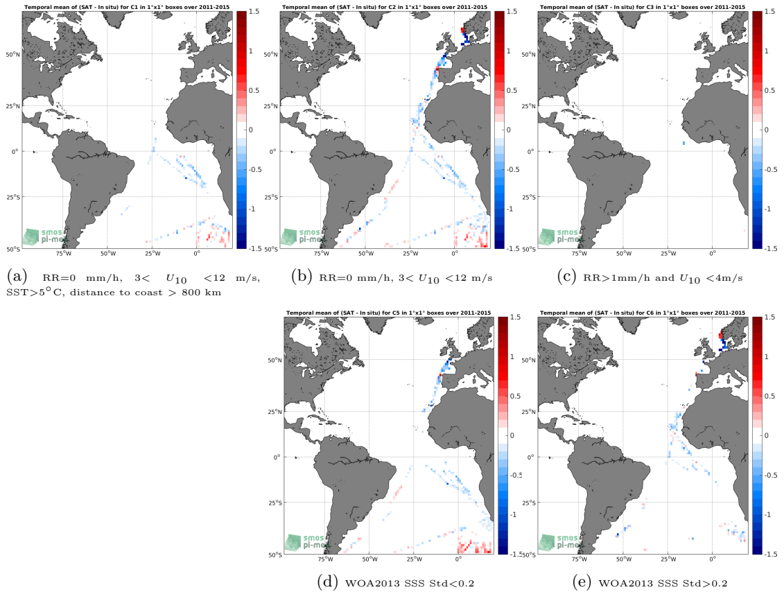
Figure 12: Temporal mean gridded over spatial boxes of size 1^\circ \times 1^\circ of \Delta SSS (Aquarius-L3-OR-V5-MONTHLY-1DEG - TSG-POLARSTERN) for 5 different subdatasets corresponding to:RR=0 mm/h, 3 < U_{10} < 12 m/s, SST >5^\circ C, distance to coast > 800 km (a), RR=0 mm/h, 3 < U_{10} < 12 m/s (b), RR >1 mm/h and U_{10} < 4 m/s (c), WOA2013 SSS Std <0.2 (d), WOA2013 SSS Std >0.2 (e).
