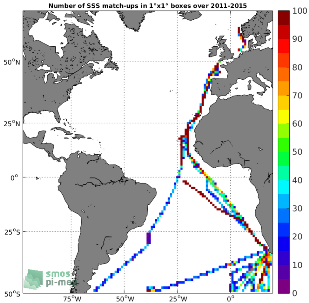
Figure 4: Number of SSS match-ups between TSG-POLARSTERN SSS and the Aquarius-L3-OR-V5-MONTHLY-1DEG SSS product for the Atlantic Ocean Pi-MEP region over 1°x1° boxes and for the full satellite product period.
