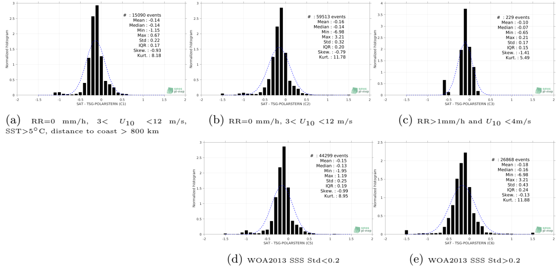
Figure 13: Normalized histogram of \Delta SSS (Aquarius-L3-OR-V5-MONTHLY-1DEG - TSG-POLARSTERN) for 5 different subdatasets corresponding to: RR=0 mm/h, 3 < U_{10} < 12 m/s, SST > 5°C, distance to coast > 800 km (a), RR=0 mm/h, 3 < U_{10} < 12 m/s (b), RR > 1mm/h and U_{10} < 4 m/s (c), WOA2013 SSS Std < 0.2 (d), WOA2013 SSS Std > 0.2 (e).
