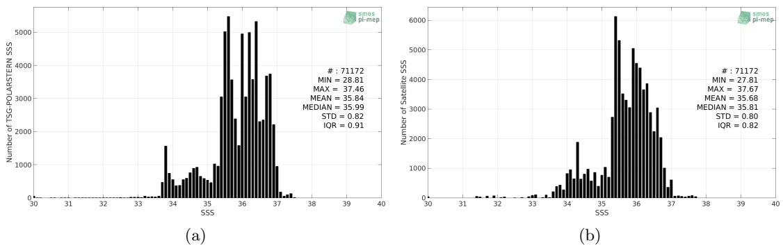
Figure 2: Histograms of SSS from TSG-POLARSTERN (a) and Aquarius-L3-OR-V5-MONTHLY-1DEG (b) considering all match-up pairs per bins of 0.1 over the Atlantic Ocean Pi-MEP region and for the full satellite product period.
