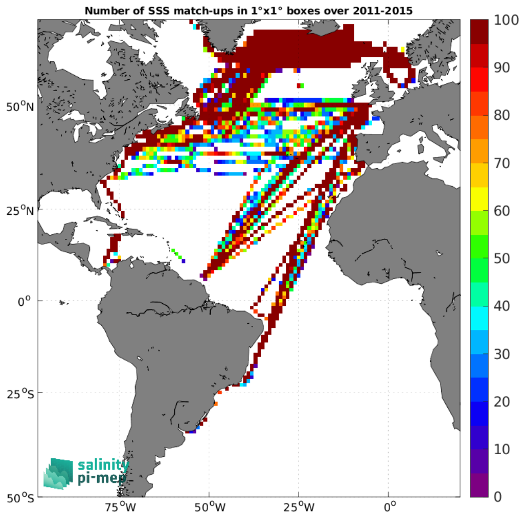
Figure 5: Number of SSS match-ups between TSG (LEGOS-DM) SSS and the Aquarius SSS L3 OR v5 - Monthly (NASA-GSFC) SSS product for the Atlantic Ocean Pi-MEP region over 1°×1° boxes and for the full satellite product period.
