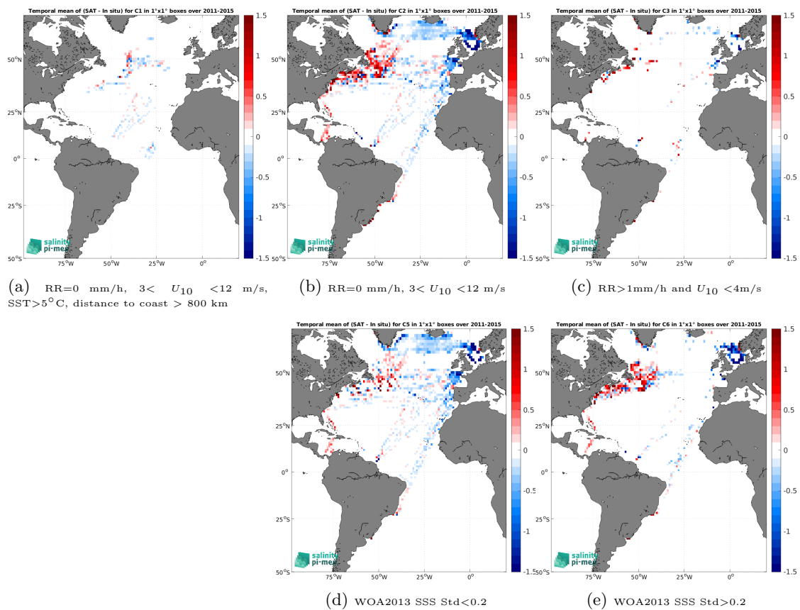
Figure 14: Temporal mean gridded over spatial boxes of size 1^\circ \times 1^\circ of \Delta\text{SSS} (Aquarius SSS L3 OR v5 - Monthly (NASA-GSFC) - TSG (LEGOS-DM)) for 5 different subdatasets corresponding to:RR=0 mm/h, 3 < U_{10} < 12 m/s, SST >5^\circ\text{C} , distance to coast > 800 km (a), RR=0 mm/h, 3 < U_{10} < 12 m/s (b), RR >1 mm/h and U_{10} < 4 m/s (c), WOA2013 SSS Std <0.2 (d), WOA2013 SSS Std >0.2 (e).
