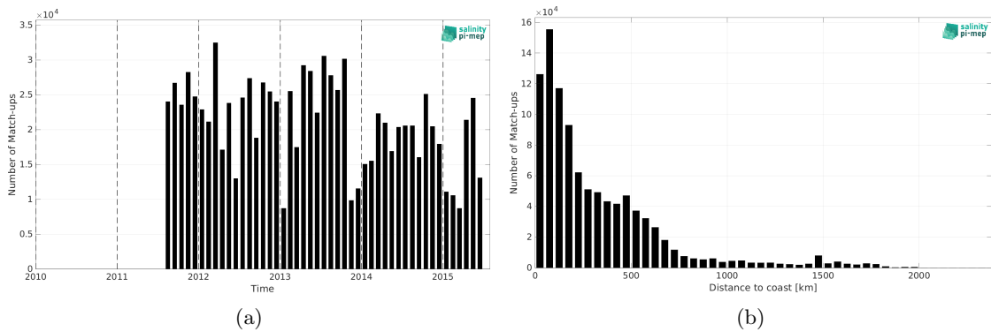
Figure 2: Number of match-ups between TSG (LEGOS-DM) and Aquarius SSS L3 OR v5 - Monthly (NASA-GSFC) SSS as a function of time (a) and as function of the distance to coast (b) over the Atlantic Ocean Pi-MEP region and for the full satellite product period.
