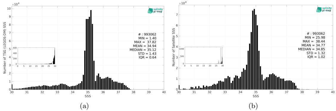
Figure 3: Histograms of SSS from TSG (LEGOS-DM) (a) and Aquarius SSS L3 OR v5 - Monthly (NASA-GSFC) (b) considering all match-up pairs per bins of 0.1 over the Atlantic Ocean Pi-MEP region and for the full satellite product period.
