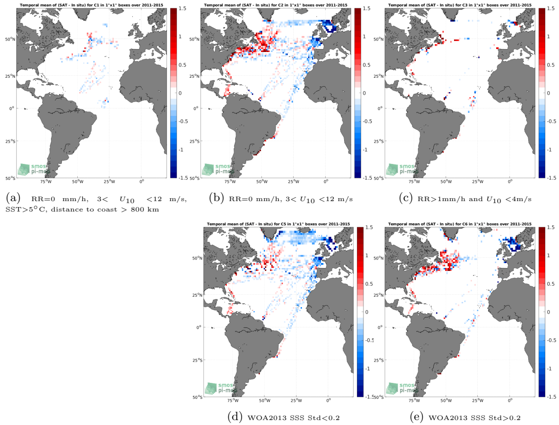
Figure 12: Temporal mean gridded over spatial boxes of size 1^\circ \times 1^\circ of \Delta SSS (Aquarius SSS L3 OR v5 - Monthly (NASA-GSFC) - TSG (LEGOS-DM)) for 5 different subdatasets corresponding to:RR=0 mm/h, 3 < U_{10} < 12 m/s, SST >5^\circ\text{C} , distance to coast > 800 km (a), RR=0 mm/h, 3 < U_{10} < 12 m/s (b), RR >1 mm/h and U_{10} < 4 m/s (c), WOA2013 SSS Std <0.2 (d), WOA2013 SSS Std >0.2 (e).
