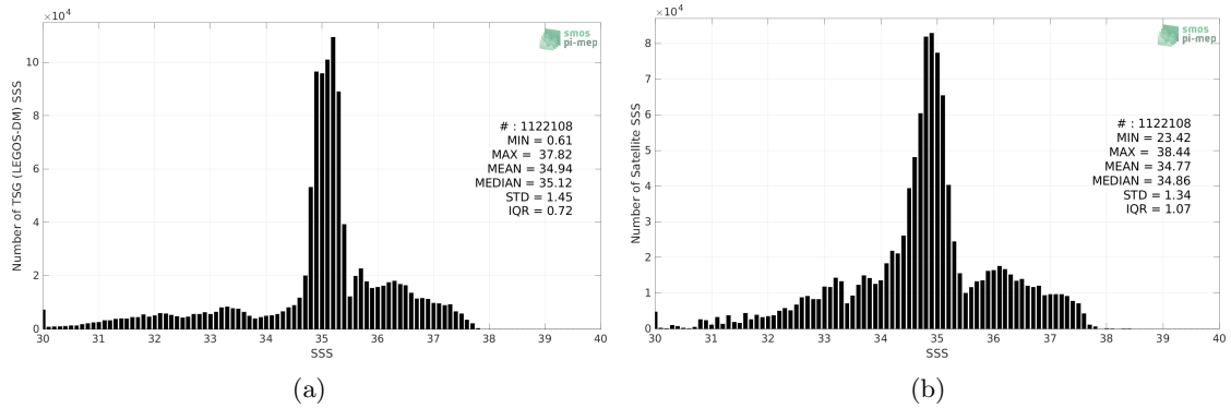
Figure 2: Histograms of SSS from TSG (LEGOS-DM) (a) and Aquarius SSS L3 OR v5 - Monthly (NASA-GSFC) (b) considering all match-up pairs per bins of 0.1 over the Atlantic Ocean Pi-MEP region and for the full satellite product period.
