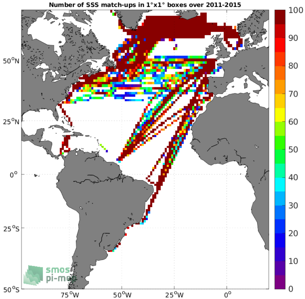
Figure 4: Number of SSS match-ups between TSG (LEGOS-DM) SSS and the Aquarius SSS L3 OR v5 - Monthly (NASA-GSFC) SSS product for the Atlantic Ocean Pi-MEP region over 1°x1° boxes and for the full satellite product period.
