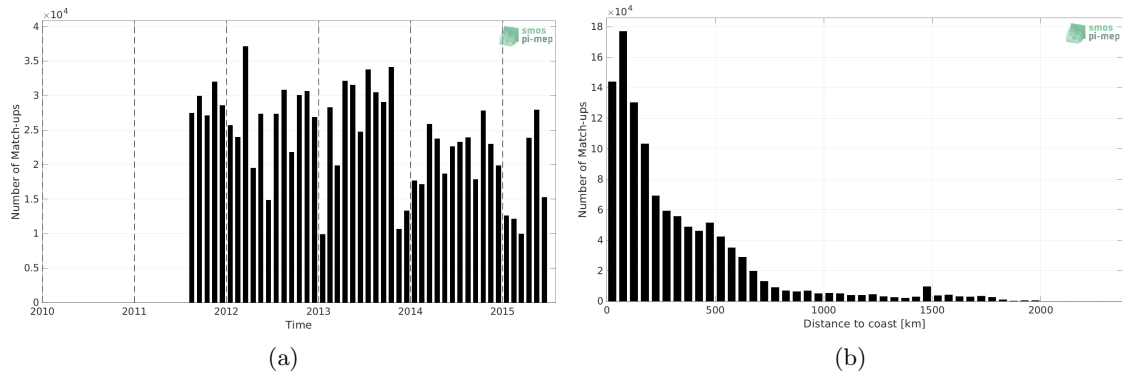
Figure 1: Number of match-ups between TSG (LEGOS-DM) and Aquarius SSS L3 OR v5 - Monthly (NASA-GSFC) SSS as a function of time (a) and as function of the distance to coast (b) over the Atlantic Ocean Pi-MEP region and for the full satellite product period.
