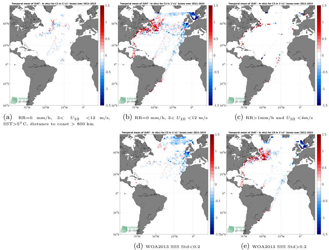
Figure 12: Temporal mean gridded over spatial boxes of size 1^\circ \times 1^\circ of \Delta SSS (Aquarius SSS L3 OR v5 - Monthly (NASA-GSFC) - TSG (LEGOS-DM)) for 5 different subdatasets corresponding to:RR=0 mm/h, 3 < U_{10} < 12 m/s, SST >5^\circ\text{C} , distance to coast > 800 km (a), RR=0 mm/h, 3 < U_{10} < 12 m/s (b), RR >1 mm/h and U_{10} < 4 m/s (c), WOA2013 SSS Std <0.2 (d), WOA2013 SSS Std >0.2 (e).
