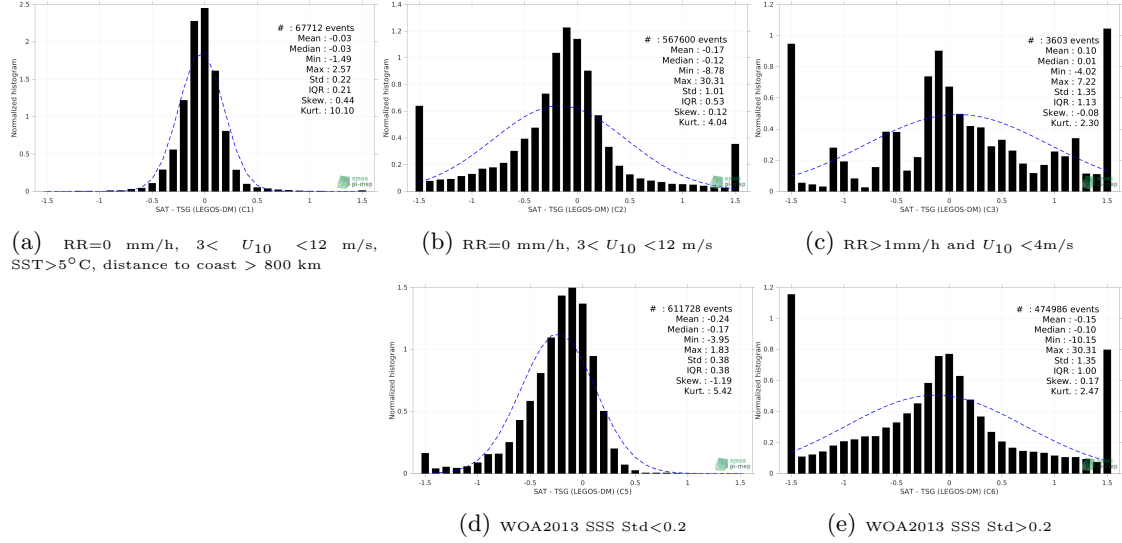
Figure 13: Normalized histogram of \Delta SSS (Aquarius SSS L3 OR v5 - Monthly (NASA-GSFC) - TSG (LEGOS-DM)) for 5 different subdatasets corresponding to: RR=0 mm/h, 3 < U_{10} < 12 m/s, SST > 5°C, distance to coast > 800 km (a), RR=0 mm/h, 3 < U_{10} < 12 m/s (b), RR > 1mm/h and U_{10} < 4 m/s (c), WOA2013 SSS Std < 0.2 (d), WOA2013 SSS Std > 0.2 (e).
