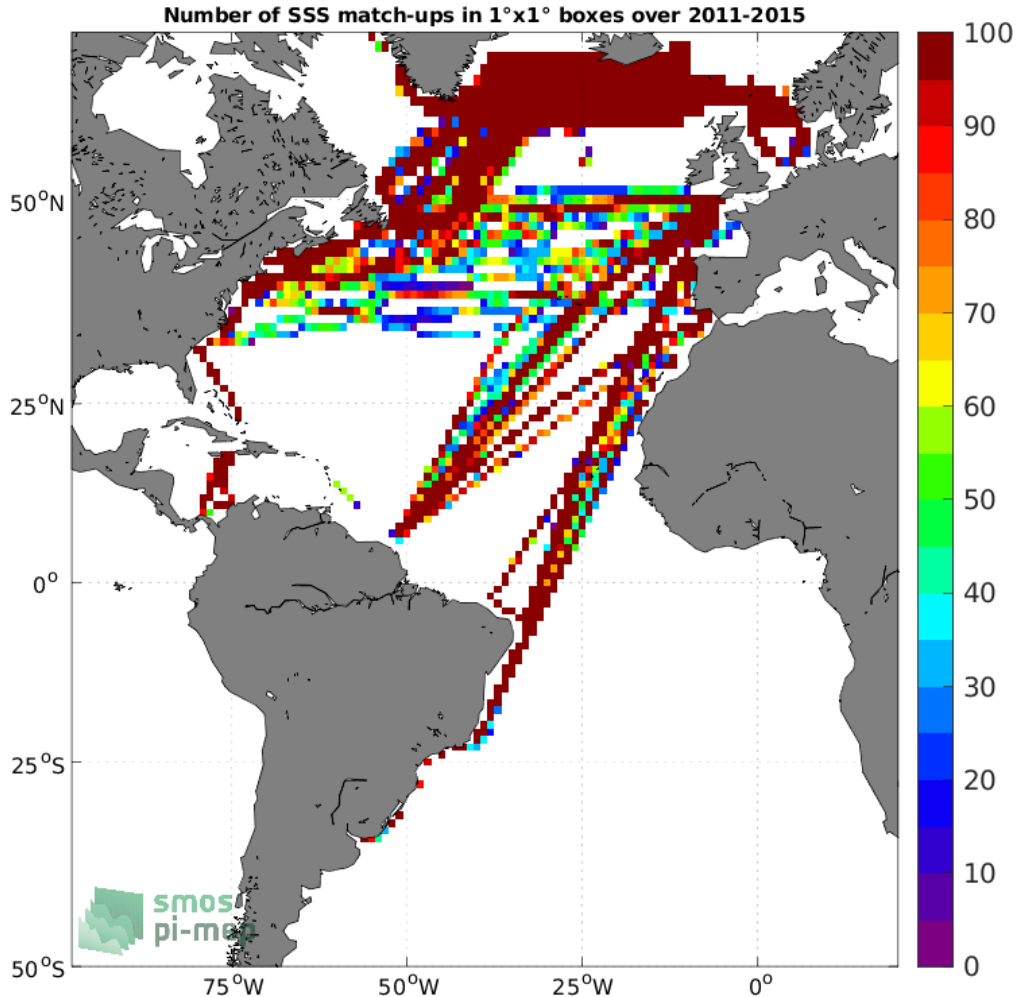
Figure 4: Number of SSS match-ups between TSG (LEGOS-DM) SSS and the Aquarius SSS L3 OR v5 - Monthly (NASA-GSFC) SSS product for the Atlantic Ocean Pi-MEP region over 1^\circ \times 1^\circ boxes and for the full satellite product period.
