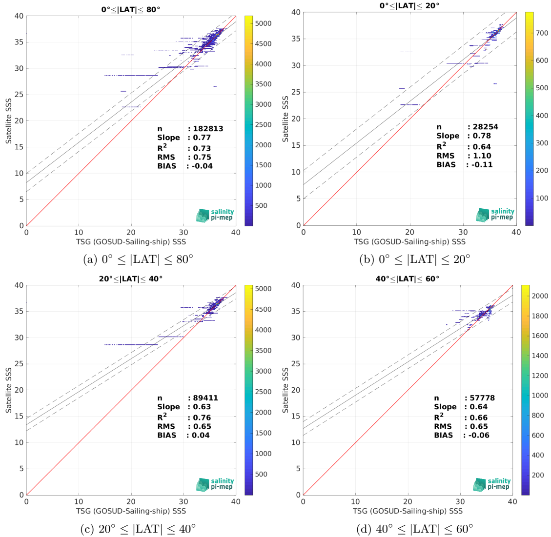
Figure 10: Contour maps of the concentration of Aquarius SSS L3 OR v5 - Monthly (NASA-GSFC) SSS ( y -axis) versus TSG (GOSUD-Sailing-ship) SSS ( x -axis) at match-up pairs for different latitude bands. For each plot, the red line shows x=y . The black thin and dashed lines indicate a linear fit through the data cloud and the \pm 95\% confidence levels, respectively. The number match-up pairs n , the slope and R^2 coefficient of the linear fit, the root mean square (RMS) and the mean bias between satellite and in situ data are indicated for each latitude band in each plots.
