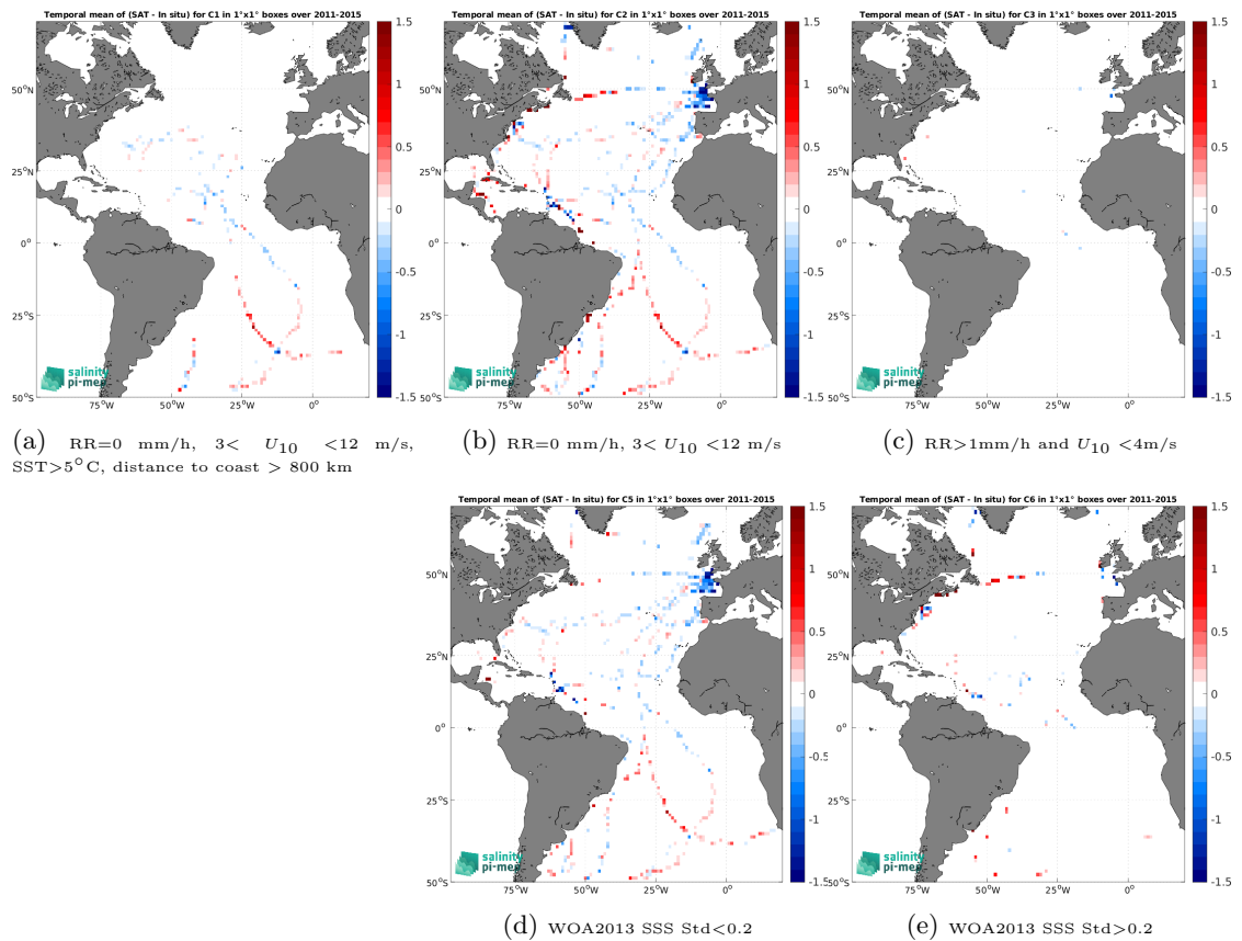
Figure 14: Temporal mean gridded over spatial boxes of size 1^\circ \times 1^\circ of \Delta\text{SSS} (Aquarius SSS L3 OR v5 - Monthly (NASA-GSFC) - TSG (GOSUD-Sailing-ship)) for 5 different subdatasets corresponding to:RR=0 mm/h, 3 < U_{10} < 12 m/s, SST>5°C, distance to coast > 800 km (a), RR=0 mm/h, 3 < U_{10} < 12 m/s (b), RR>1mm/h and U_{10} < 4 m/s (c), WOA2013 SSS Std<0.2 (d), WOA2013 SSS Std>0.2 (e).
