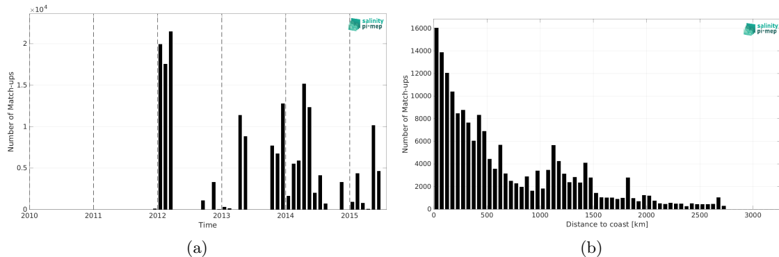
Figure 2: Number of match-ups between TSG (GOSUD-Sailing-ship) and Aquarius SSS L3 OR v5 - Monthly (NASA-GSFC) SSS as a function of time (a) and as function of the distance to coast (b) over the Atlantic Ocean Pi-MEP region and for the full satellite product period.
