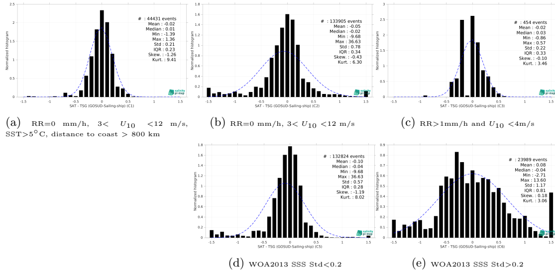
Figure 15: Normalized histogram of \Delta\text{SSS} (Aquarius SSS L3 OR v5 - Monthly (NASA-GSFC) - TSG (GOSUD-Sailing-ship)) for 5 different subdatasets corresponding to: RR=0 mm/h, 3 < U_{10} < 12 m/s, SST>5°C, distance to coast > 800 km (a), RR=0 mm/h, 3 < U_{10} < 12 m/s (b), RR>1mm/h and U_{10} < 4 m/s (c), WOA2013 SSS Std<0.2 (d), WOA2013 SSS Std>0.2 (e).
