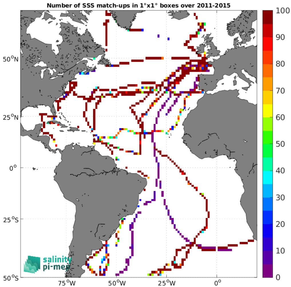
Figure 5: Number of SSS match-ups between TSG (GOSUD-Sailing-ship) SSS and the Aquarius SSS L3 OR v5 - Monthly (NASA-GSFC) SSS product for the Atlantic Ocean Pi-MEP region over 1^{\circ} \times 1^{\circ} boxes and for the full satellite product period.
