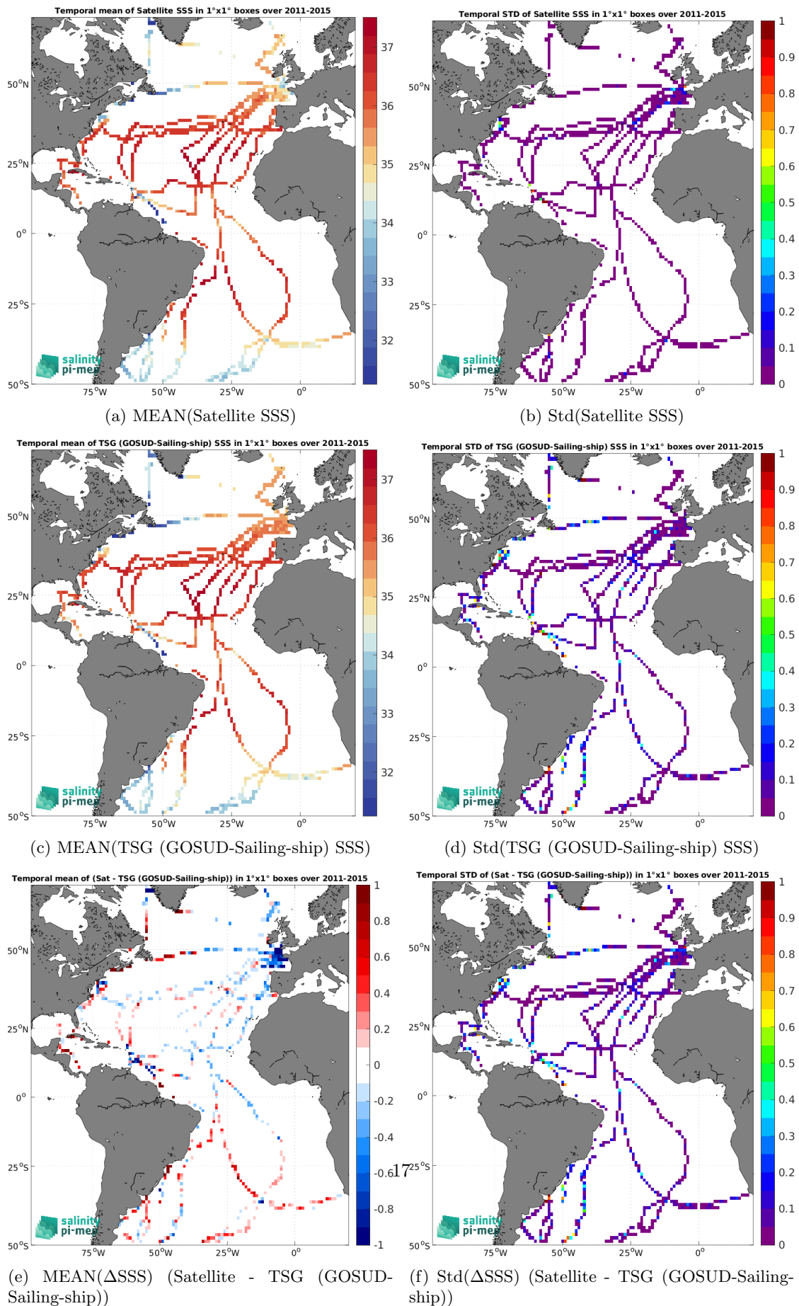
Figure 7: Temporal mean (left) and Std (right) of SSS from Aquarius SSS L3 OR v5 - Monthly (NASA-GSFC) (top), TSG (GOSUD-Sailing-ship) (middle), and of \Delta SSS (Satellite - TSG (GOSUD-Sailing-ship)). Only match-up pairs are used to generate these maps.
