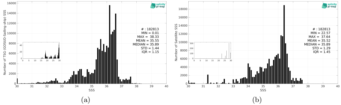
Figure 3: Histograms of SSS from TSG (GOSUD-Sailing-ship) (a) and Aquarius SSS L3 OR v5 - Monthly (NASA-GSFC) (b) considering all match-up pairs per bins of 0.1 over the Atlantic Ocean Pi-MEP region and for the full satellite product period.
