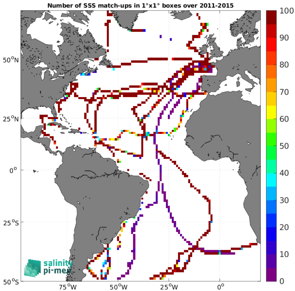
Figure 4: Number of SSS match-ups between TSG (GOSUD-Sailing-ship) SSS and the Aquarius SSS L3 OR v5 - Monthly (NASA-GSFC) SSS product for the Atlantic Ocean Pi-MEP region over 1^{\circ} \times 1^{\circ} boxes and for the full satellite product period.
