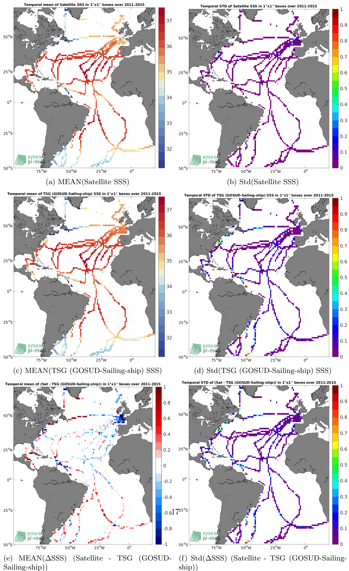
Figure 6: Temporal mean (left) and Std (right) of SSS from Aquarius SSS L3 OR v5 - Monthly (NASA-GSFC) (top), TSG (GOSUD-Sailing-ship) (middle), and of \Delta SSS (Satellite - TSG (GOSUD-Sailing-ship)). Only match-up pairs are used to generate these maps.
