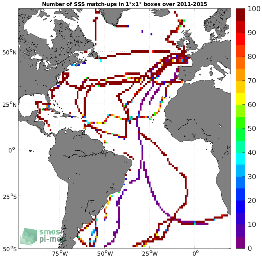
Figure 4: Number of SSS match-ups between TSG (GOSUD-Sailing-ship) SSS and the Aquarius SSS L3 OR v5 - Monthly (NASA-GSFC) SSS product for the Atlantic Ocean Pi-MEP region over 1°x1° boxes and for the full satellite product period.
