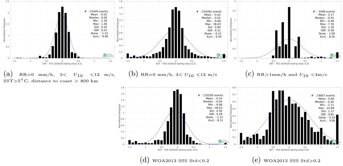
Figure 13: Normalized histogram of \Delta SSS (Aquarius SSS L3 OR v5 - Monthly (NASA-GSFC) - TSG (GOSUD-Sailing-ship)) for 5 different subdatasets corresponding to: RR=0 mm/h, 3 < U_{10} < 12 m/s, SST>5°C, distance to coast > 800 km (a), RR=0 mm/h, 3 < U_{10} < 12 m/s (b), RR>1mm/h and U_{10} < 4 m/s (c), WOA2013 SSS Std<0.2 (d), WOA2013 SSS Std>0.2 (e).
