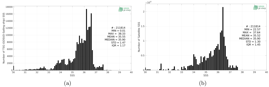
Figure 2: Histograms of SSS from TSG (GOSUD-Sailing-ship) (a) and Aquarius SSS L3 OR v5 - Monthly (NASA-GSFC) (b) considering all match-up pairs per bins of 0.1 over the Atlantic Ocean Pi-MEP region and for the full satellite product period.
