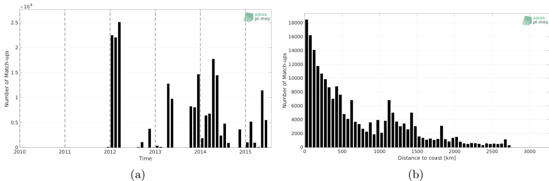
Figure 1: Number of match-ups between TSG (GOSUD-Sailing-ship) and Aquarius SSS L3 OR v5 - Monthly (NASA-GSFC) SSS as a function of time (a) and as function of the distance to coast (b) over the Atlantic Ocean Pi-MEP region and for the full satellite product period.
