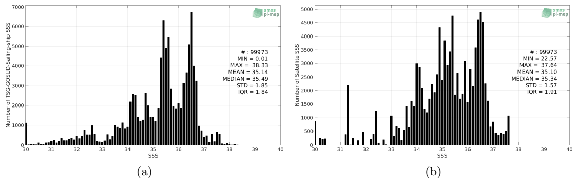
Figure 2: Histograms of SSS from TSG-GOSUD-Sailing-ship (a) and Aquarius-L3-OR-V5-MONTHLY-1DEG (b) considering all match-up pairs per bins of 0.1 over the Atlantic Ocean Pi-MEP region and for the full satellite product period.
