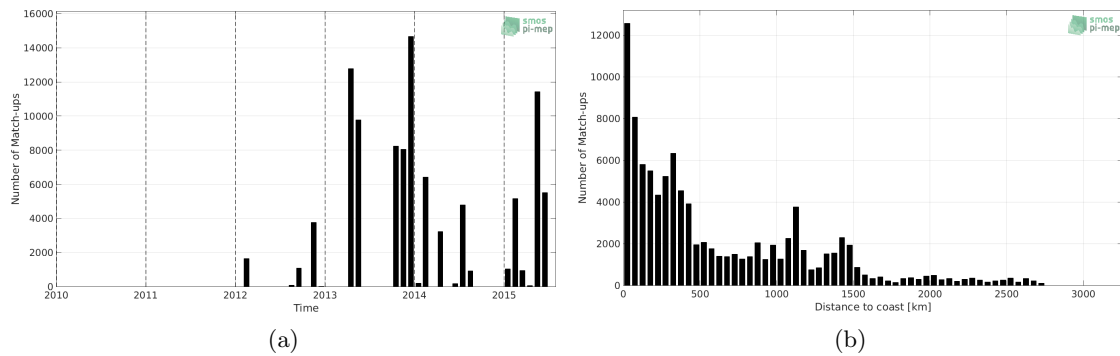
Figure 1: Number of match-ups between TSG-GOSUD-Sailing-ship and Aquarius-L3-OR-V5-MONTHLY-1DEG SSS as a function of time (a) and as function of the distance to coast (b) over the Atlantic Ocean Pi-MEP region and for the full satellite product period.
