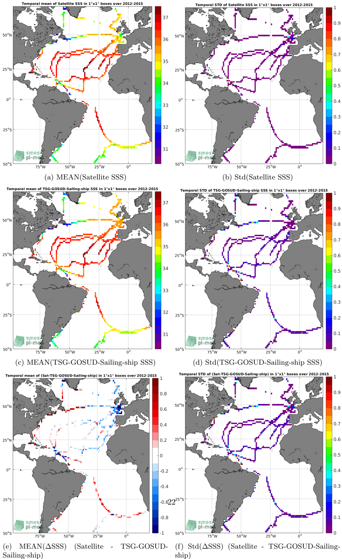
Figure 6: Temporal mean (left) and Std (right) of SSS from Aquarius-L3-OR-V5-MONTHLY-1DEG (top), TSG-GOSUD-Sailing-ship (middle), and of \Delta SSS (Satellite - TSG-GOSUD-Sailing-ship). Only match-up pairs are used to generate these maps.
