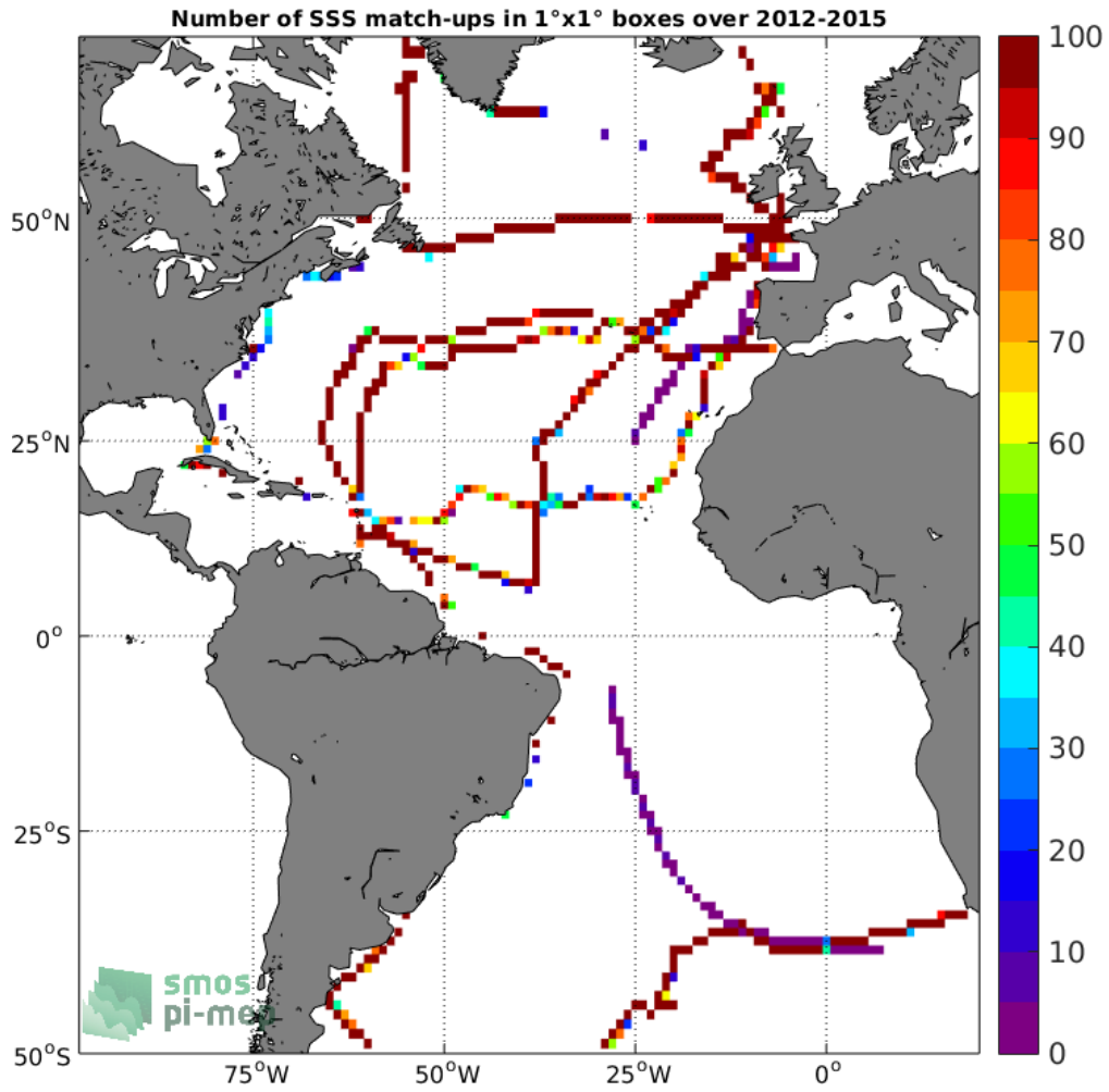
Figure 4: Number of SSS match-ups between TSG-GOSUD-Sailing-ship SSS and the Aquarius-L3-OR-V5-MONTHLY-1DEG SSS product for the Atlantic Ocean Pi-MEP region over 1°x1° boxes and for the full satellite product period.
