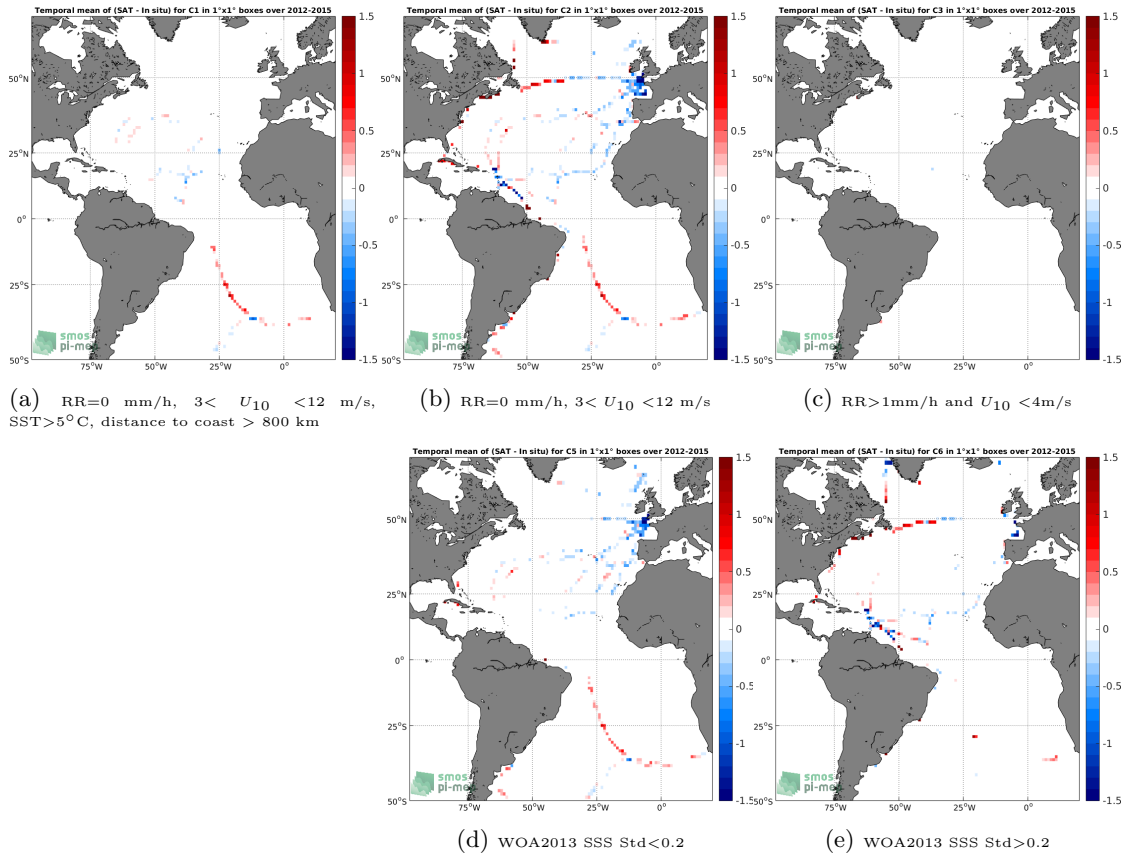
Figure 12: Temporal mean gridded over spatial boxes of size 1^\circ \times 1^\circ of \Delta SSS (Aquarius-L3-OR-V5-MONTHLY-1DEG - TSG-GOSUD-Sailing-ship) for 5 different subdatasets corresponding to:RR=0 mm/h, 3 < U_{10} < 12 m/s, SST >5^\circ C, distance to coast > 800 km (a), RR=0 mm/h, 3 < U_{10} < 12 m/s (b), RR >1 mm/h and U_{10} < 4 m/s (c), WOA2013 SSS Std <0.2 (d), WOA2013 SSS Std >0.2 (e).
