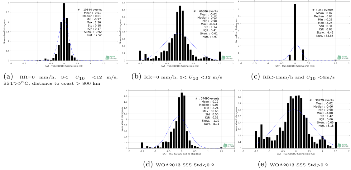
Figure 13: Normalized histogram of \Delta SSS (Aquarius-L3-OR-V5-MONTHLY-1DEG - TSG-GOSUD-Sailing-ship) for 5 different subdatasets corresponding to: RR=0 mm/h, 3 < U_{10} < 12 m/s, SST>5°C, distance to coast > 800 km (a), RR=0 mm/h, 3 < U_{10} < 12 m/s (b), RR>1mm/h and U_{10} < 4 m/s (c), WOA2013 SSS Std<0.2 (d), WOA2013 SSS Std>0.2 (e).
