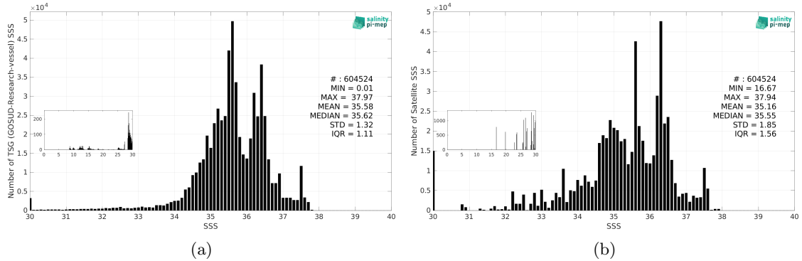
Figure 3: Histograms of SSS from TSG (GOSUD-Research-vessel) (a) and Aquarius SSS L3 OR v5 - Monthly (NASA-GSFC) (b) considering all match-up pairs per bins of 0.1 over the Atlantic Ocean Pi-MEP region and for the full satellite product period.
