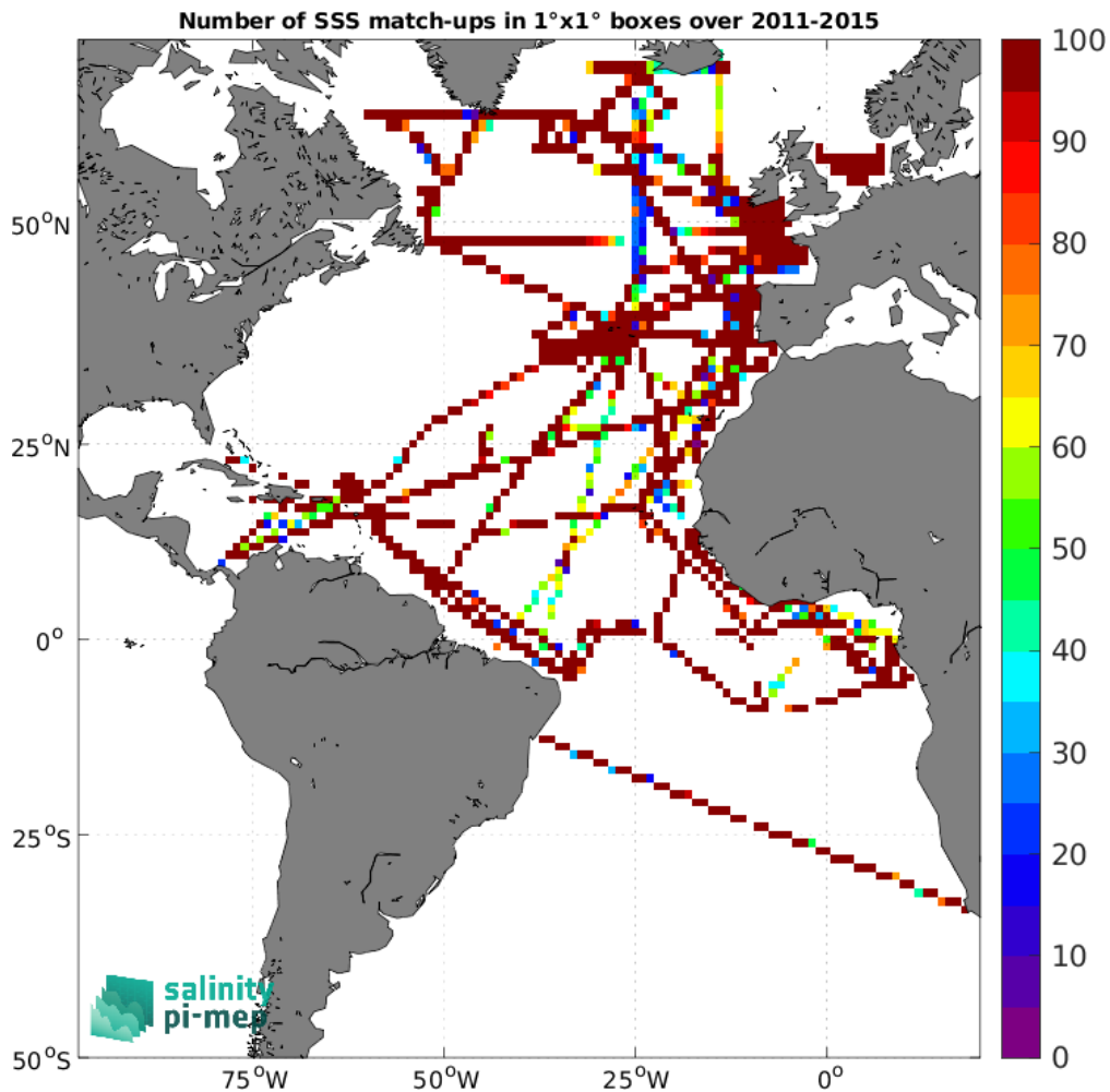
Figure 5: Number of SSS match-ups between TSG (GOSUD-Research-vessel) SSS and the Aquarius SSS L3 OR v5 - Monthly (NASA-GSFC) SSS product for the Atlantic Ocean Pi-MEP region over 1^\circ \times 1^\circ boxes and for the full satellite product period.
