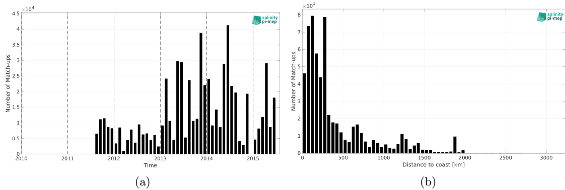
Figure 2: Number of match-ups between TSG (GOSUD-Research-vessel) and Aquarius SSS L3 OR v5 - Monthly (NASA-GSFC) SSS as a function of time (a) and as function of the distance to coast (b) over the Atlantic Ocean Pi-MEP region and for the full satellite product period.
