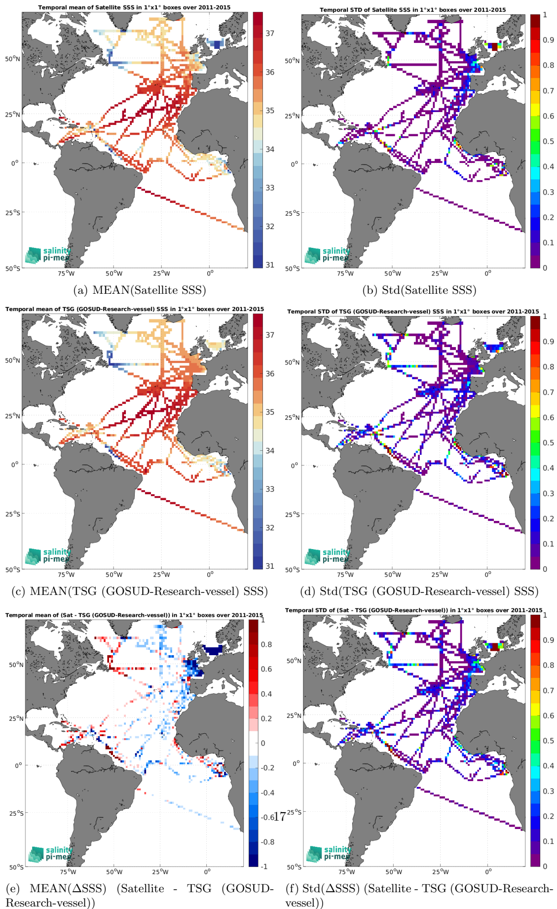
Figure 7: Temporal mean (left) and Std (right) of SSS from Aquarius SSS L3 OR v5 - Monthly (NASA-GSFC) (top), TSG (GOSUD-Research-vessel) (middle), and of \Delta SSS (Satellite - TSG (GOSUD-Research-vessel)). Only match-up pairs are used to generate these maps.
