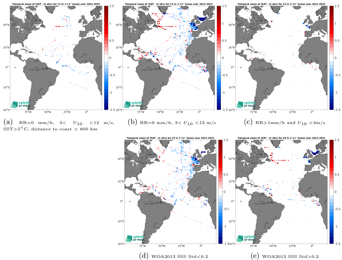
Figure 14: Temporal mean gridded over spatial boxes of size 1^\circ \times 1^\circ of \Delta\text{SSS} (Aquarius SSS L3 OR v5 - Monthly (NASA-GSFC) - TSG (GOSUD-Research-vessel)) for 5 different subdatasets corresponding to:RR=0 mm/h, 3 < U_{10} < 12 m/s, SST>5°C, distance to coast > 800 km (a), RR=0 mm/h, 3 < U_{10} < 12 m/s (b), RR>1mm/h and U_{10} < 4 m/s (c), WOA2013 SSS Std<0.2 (d), WOA2013 SSS Std>0.2 (e).
