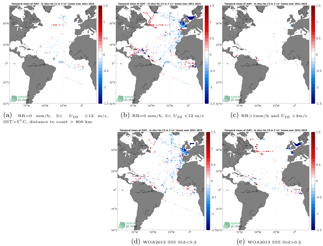
Figure 12: Temporal mean gridded over spatial boxes of size 1^\circ \times 1^\circ of \Delta\text{SSS} (Aquarius SSS L3 OR v5 - Monthly (NASA-GSFC) - TSG (GOSUD-Research-vessel)) for 5 different subdatasets corresponding to:RR=0 mm/h, 3 < U_{10} < 12 m/s, SST>5°C, distance to coast > 800 km (a), RR=0 mm/h, 3 < U_{10} < 12 m/s (b), RR>1mm/h and U_{10} < 4 m/s (c), WOA2013 SSS Std<0.2 (d), WOA2013 SSS Std>0.2 (e).
