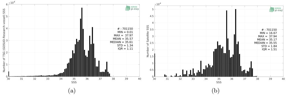
Figure 2: Histograms of SSS from TSG (GOSUD-Research-vessel) (a) and Aquarius SSS L3 OR v5 - Monthly (NASA-GSFC) (b) considering all match-up pairs per bins of 0.1 over the Atlantic Ocean Pi-MEP region and for the full satellite product period.
