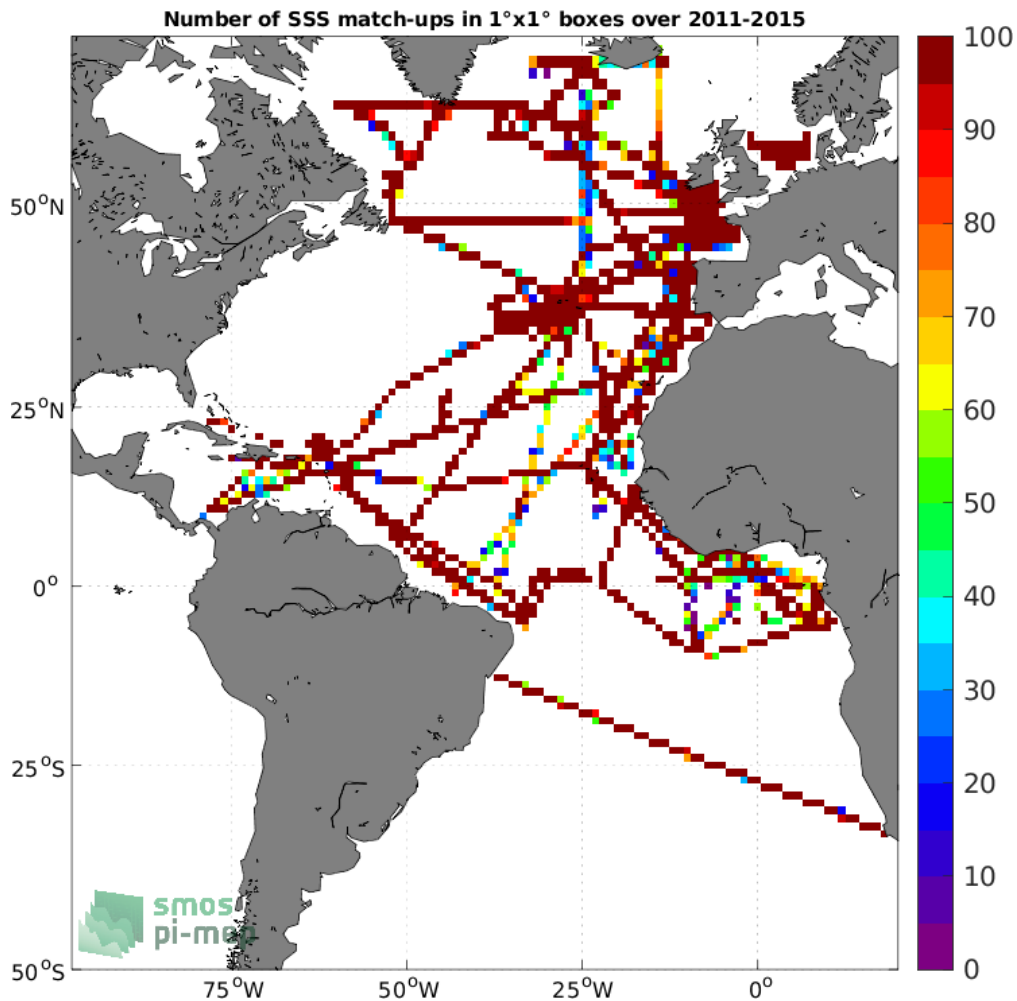
Figure 4: Number of SSS match-ups between TSG (GOSUD-Research-vessel) SSS and the Aquarius SSS L3 OR v5 - Monthly (NASA-GSFC) SSS product for the Atlantic Ocean Pi-MEP region over 1°x1° boxes and for the full satellite product period.
