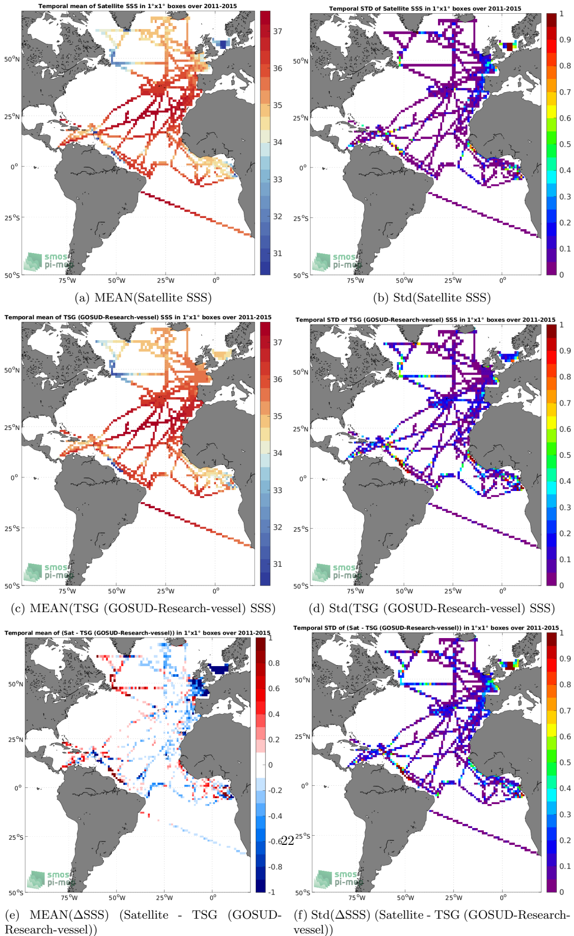
Figure 6: Temporal mean (left) and Std (right) of SSS from Aquarius SSS L3 OR v5 - Monthly (NASA-GSFC) (top), TSG (GOSUD-Research-vessel) (middle), and of \Delta SSS (Satellite - TSG (GOSUD-Research-vessel)). Only match-up pairs are used to generate these maps.
