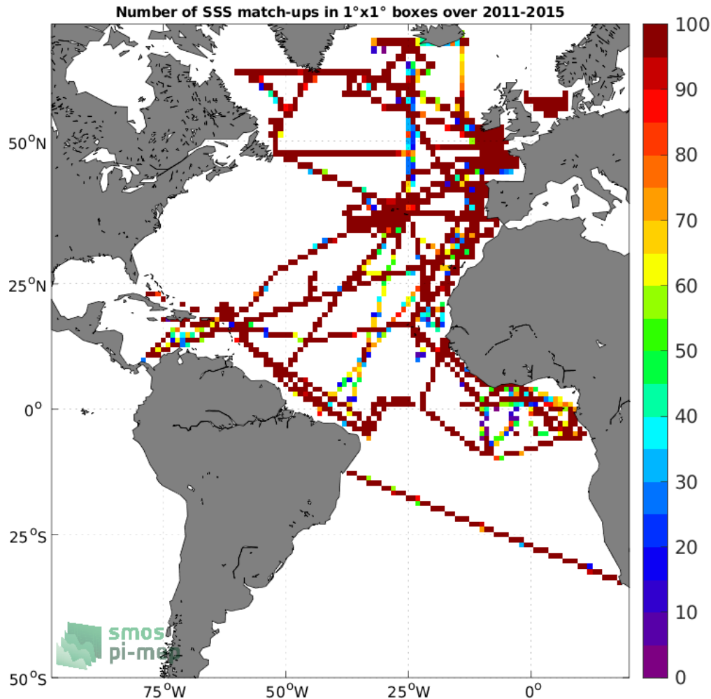
Figure 4: Number of SSS match-ups between TSG (GOSUD-Research-vessel) SSS and the Aquarius SSS L3 OR v5 - Monthly (NASA-GSFC) SSS product for the Atlantic Ocean Pi-MEP region over 1^\circ \times 1^\circ boxes and for the full satellite product period.
