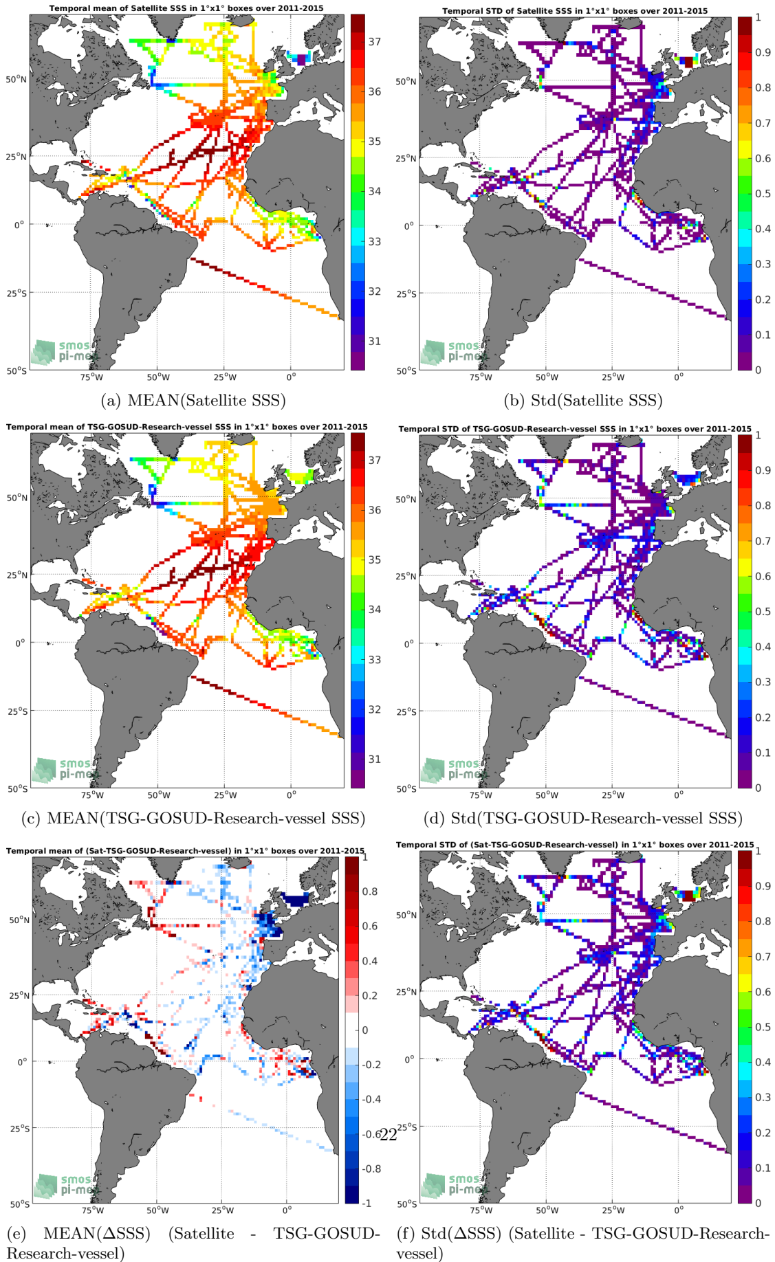
Figure 6: Temporal mean (left) and Std (right) of SSS from Aquarius-L3-OR-V5-MONTHLY-1DEG (top), TSG-GOSUD-Research-vessel (middle), and of \Delta SSS (Satellite - TSG-GOSUD-Research-vessel). Only match-up pairs are used to generate these maps.
