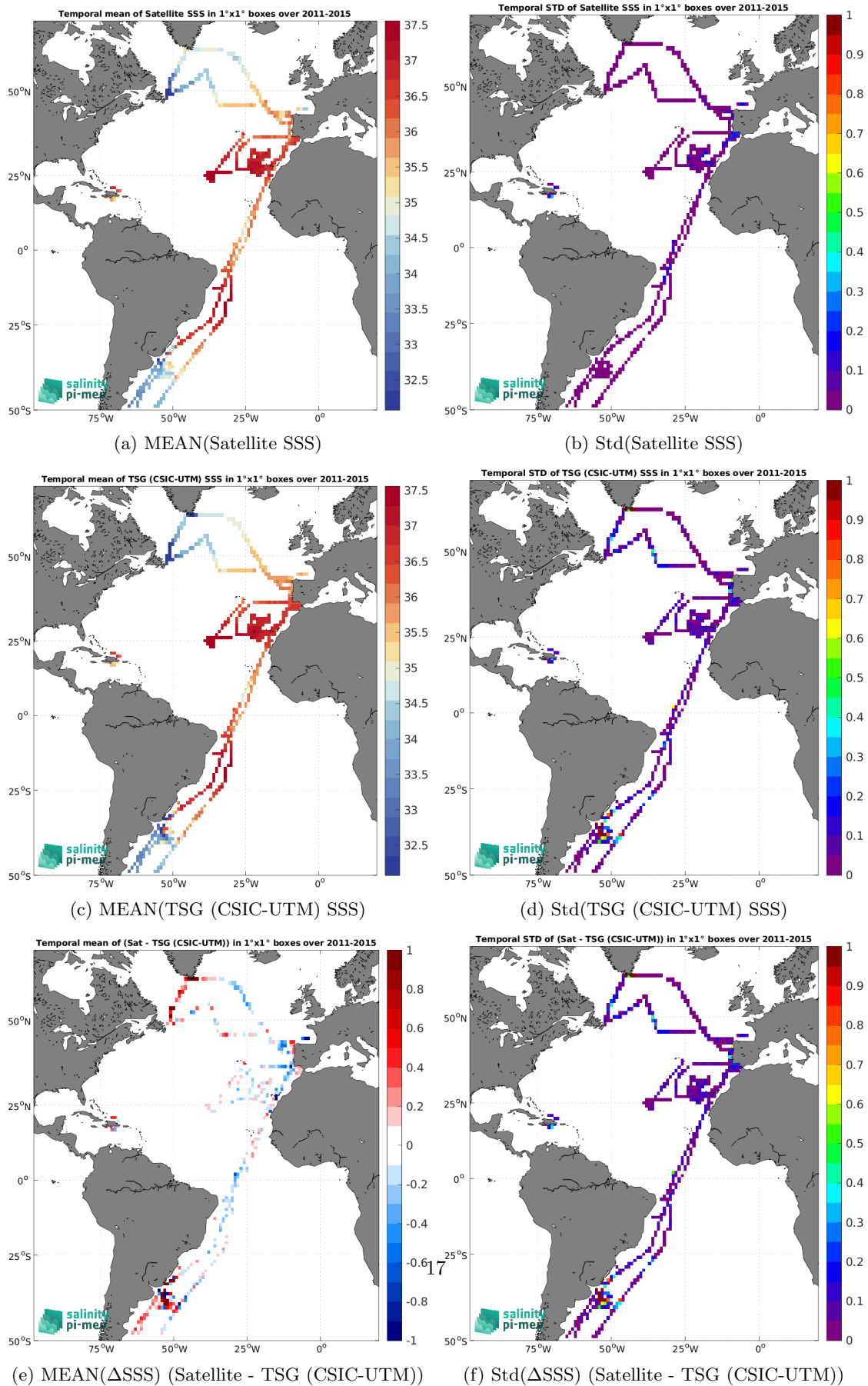
Figure 7: Temporal mean (left) and Std (right) of SSS from Aquarius SSS L3 OR v5 - Monthly (NASA-GSFC) (top), TSG (CSIC-UTM) (middle), and of \Delta SSS (Satellite - TSG (CSIC-UTM)). Only match-up pairs are used to generate these maps.
