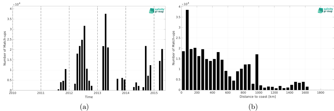
Figure 2: Number of match-ups between TSG (CSIC-UTM) and Aquarius SSS L3 OR v5 - Monthly (NASA-GSFC) SSS as a function of time (a) and as function of the distance to coast (b) over the Atlantic Ocean Pi-MEP region and for the full satellite product period.
