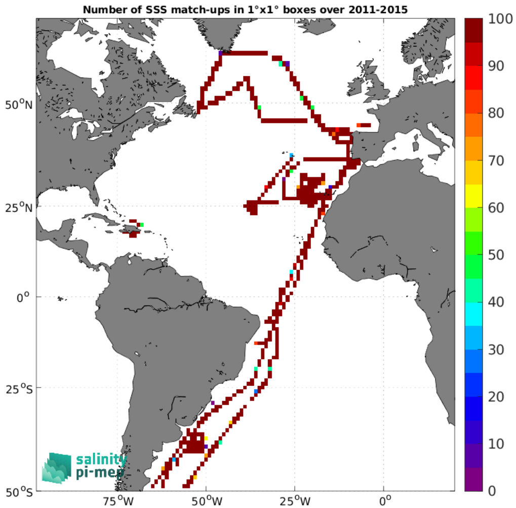
Figure 5: Number of SSS match-ups between TSG (CSIC-UTM) SSS and the Aquarius SSS L3 OR v5 - Monthly (NASA-GSFC) SSS product for the Atlantic Ocean Pi-MEP region over 1°x1° boxes and for the full satellite product period.
