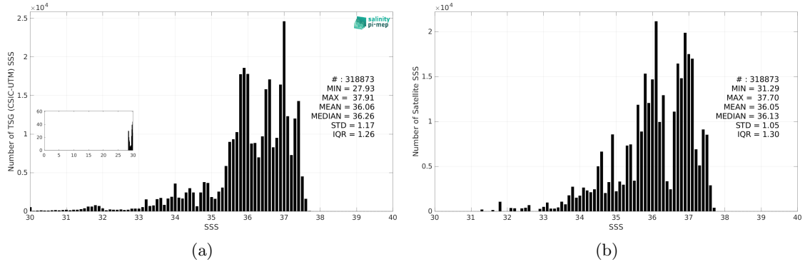
Figure 3: Histograms of SSS from TSG (CSIC-UTM) (a) and Aquarius SSS L3 OR v5 - Monthly (NASA-GSFC) (b) considering all match-up pairs per bins of 0.1 over the Atlantic Ocean Pi-MEP region and for the full satellite product period.
