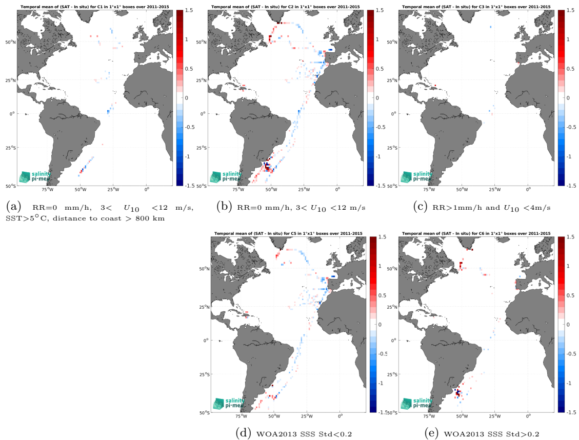
Figure 14: Temporal mean gridded over spatial boxes of size 1^\circ \times 1^\circ of \Delta SSS (Aquarius SSS L3 OR v5 - Monthly (NASA-GSFC) - TSG (CSIC-UTM)) for 5 different subdatasets corresponding to:RR=0 mm/h, 3 < U_{10} < 12 m/s, SST>5°C, distance to coast > 800 km (a), RR=0 mm/h, 3 < U_{10} < 12 m/s (b), RR>1mm/h and U_{10} < 4 m/s (c), WOA2013 SSS Std<0.2 (d), WOA2013 SSS Std>0.2 (e).
