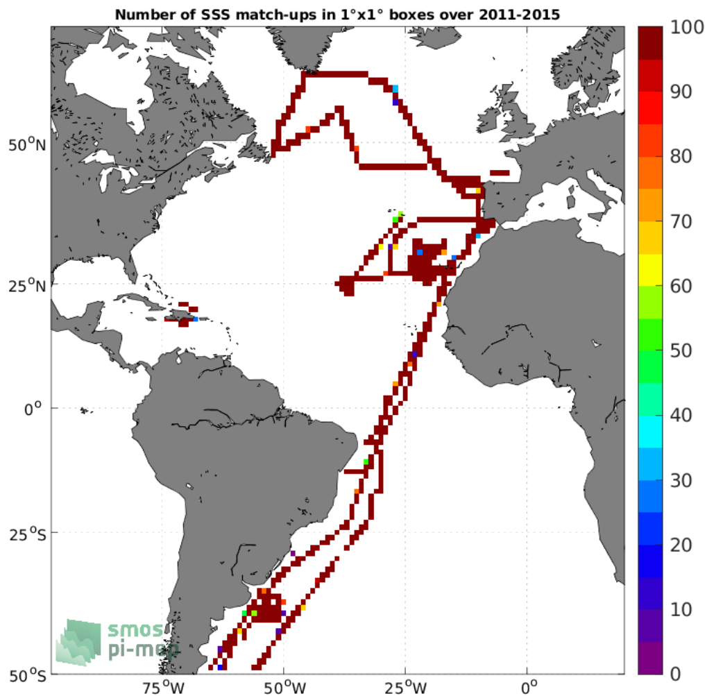
Figure 4: Number of SSS match-ups between TSG (CSIC-UTM) SSS and the Aquarius SSS L3 OR v5 - Monthly (NASA-GSFC) SSS product for the Atlantic Ocean Pi-MEP region over 1°x1° boxes and for the full satellite product period.
