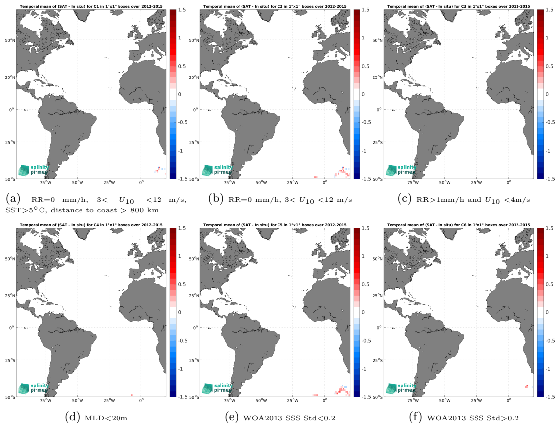
Figure 12: Temporal mean gridded over spatial boxes of size 1^\circ \times 1^\circ of \Delta\text{SSS} (Aquarius SSS L3 OR v5 - Monthly (NASA-GSFC) - Marine mammals) for 6 different subdatasets corresponding to: RR=0 mm/h, 3 < U_{10} < 12 m/s, SST > 5^\circ\text{C} , distance to coast > 800 km (a), RR=0 mm/h, 3 < U_{10} < 12 m/s (b), RR > 1 mm/h and U_{10} < 4 m/s (c), MLD < 20 m (d), WOA2013 SSS Std < 0.2 (e), WOA2013 SSS Std > 0.2 (f).
