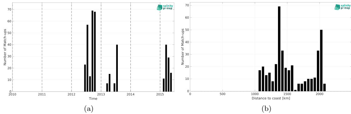
Figure 1: Number of match-ups between Marine mammals and Aquarius SSS L3 OR v5 - Monthly (NASA-GSFC) SSS as a function of time (a) and as function of the distance to coast (b) over the Atlantic Ocean Pi-MEP region and for the full satellite product period.
