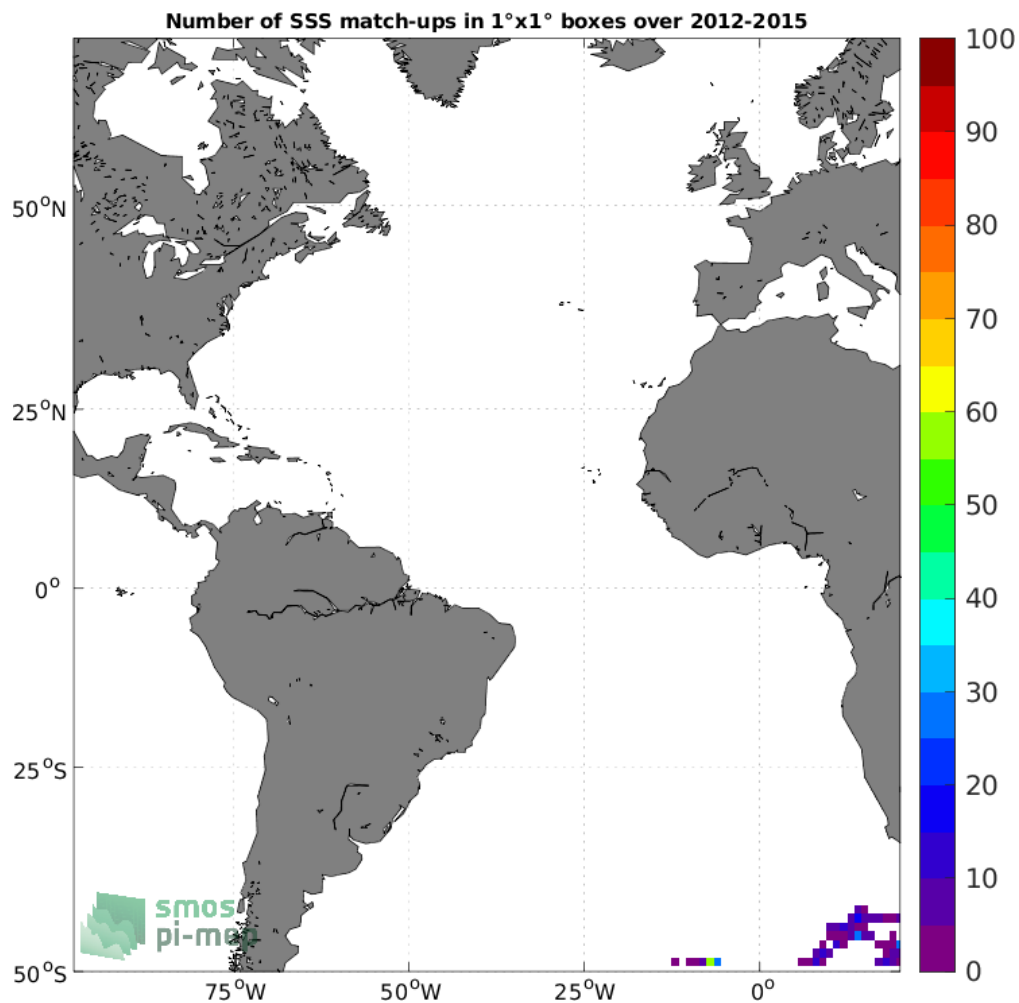
Figure 4: Number of SSS match-ups between Marine mammals SSS and the Aquarius SSS L3 OR v5 - Monthly (NASA-GSFC) SSS product for the Atlantic Ocean Pi-MEP region over 1°x1° boxes and for the full satellite product period.
