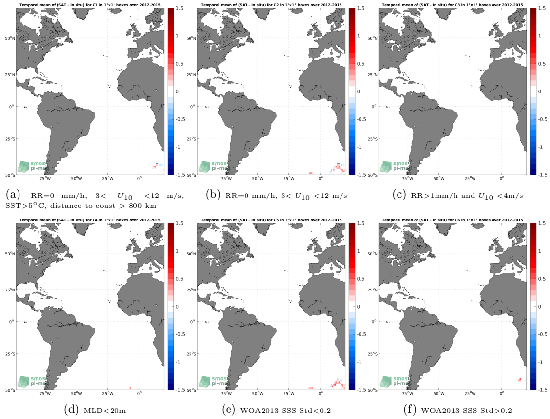
Figure 12: Temporal mean gridded over spatial boxes of size 1^\circ \times 1^\circ of \Delta SSS (Aquarius SSS L3 OR v5 - Monthly (NASA-GSFC) - Marine mammals) for 6 different subdatasets corresponding to: RR=0 mm/h, 3 < U_{10} < 12 m/s, SST > 5°C, distance to coast > 800 km (a), RR=0 mm/h, 3 < U_{10} < 12 m/s (b), RR > 1mm/h and U_{10} < 4 m/s (c), MLD < 20m (d), WOA2013 SSS Std < 0.2 (e), WOA2013 SSS Std > 0.2 (f).
