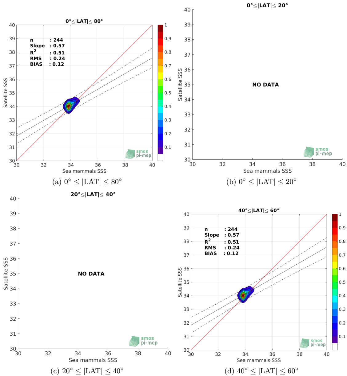
Figure 9: Contour maps of the concentration of Aquarius-L3-OR-V5-MONTHLY-1DEG SSS (y-axis) versus Sea mammals SSS (x-axis) at match-up pairs for different latitude bands. For each plot, the red line shows x=y . The black thin and dashed lines indicate a linear fit through the data cloud and the \pm 95\% confidence levels, respectively. The number match-up pairs n , the slope and R^2 coefficient of the linear fit, the root mean square (RMS) and the mean bias between satellite and in situ data are indicated for each latitude band in each plots.
