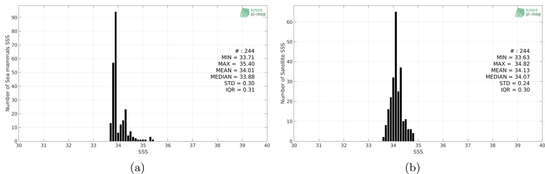
Figure 2: Histograms of SSS from Sea mammals (a) and Aquarius-L3-OR-V5-MONTHLY-1DEG (b) considering all match-up pairs per bins of 0.1 over the Atlantic Ocean Pi-MEP region and for the full satellite product period.
