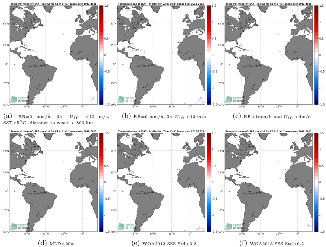
Figure 12: Temporal mean gridded over spatial boxes of size 1^\circ \times 1^\circ of \Delta SSS (Aquarius-L3-OR-V5-MONTHLY-1DEG - Sea mammals) for 6 different subdatasets corresponding to:RR=0 mm/h, 3 < U_{10} < 12 m/s, SST >5^\circ C, distance to coast > 800 km (a), RR=0 mm/h, 3 < U_{10} < 12 m/s (b), RR >1 mm/h and U_{10} < 4 m/s (c),MLD <20 m (d),WOA2013 SSS Std <0.2 (e),WOA2013 SSS Std >0.2 (f).
