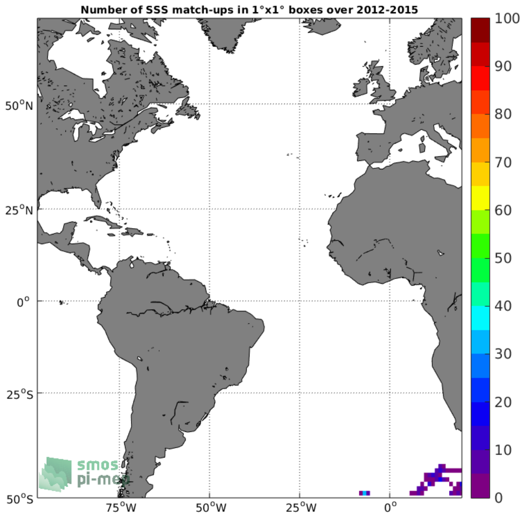
Figure 4: Number of SSS match-ups between Sea mammals SSS and the Aquarius-L3-OR-V5-MONTHLY-1DEG SSS product for the Atlantic Ocean Pi-MEP region over 1°x1° boxes and for the full satellite product period.
