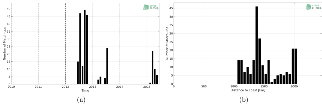
Figure 1: Number of match-ups between Sea mammals and Aquarius-L3-OR-V5-MONTHLY-1DEG SSS as a function of time (a) and as function of the distance to coast (b) over the Atlantic Ocean Pi-MEP region and for the full satellite product period.
