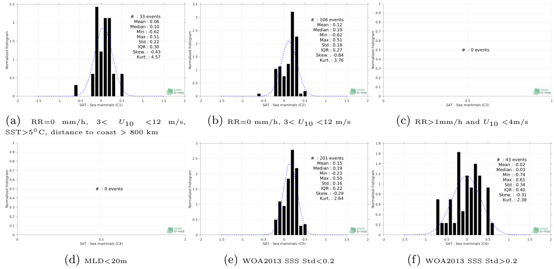
Figure 13: Normalized histogram of \Delta SSS (Aquarius-L3-OR-V5-MONTHLY-1DEG - Sea mammals) for 6 different subdatasets corresponding to: RR=0 mm/h, 3 < U_{10} < 12 m/s, SST>5°C, distance to coast > 800 km (a), RR=0 mm/h, 3 < U_{10} < 12 m/s (b), RR>1mm/h and U_{10} < 4 m/s (c), MLD<20m (d), WOA2013 SSS Std<0.2 (e), WOA2013 SSS Std>0.2 (f).
