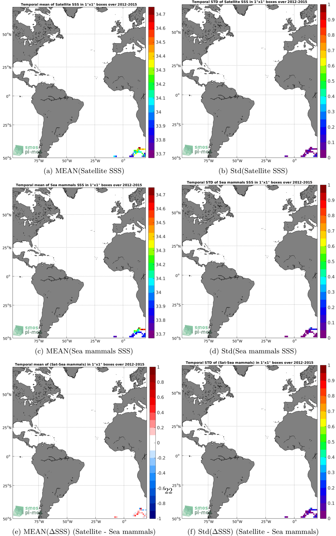
Figure 6: Temporal mean (left) and Std (right) of SSS from Aquarius-L3-OR-V5-MONTHLY-1DEG (top), Sea mammals (middle), and of \Delta SSS (Satellite - Sea mammals). Only match-up pairs are used to generate these maps.
