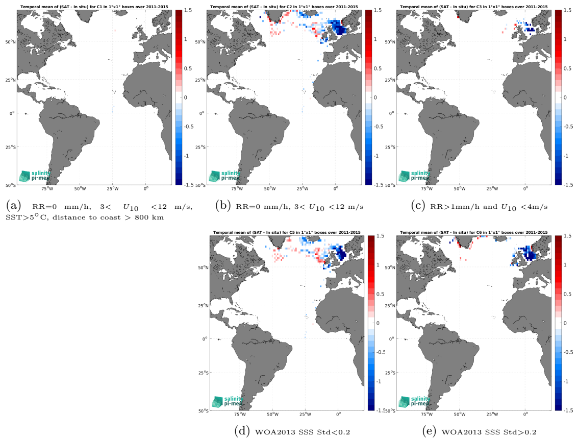
Figure 14: Temporal mean gridded over spatial boxes of size 1^\circ \times 1^\circ of \Delta\text{SSS} (Aquarius SSS L3 OR v5 - Monthly (NASA-GSFC) - ICES) for 5 different subdatasets corresponding to:RR=0 mm/h, 3 < U_{10} < 12 m/s, SST>5°C, distance to coast > 800 km (a), RR=0 mm/h, 3 < U_{10} < 12 m/s (b), RR>1mm/h and U_{10} < 4 m/s (c), WOA2013 SSS Std<0.2 (d), WOA2013 SSS Std>0.2 (e).
