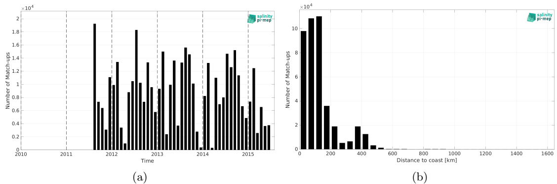
Figure 2: Number of match-ups between ICES and Aquarius SSS L3 OR v5 - Monthly (NASA-GSFC) SSS as a function of time (a) and as function of the distance to coast (b) over the Atlantic Ocean Pi-MEP region and for the full satellite product period.
