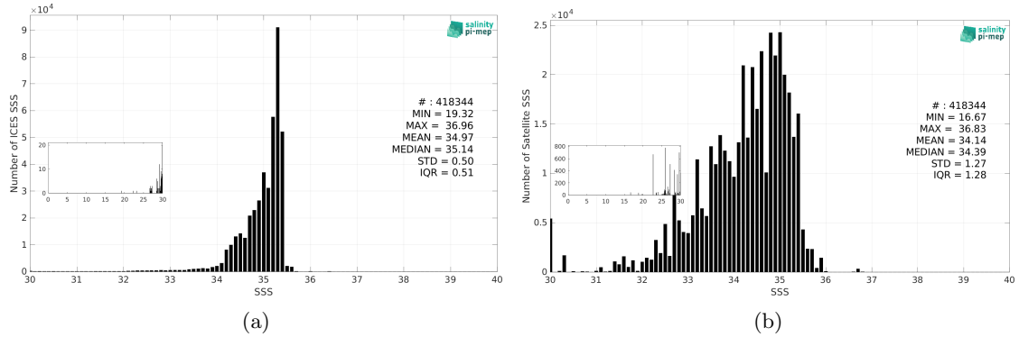
Figure 3: Histograms of SSS from ICES (a) and Aquarius SSS L3 OR v5 - Monthly (NASA-GSFC) (b) considering all match-up pairs per bins of 0.1 over the Atlantic Ocean Pi-MEP region and for the full satellite product period.
