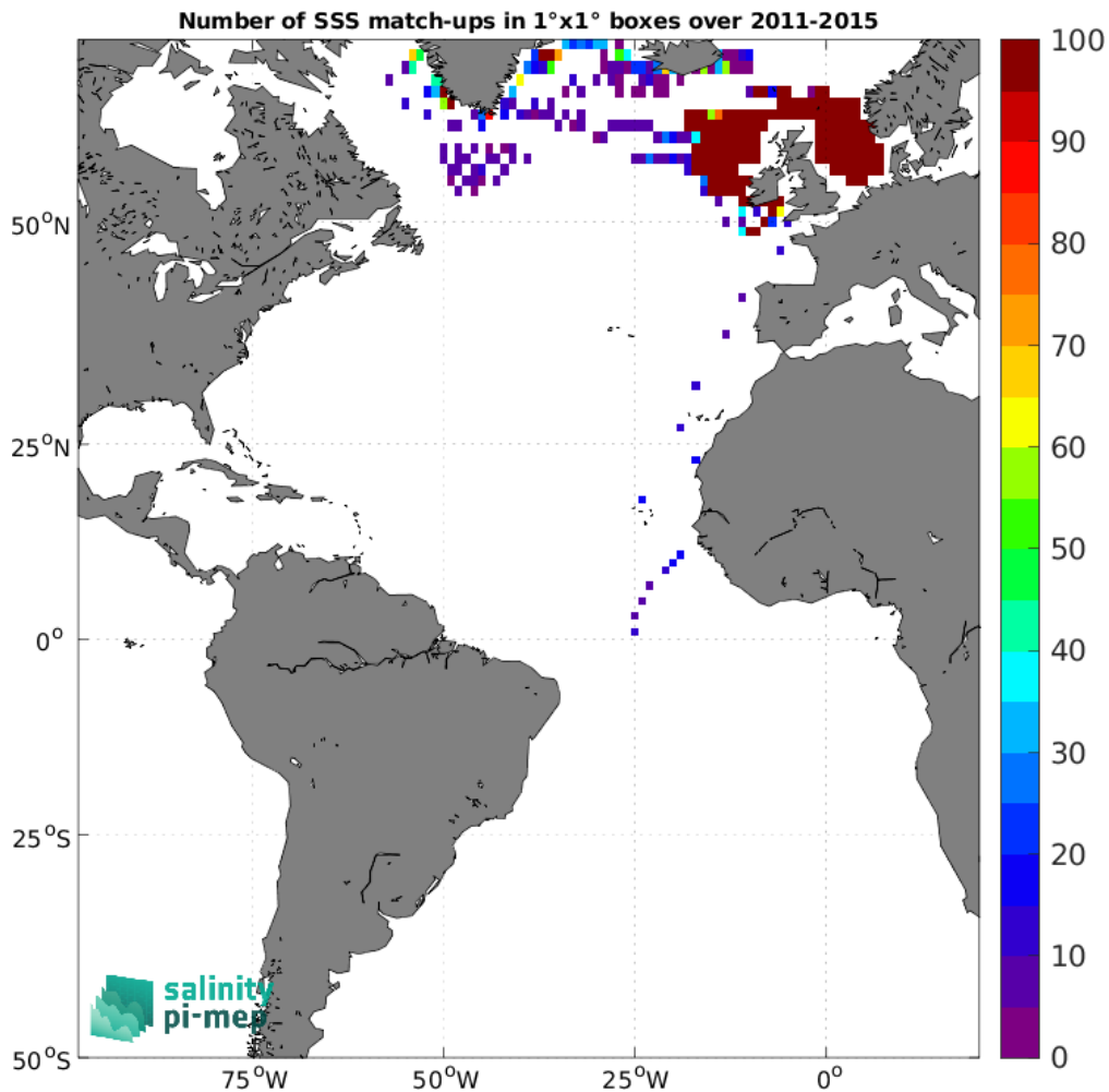
Figure 5: Number of SSS match-ups between ICES SSS and the Aquarius SSS L3 OR v5 - Monthly (NASA-GSFC) SSS product for the Atlantic Ocean Pi-MEP region over 1^{\circ} \times 1^{\circ} boxes and for the full satellite product period.
