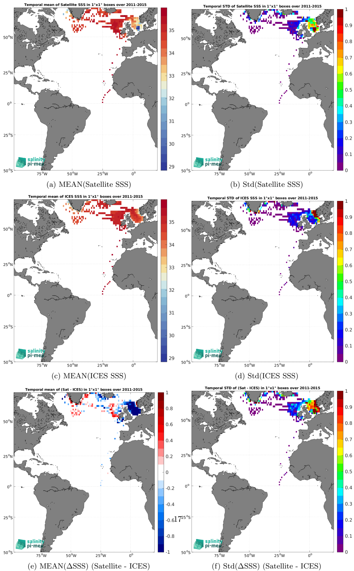
Figure 7: Temporal mean (left) and Std (right) of SSS from Aquarius SSS L3 OR v5 - Monthly (NASA-GSFC) (top), ICES (middle), and of \Delta SSS (Satellite - ICES). Only match-up pairs are used to generate these maps.
