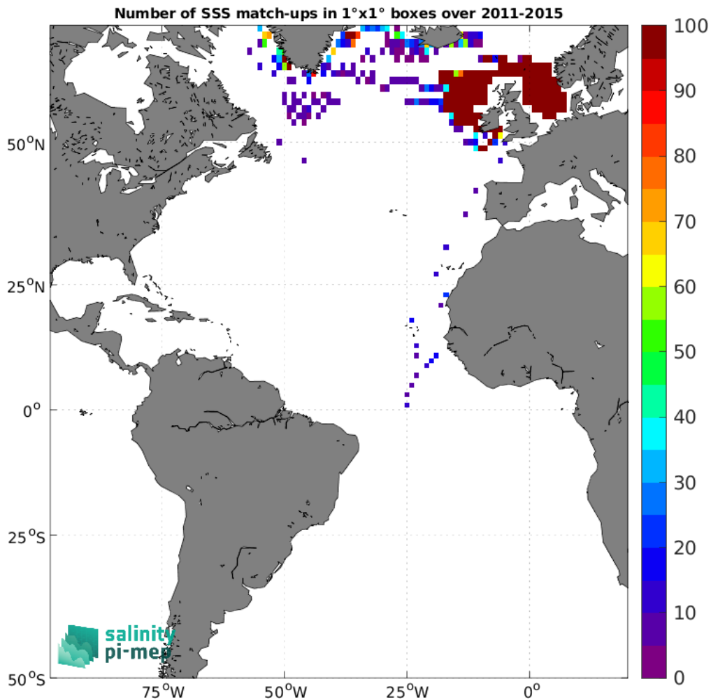
Figure 4: Number of SSS match-ups between ICES SSS and the Aquarius SSS L3 OR v5 - Monthly (NASA-GSFC) SSS product for the Atlantic Ocean Pi-MEP region over 1^\circ \times 1^\circ boxes and for the full satellite product period.
