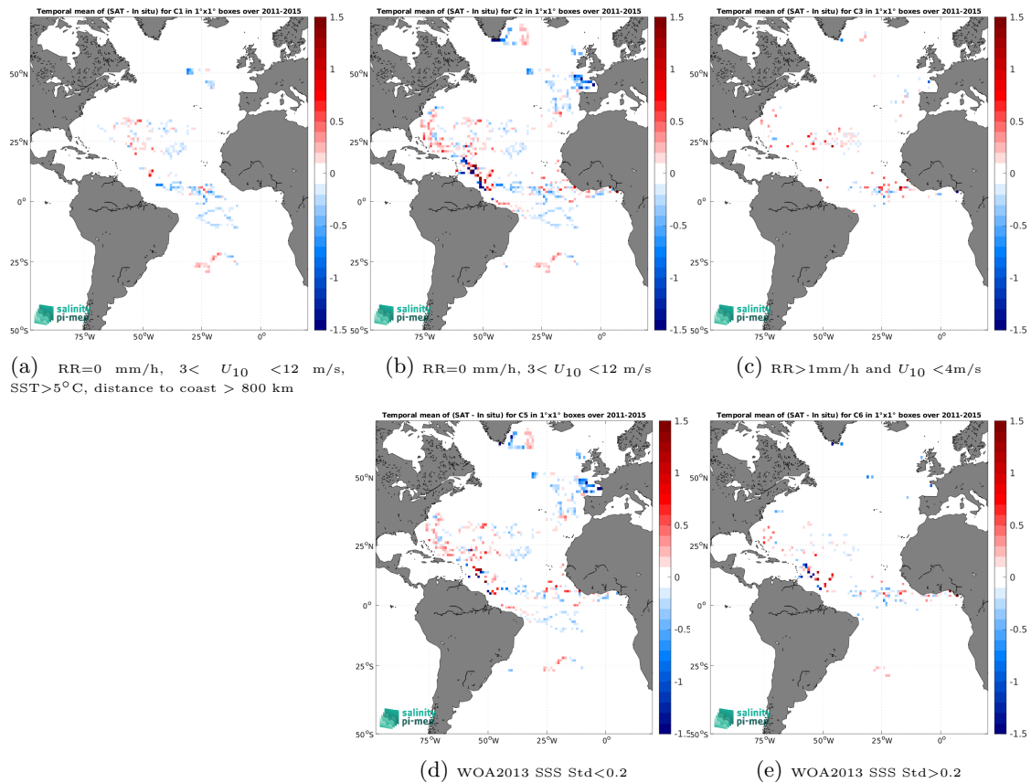
Figure 13: Temporal mean gridded over spatial boxes of size 1^\circ \times 1^\circ of \Delta SSS (Aquarius SSS L3 OR v5 - Monthly (NASA-GSFC) - Surface drifters) for 5 different subdatasets corresponding to:RR=0 mm/h, 3 < U_{10} < 12 m/s, SST >5^\circ\text{C} , distance to coast > 800 km (a), RR=0 mm/h, 3 < U_{10} < 12 m/s (b), RR >1 mm/h and U_{10} < 4 m/s (c), WOA2013 SSS Std <0.2 (d), WOA2013 SSS Std >0.2 (e).
