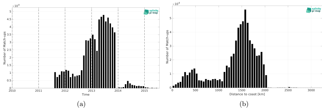
Figure 2: Number of match-ups between Surface drifters and Aquarius SSS L3 OR v5 - Monthly (NASA-GSFC) SSS as a function of time (a) and as function of the distance to coast (b) over the Atlantic Ocean Pi-MEP region and for the full satellite product period.
