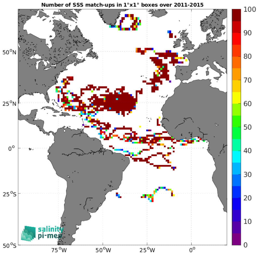
Figure 4: Number of SSS match-ups between Surface drifters SSS and the Aquarius SSS L3 OR v5 - Monthly (NASA-GSFC) SSS product for the Atlantic Ocean Pi-MEP region over 1^{\circ} \times 1^{\circ} boxes and for the full satellite product period.
