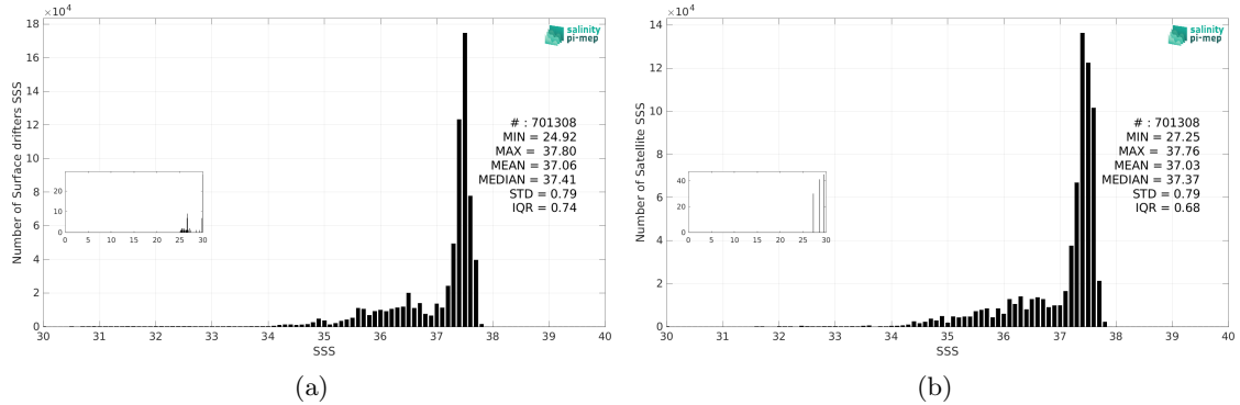
Figure 3: Histograms of SSS from Surface drifters (a) and Aquarius SSS L3 OR v5 - Monthly (NASA-GSFC) (b) considering all match-up pairs per bins of 0.1 over the Atlantic Ocean Pi-MEP region and for the full satellite product period.
