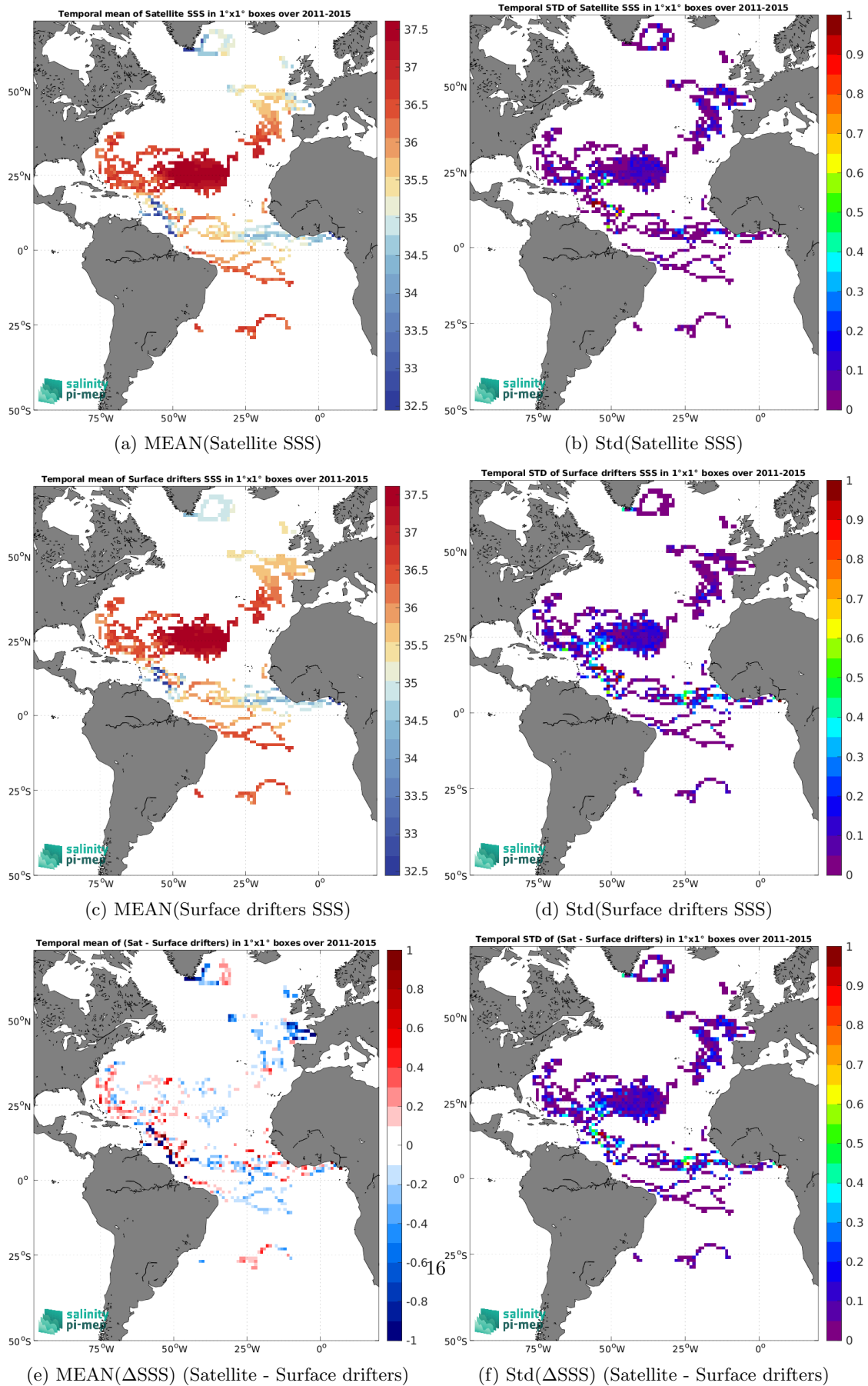
Figure 6: Temporal mean (left) and Std (right) of SSS from Aquarius SSS L3 OR v5 - Monthly (NASA-GSFC) (top), Surface drifters (middle), and of \Delta SSS (Satellite - Surface drifters). Only match-up pairs are used to generate these maps.
