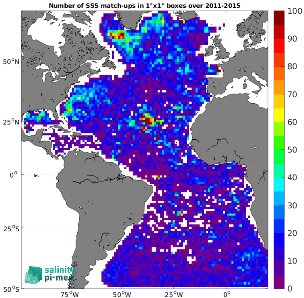
Figure 4: Number of SSS match-ups between Argo SSS and the Aquarius SSS L3 OR v5 - Monthly (NASA-GSFC) SSS product for the Atlantic Ocean Pi-MEP region over 1^{\circ} \times 1^{\circ} boxes and for the full satellite product period.
