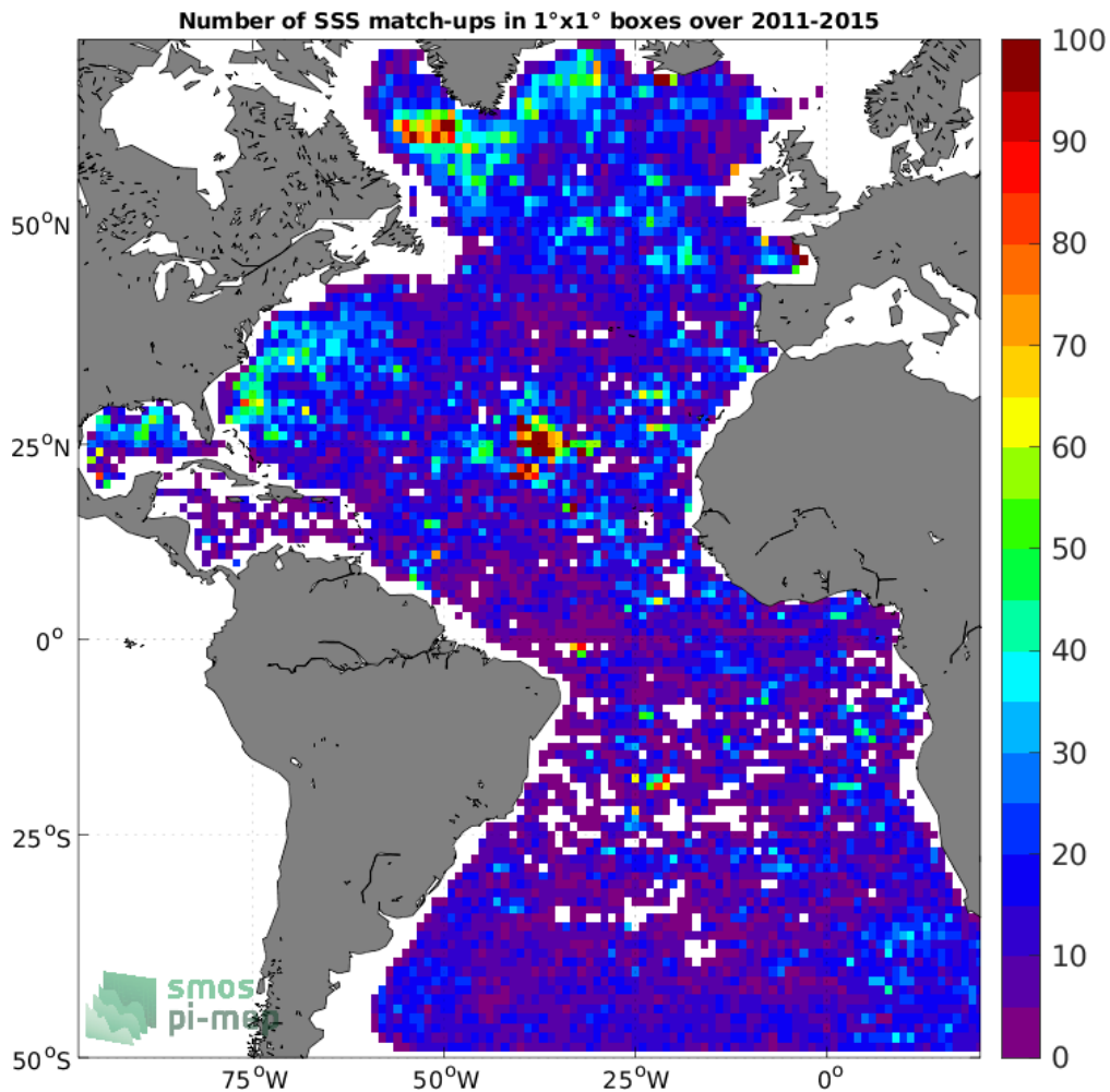
Figure 4: Number of SSS match-ups between Argo SSS and the Aquarius SSS L3 OR v5 - Monthly (NASA-GSFC) SSS product for the Atlantic Ocean Pi-MEP region over 1°×1° boxes and for the full satellite product period.
