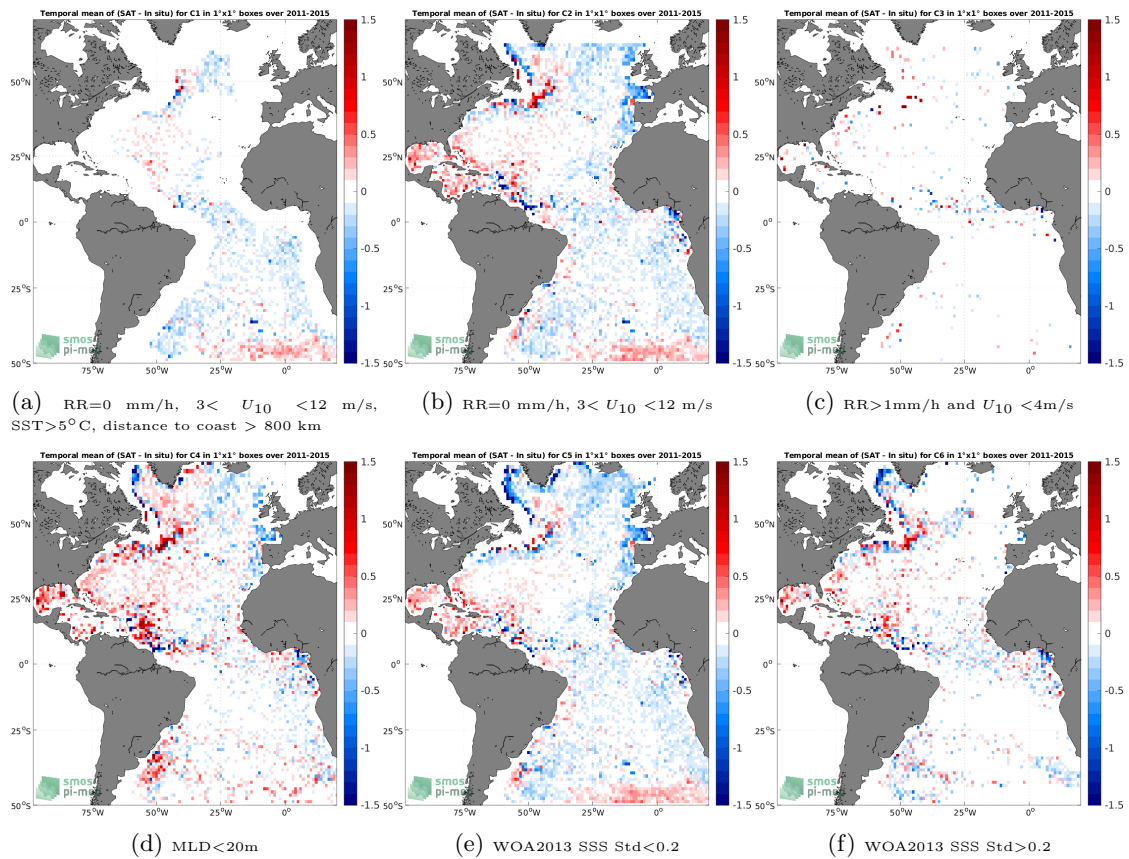
Figure 12: Temporal mean gridded over spatial boxes of size 1^\circ \times 1^\circ of \Delta SSS (Aquarius SSS L3 OR v5 - Monthly (NASA-GSFC) - Argo) for 6 different subdatasets corresponding to:RR=0 mm/h, 3 < U_{10} < 12 m/s, SST >5^\circ C, distance to coast > 800 km (a), RR=0 mm/h, 3 < U_{10} < 12 m/s (b), RR >1 mm/h and U_{10} < 4 m/s (c),MLD <20 m (d),WOA2013 SSS Std <0.2 (e),WOA2013 SSS Std >0.2 (f).
