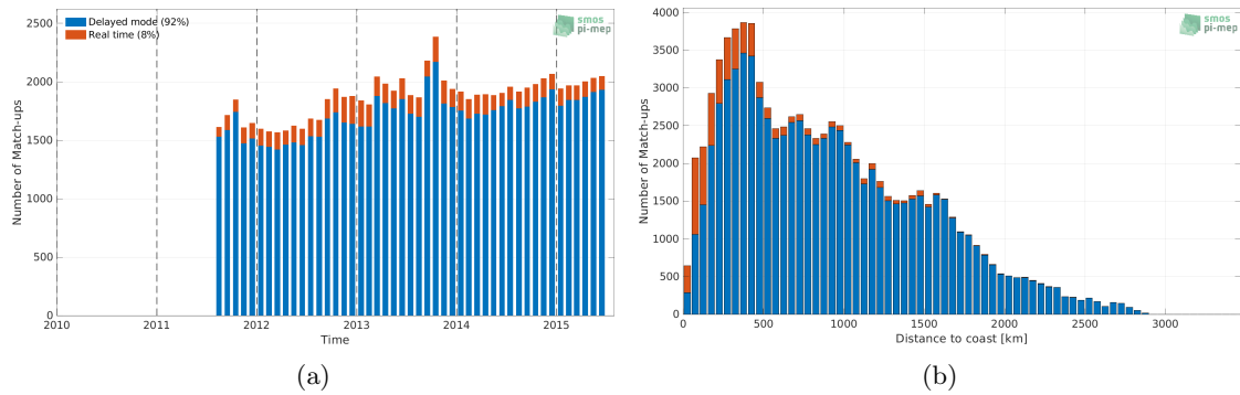
Figure 1: Number of match-ups between Argo and Aquarius SSS L3 OR v5 - Monthly (NASA-GSFC) SSS as a function of time (a) and as function of the distance to coast (b) over the Atlantic Ocean Pi-MEP region and for the full satellite product period.
