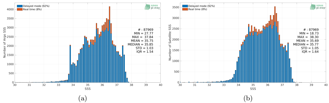
Figure 2: Histograms of SSS from Argo (a) and Aquarius SSS L3 OR v5 - Monthly (NASA-GSFC) (b) considering all match-up pairs per bins of 0.1 over the Atlantic Ocean Pi-MEP region and for the full satellite product period.
