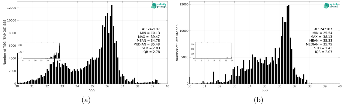
Figure 3: Histograms of SSS from TSG (SAMOS) (a) and Aquarius SSS L3 OR v5 - Monthly - Rain mask (NASA-GSFC) (b) considering all match-up pairs per bins of 0.1 over the Atlantic Ocean Pi-MEP region and for the full satellite product period.
