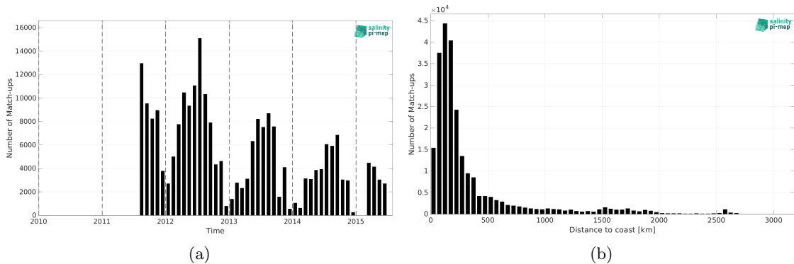
Figure 2: Number of match-ups between TSG (SAMOS) and Aquarius SSS L3 OR v5 - Monthly - Rain mask (NASA-GSFC) SSS as a function of time (a) and as function of the distance to coast (b) over the Atlantic Ocean Pi-MEP region and for the full satellite product period.
