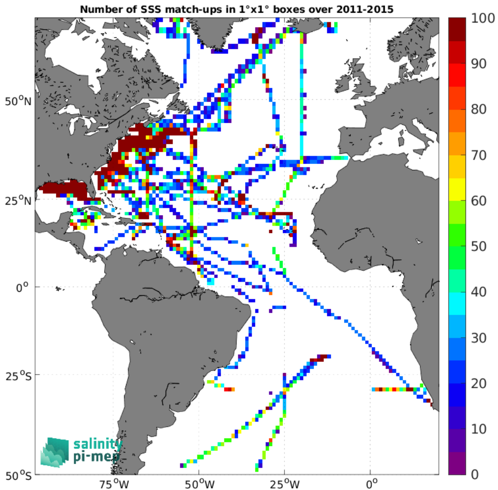
Figure 5: Number of SSS match-ups between TSG (SAMOS) SSS and the Aquarius SSS L3 OR v5 - Monthly - Rain mask (NASA-GSFC) SSS product for the Atlantic Ocean Pi-MEP region over 1^\circ \times 1^\circ boxes and for the full satellite product period.
