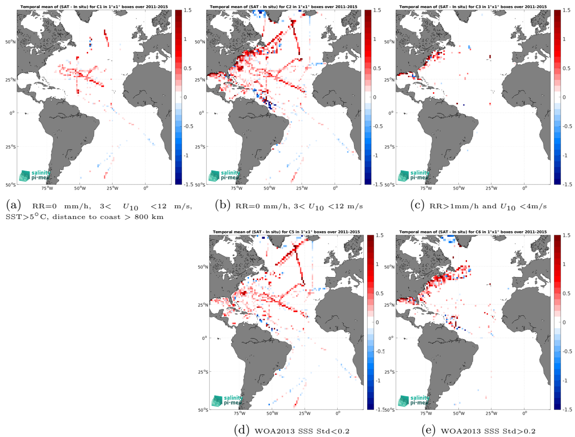
Figure 14: Temporal mean gridded over spatial boxes of size 1^\circ \times 1^\circ of \Delta\text{SSS} (Aquarius SSS L3 OR v5 - Monthly - Rain mask (NASA-GSFC) - TSG (SAMOS)) for 5 different subdatasets corresponding to:RR=0 mm/h, 3 < U_{10} < 12 m/s, SST >5^\circ\text{C} , distance to coast > 800 km (a), RR=0 mm/h, 3 < U_{10} < 12 m/s (b), RR >1 mm/h and U_{10} < 4 m/s (c), WOA2013 SSS Std <0.2 (d), WOA2013 SSS Std >0.2 (e).
