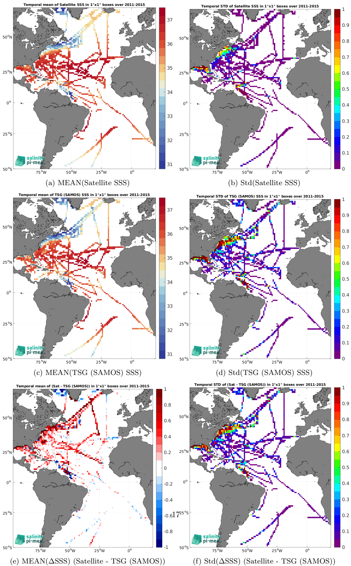
Figure 7: Temporal mean (left) and Std (right) of SSS from Aquarius SSS L3 OR v5 - Monthly - Rain mask (NASA-GSFC) (top), TSG (SAMOS) (middle), and of \Delta SSS (Satellite - TSG (SAMOS)). Only match-up pairs are used to generate these maps.
