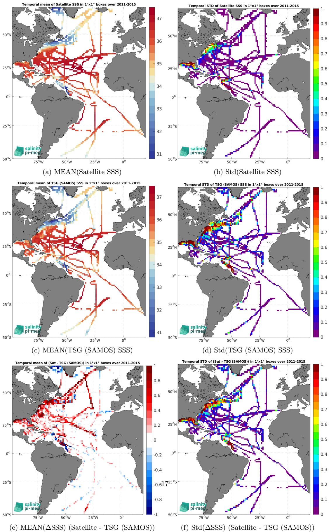
Figure 6: Temporal mean (left) and Std (right) of SSS from Aquarius SSS L3 OR v5 - Monthly - Rain mask (NASA-GSFC) (top), TSG (SAMOS) (middle), and of \Delta SSS (Satellite - TSG (SAMOS)). Only match-up pairs are used to generate these maps.
