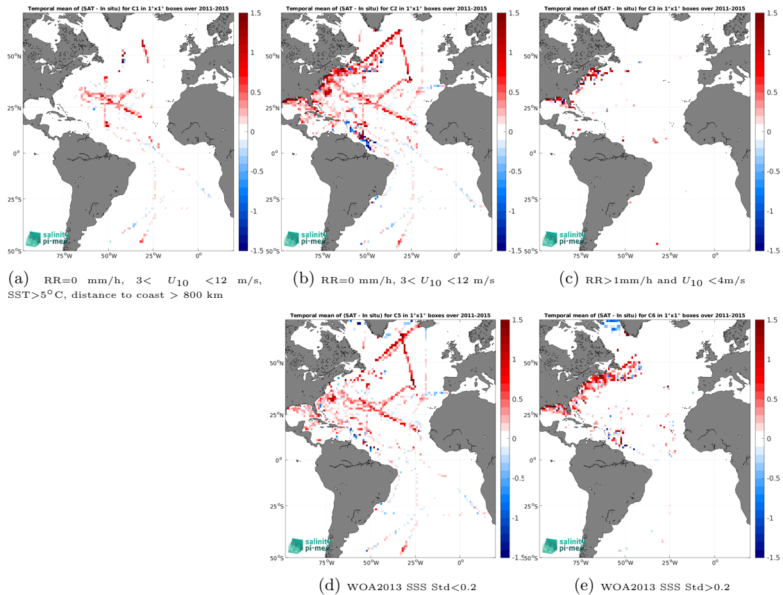
Figure 12: Temporal mean gridded over spatial boxes of size 1^\circ \times 1^\circ of \Delta SSS (Aquarius SSS L3 OR v5 - Monthly - Rain mask (NASA-GSFC) - TSG (SAMOS)) for 5 different subdatasets corresponding to:RR=0 mm/h, 3 < U_{10} < 12 m/s, SST >5^\circ\text{C} , distance to coast > 800 km (a), RR=0 mm/h, 3 < U_{10} < 12 m/s (b), RR >1 mm/h and U_{10} < 4 m/s (c), WOA2013 SSS Std <0.2 (d), WOA2013 SSS Std >0.2 (e).
