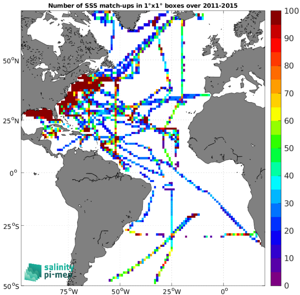
Figure 4: Number of SSS match-ups between TSG (SAMOS) SSS and the Aquarius SSS L3 OR v5 - Monthly - Rain mask (NASA-GSFC) SSS product for the Atlantic Ocean Pi-MEP region over 1^{\circ} \times 1^{\circ} boxes and for the full satellite product period.
