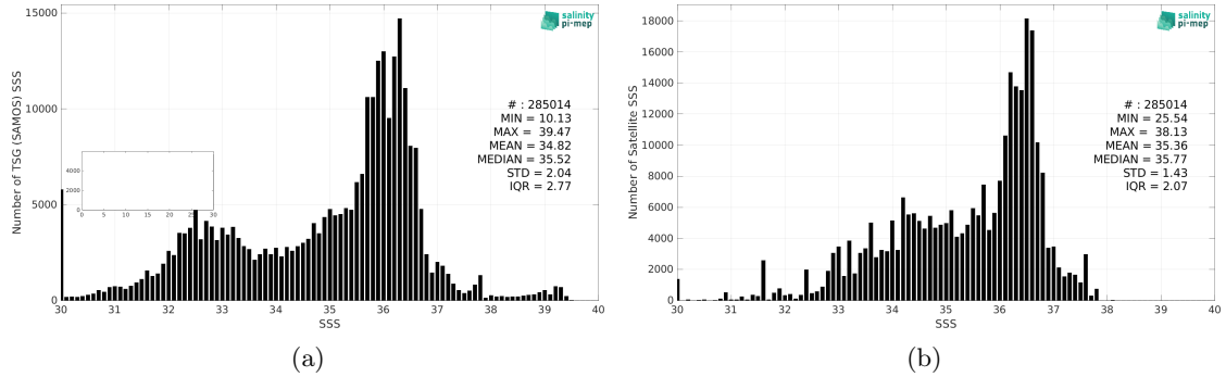
Figure 2: Histograms of SSS from TSG (SAMOS) (a) and Aquarius SSS L3 OR v5 - Monthly - Rain mask (NASA-GSFC) (b) considering all match-up pairs per bins of 0.1 over the Atlantic Ocean Pi-MEP region and for the full satellite product period.
