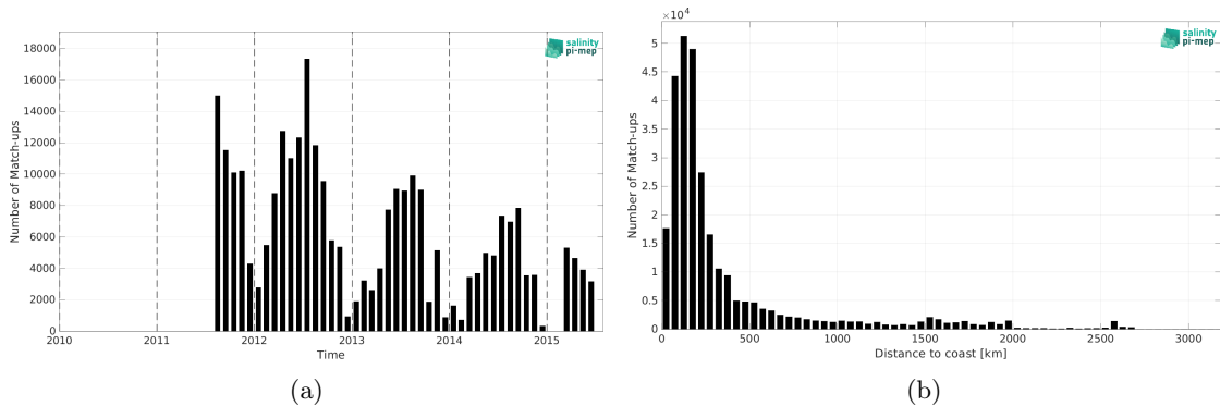
Figure 1: Number of match-ups between TSG (SAMOS) and Aquarius SSS L3 OR v5 - Monthly - Rain mask (NASA-GSFC) SSS as a function of time (a) and as function of the distance to coast (b) over the Atlantic Ocean Pi-MEP region and for the full satellite product period.
