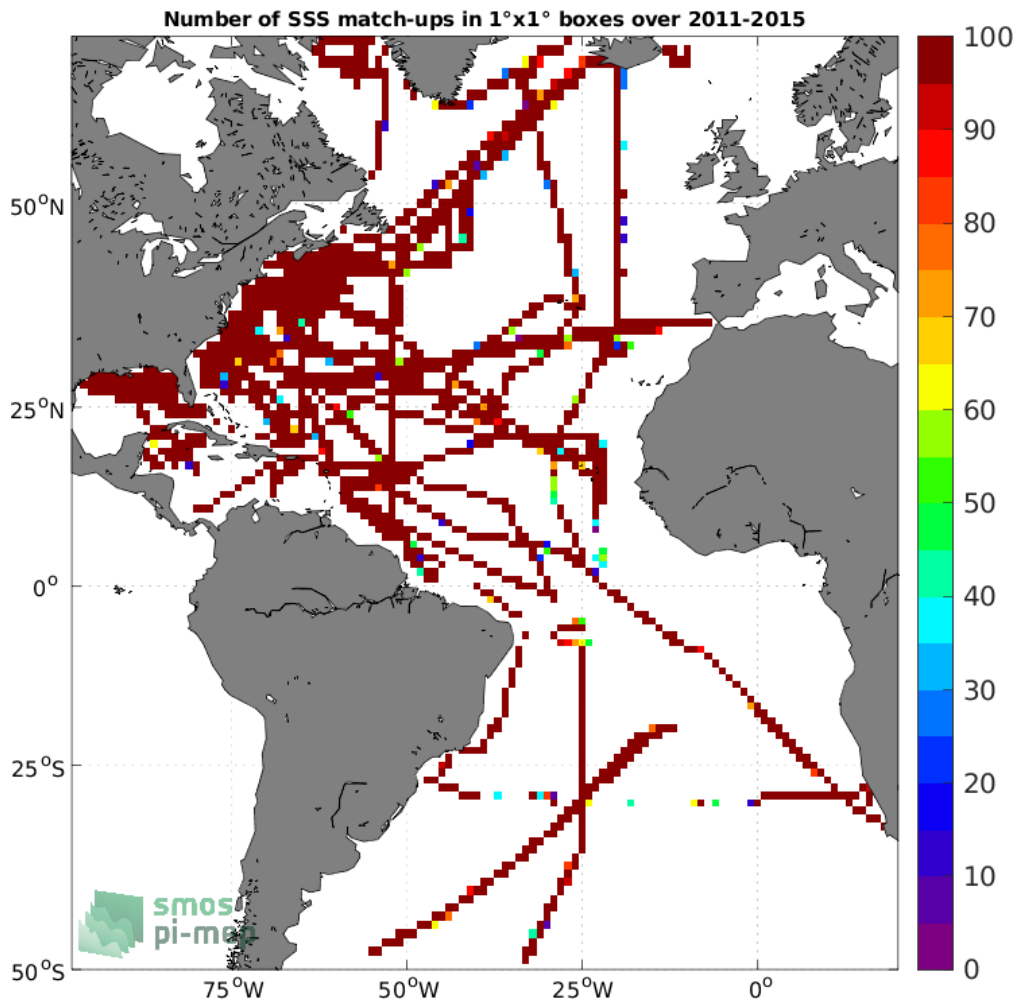
Figure 4: Number of SSS match-ups between TSG (SAMOS) SSS and the Aquarius SSS L3 OR v5 - Monthly - Rain mask (NASA-GSFC) SSS product for the Atlantic Ocean Pi-MEP region over 1°x1° boxes and for the full satellite product period.
