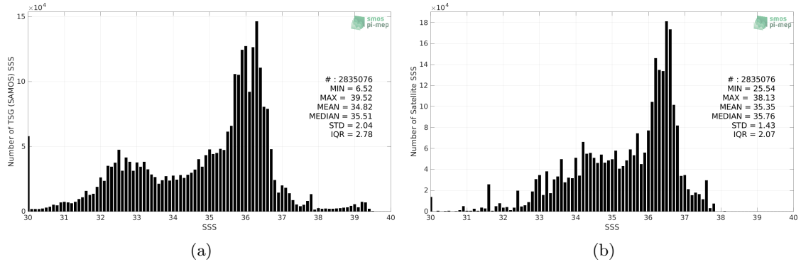
Figure 2: Histograms of SSS from TSG (SAMOS) (a) and Aquarius SSS L3 OR v5 - Monthly - Rain mask (NASA-GSFC) (b) considering all match-up pairs per bins of 0.1 over the Atlantic Ocean Pi-MEP region and for the full satellite product period.
