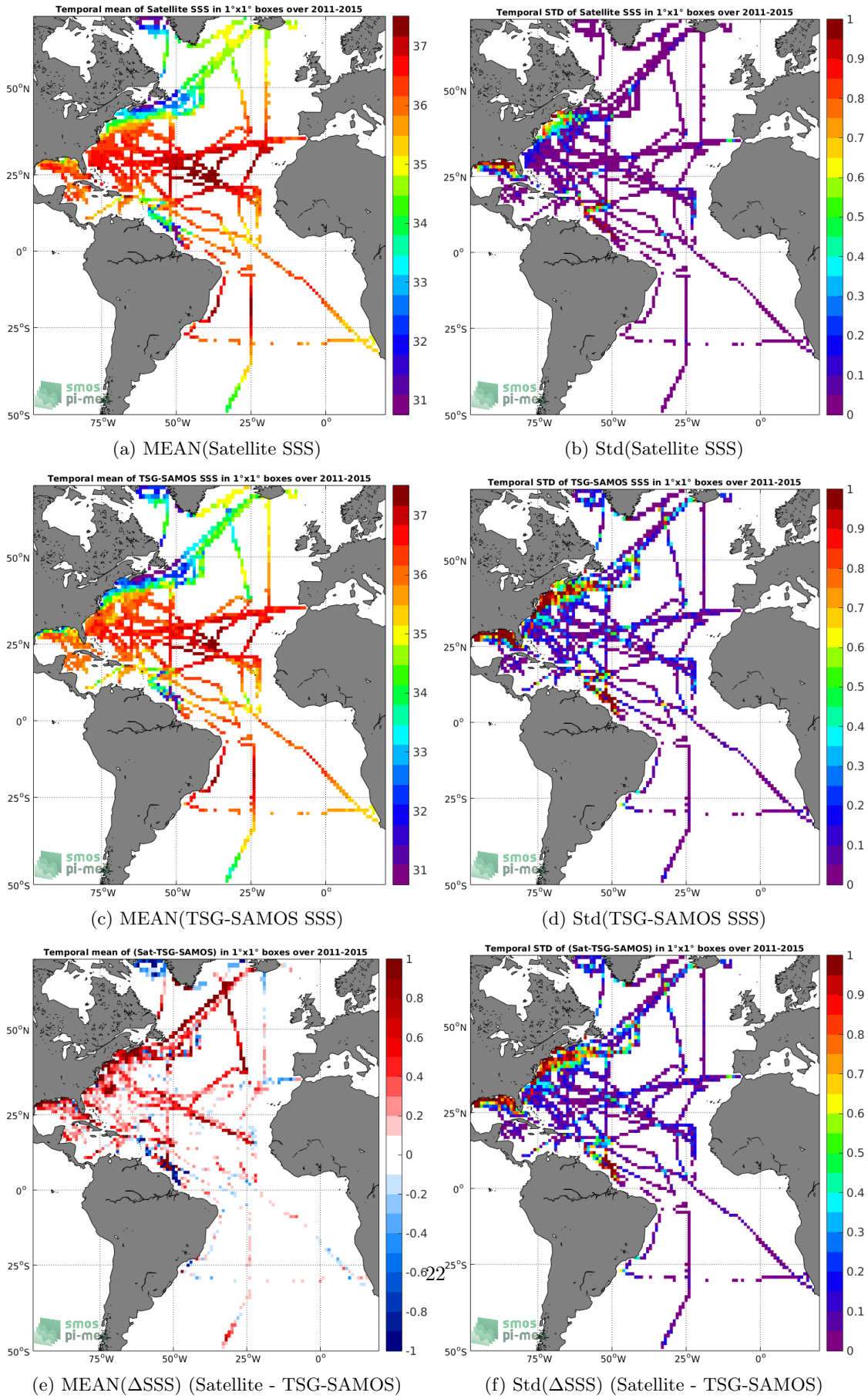
Figure 6: Temporal mean (left) and Std (right) of SSS from Aquarius-L3-OR-V5-MONTHLY-RAIN-MASK-IDEQ (top), TSG-SAMOS (middle), and of \Delta SSS (Satellite - TSG-SAMOS). Only match-up pairs are used to generate these maps.
