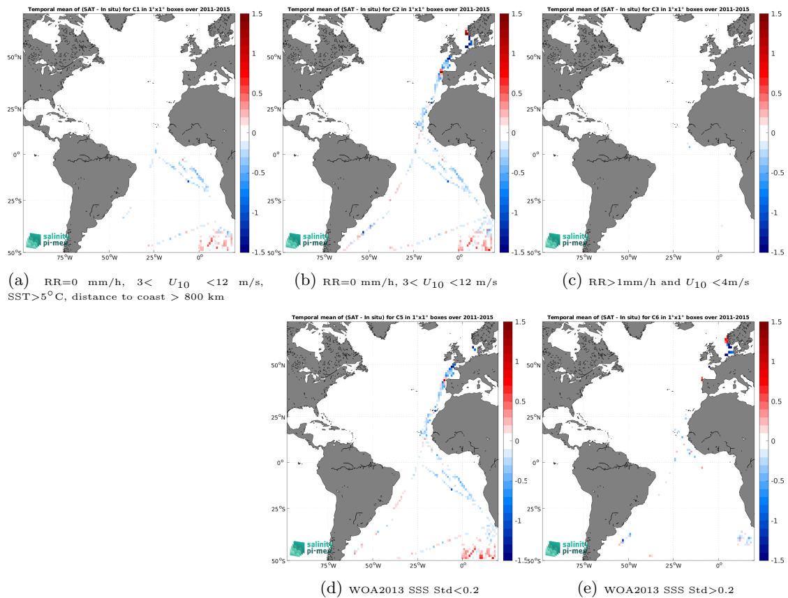
Figure 14: Temporal mean gridded over spatial boxes of size 1^\circ \times 1^\circ of \Delta\text{SSS} (Aquarius SSS L3 OR v5 - Monthly - Rain mask (NASA-GSFC) - TSG (Polarstern)) for 5 different subdatasets corresponding to:RR=0 mm/h, 3 < U_{10} < 12 m/s, SST >5^\circ\text{C} , distance to coast > 800 km (a), RR=0 mm/h, 3 < U_{10} < 12 m/s (b), RR >1 mm/h and U_{10} < 4 m/s (c), WOA2013 SSS Std <0.2 (d), WOA2013 SSS Std >0.2 (e).
