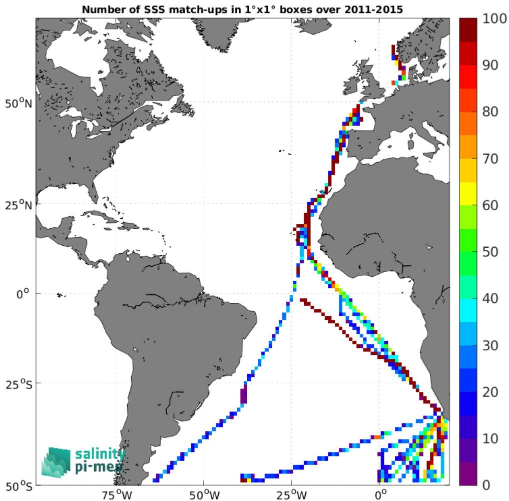
Figure 5: Number of SSS match-ups between TSG (Polarstern) SSS and the Aquarius SSS L3 OR v5 - Monthly - Rain mask (NASA-GSFC) SSS product for the Atlantic Ocean Pi-MEP region over 1°x1° boxes and for the full satellite product period.
