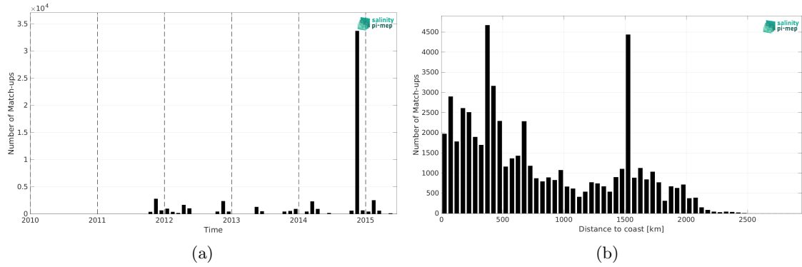
Figure 2: Number of match-ups between TSG (Polarstern) and Aquarius SSS L3 OR v5 - Monthly - Rain mask (NASA-GSFC) SSS as a function of time (a) and as function of the distance to coast (b) over the Atlantic Ocean Pi-MEP region and for the full satellite product period.
