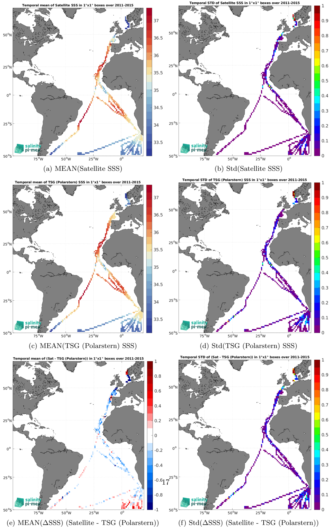
Figure 7: Temporal mean (left) and Std (right) of SSS from Aquarius SSS L3 OR v5 - Monthly - Rain mask (NASA-GSFC) (top), TSG (Polarstern) (middle), and of \Delta SSS (Satellite - TSG (Polarstern)). Only match-up pairs are used to generate these maps.
