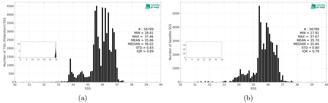
Figure 3: Histograms of SSS from TSG (Polarstern) (a) and Aquarius SSS L3 OR v5 - Monthly - Rain mask (NASA-GSFC) (b) considering all match-up pairs per bins of 0.1 over the Atlantic Ocean Pi-MEP region and for the full satellite product period.
