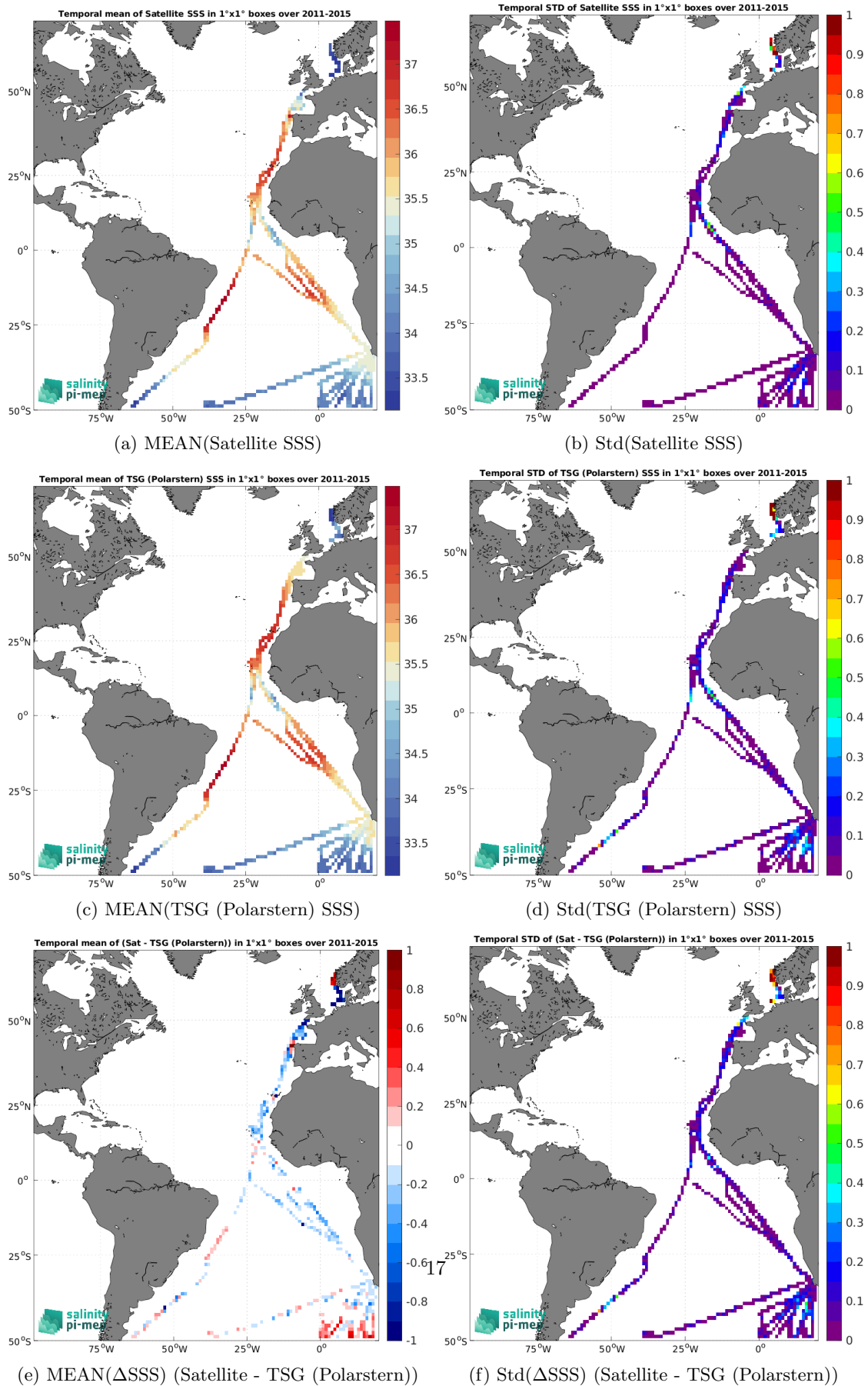
Figure 6: Temporal mean (left) and Std (right) of SSS from Aquarius SSS L3 OR v5 - Monthly - Rain mask (NASA-GSFC) (top), TSG (Polarstern) (middle), and of \Delta SSS (Satellite - TSG (Polarstern)). Only match-up pairs are used to generate these maps.
