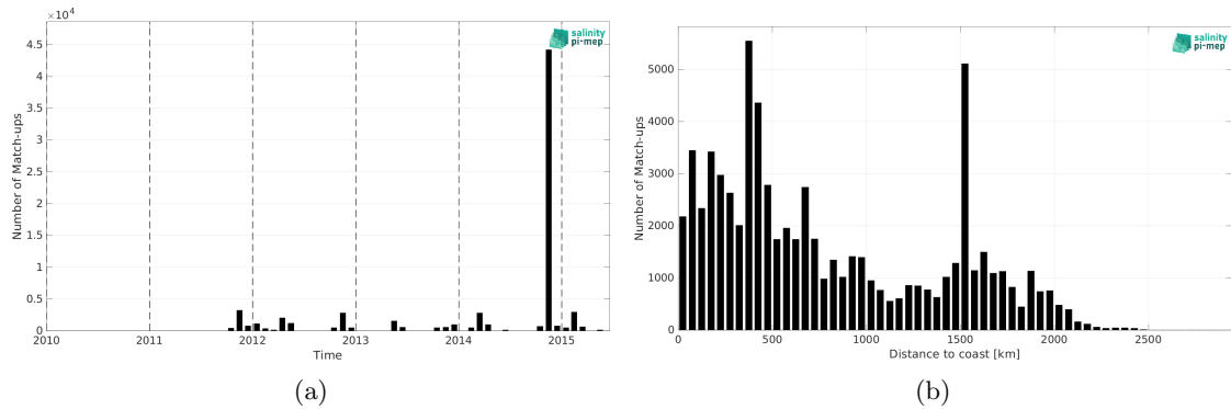
Figure 1: Number of match-ups between TSG (Polarstern) and Aquarius SSS L3 OR v5 - Monthly - Rain mask (NASA-GSFC) SSS as a function of time (a) and as function of the distance to coast (b) over the Atlantic Ocean Pi-MEP region and for the full satellite product period.
