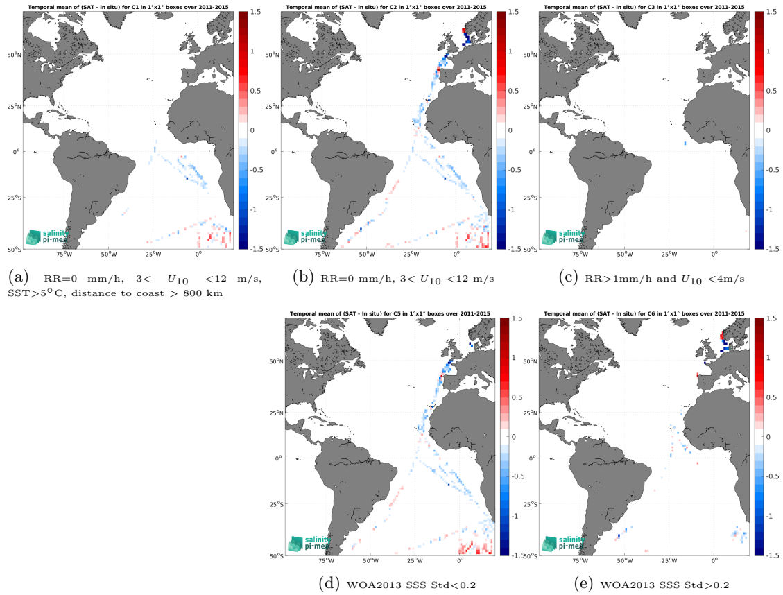
Figure 12: Temporal mean gridded over spatial boxes of size 1^\circ \times 1^\circ of \Delta SSS (Aquarius SSS L3 OR v5 - Monthly - Rain mask (NASA-GSFC) - TSG (Polarstern)) for 5 different subdatasets corresponding to:RR=0 mm/h, 3 < U_{10} < 12 m/s, SST >5^\circ\text{C} , distance to coast > 800 km (a), RR=0 mm/h, 3 < U_{10} < 12 m/s (b), RR >1 mm/h and U_{10} < 4 m/s (c), WOA2013 SSS Std <0.2 (d), WOA2013 SSS Std >0.2 (e).
