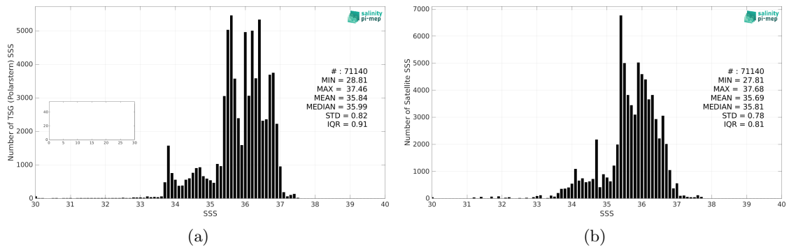
Figure 2: Histograms of SSS from TSG (Polarstern) (a) and Aquarius SSS L3 OR v5 - Monthly - Rain mask (NASA-GSFC) (b) considering all match-up pairs per bins of 0.1 over the Atlantic Ocean Pi-MEP region and for the full satellite product period.
