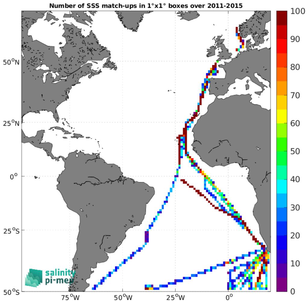
Figure 4: Number of SSS match-ups between TSG (Polarstern) SSS and the Aquarius SSS L3 OR v5 - Monthly - Rain mask (NASA-GSFC) SSS product for the Atlantic Ocean Pi-MEP region over 1°×1° boxes and for the full satellite product period.
