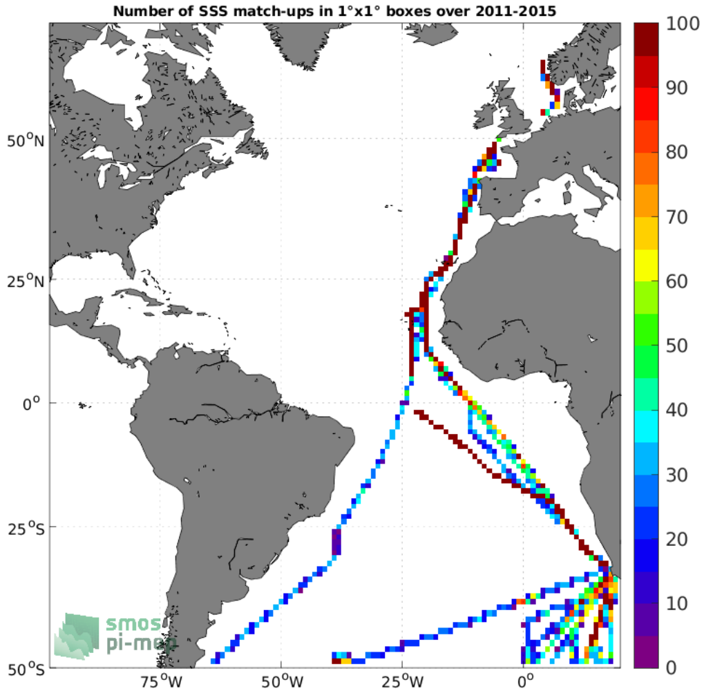
Figure 4: Number of SSS match-ups between TSG (Polarstern) SSS and the Aquarius SSS L3 OR v5 - Monthly - Rain mask (NASA-GSFC) SSS product for the Atlantic Ocean Pi-MEP region over 1°x1° boxes and for the full satellite product period.
