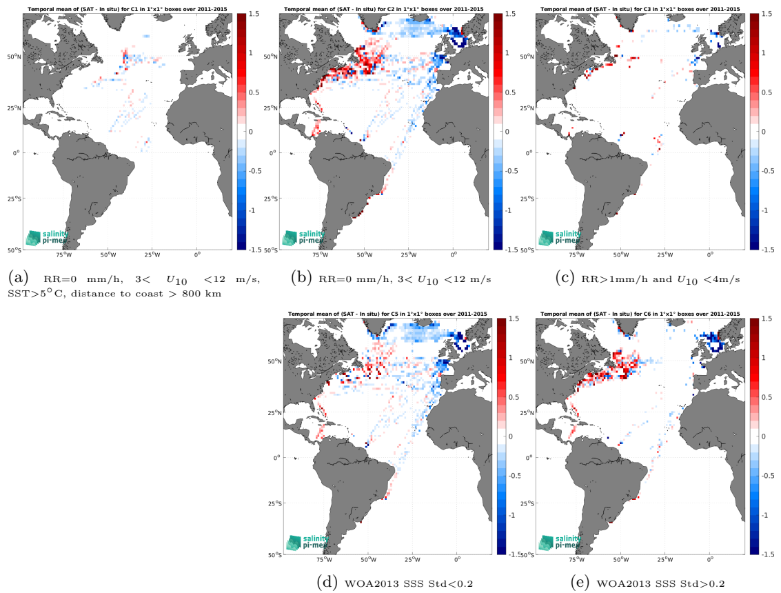
Figure 14: Temporal mean gridded over spatial boxes of size 1^\circ \times 1^\circ of \Delta\text{SSS} (Aquarius SSS L3 OR v5 - Monthly - Rain mask (NASA-GSFC) - TSG (LEGOS-DM)) for 5 different subdatasets corresponding to:RR=0 mm/h, 3 < U_{10} < 12 m/s, SST>5°C, distance to coast > 800 km (a), RR=0 mm/h, 3 < U_{10} < 12 m/s (b), RR>1mm/h and U_{10} < 4 m/s (c), WOA2013 SSS Std<0.2 (d), WOA2013 SSS Std>0.2 (e).
