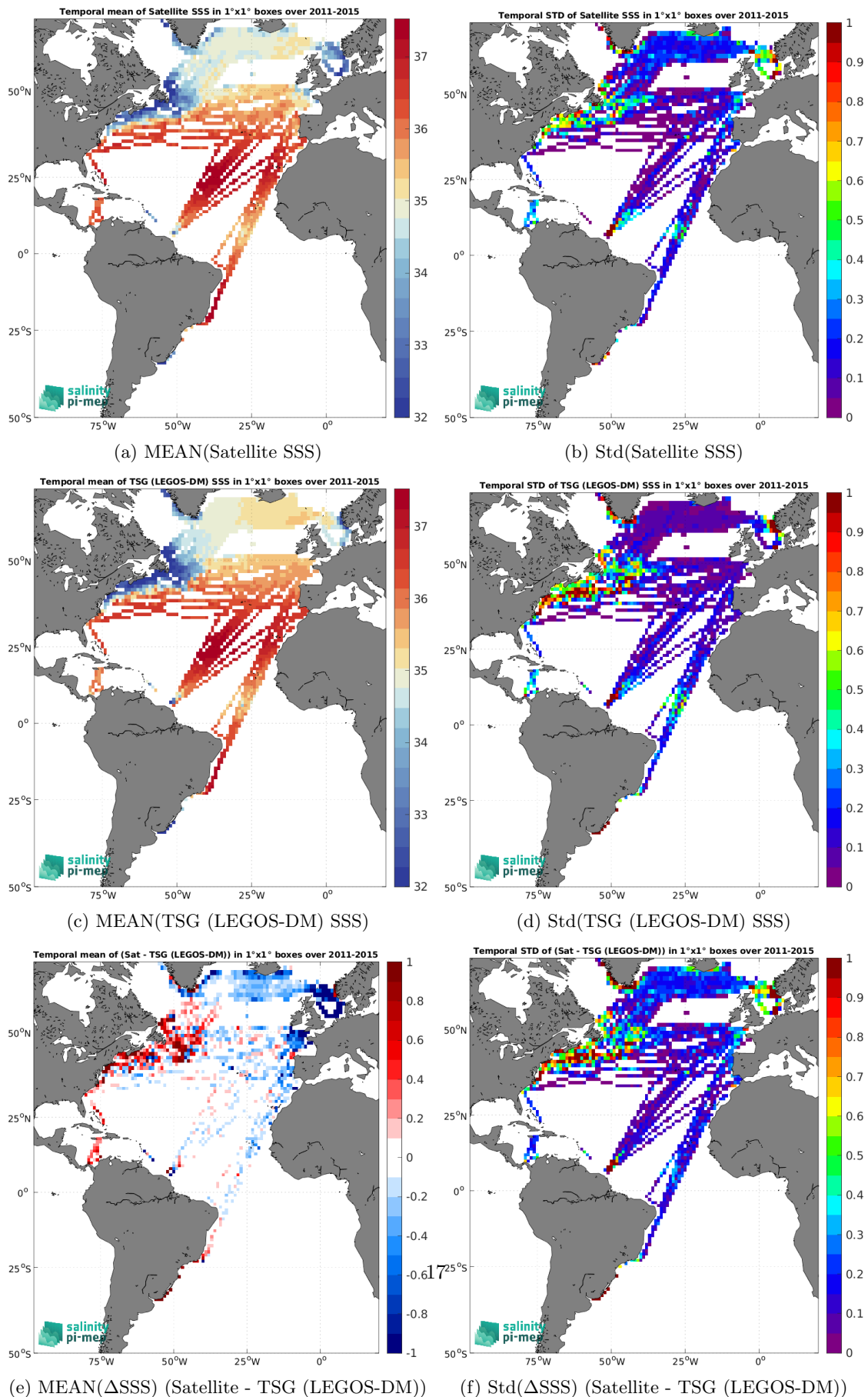
Figure 7: Temporal mean (left) and Std (right) of SSS from Aquarius SSS L3 OR v5 - Monthly - Rain mask (NASA-GSFC) (top), TSG (LEGOS-DM) (middle), and of \Delta SSS (Satellite - TSG (LEGOS-DM)). Only match-up pairs are used to generate these maps.
