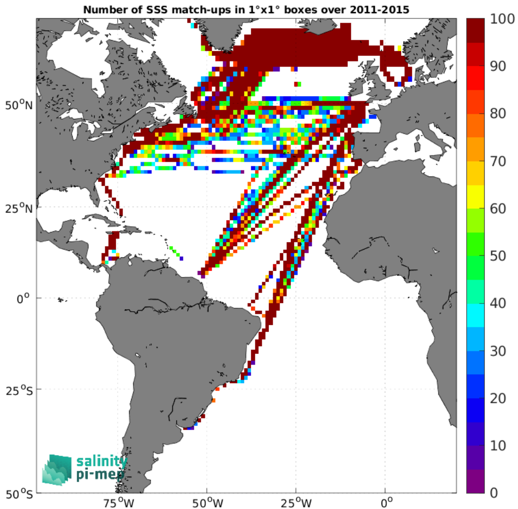
Figure 5: Number of SSS match-ups between TSG (LEGOS-DM) SSS and the Aquarius SSS L3 OR v5 - Monthly - Rain mask (NASA-GSFC) SSS product for the Atlantic Ocean Pi-MEP region over 1^\circ \times 1^\circ boxes and for the full satellite product period.
