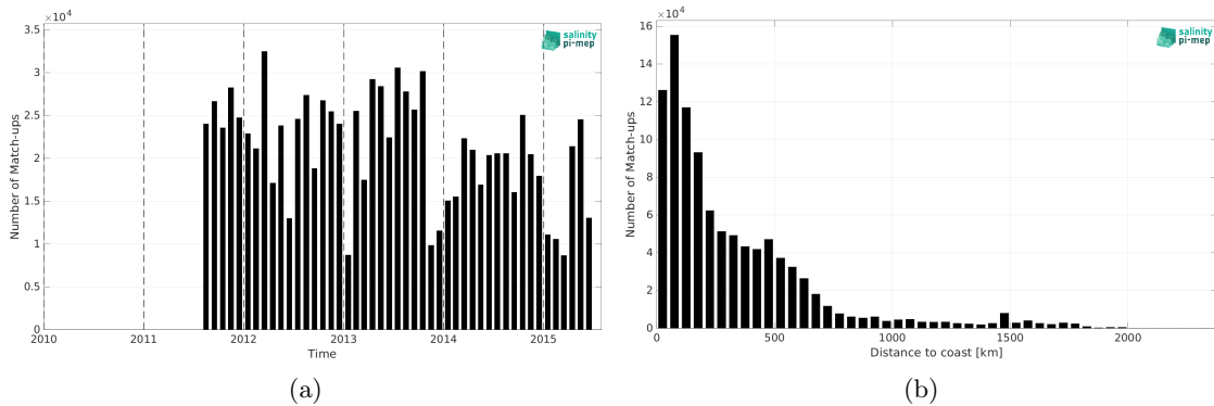
Figure 2: Number of match-ups between TSG (LEGOS-DM) and Aquarius SSS L3 OR v5 - Monthly - Rain mask (NASA-GSFC) SSS as a function of time (a) and as function of the distance to coast (b) over the Atlantic Ocean Pi-MEP region and for the full satellite product period.
