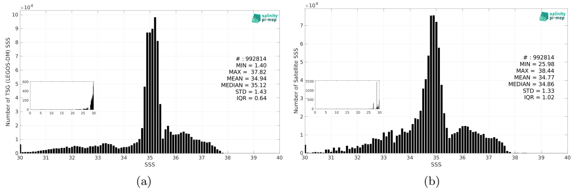
Figure 3: Histograms of SSS from TSG (LEGOS-DM) (a) and Aquarius SSS L3 OR v5 - Monthly - Rain mask (NASA-GSFC) (b) considering all match-up pairs per bins of 0.1 over the Atlantic Ocean Pi-MEP region and for the full satellite product period.
