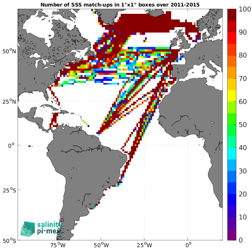
Figure 4: Number of SSS match-ups between TSG (LEGOS-DM) SSS and the Aquarius SSS L3 OR v5 - Monthly - Rain mask (NASA-GSFC) SSS product for the Atlantic Ocean Pi-MEP region over 1^\circ \times 1^\circ boxes and for the full satellite product period.
