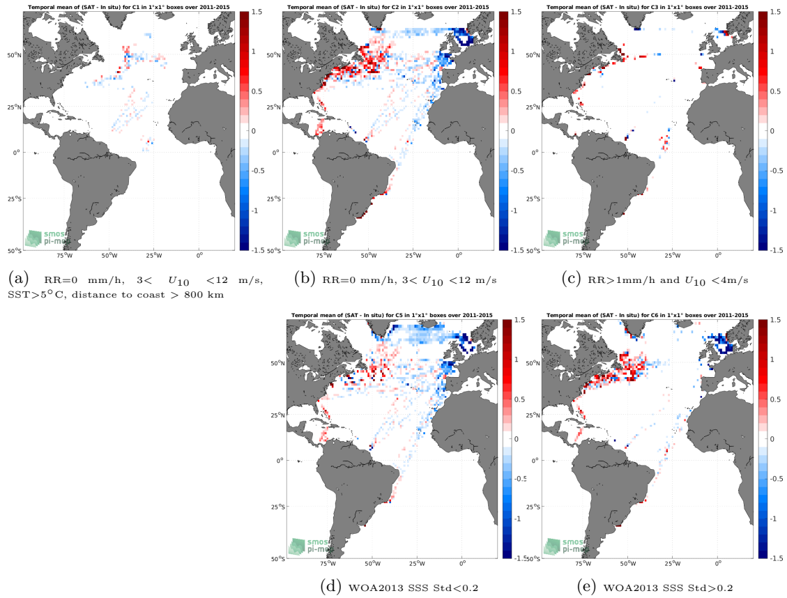
Figure 12: Temporal mean gridded over spatial boxes of size 1^\circ \times 1^\circ of \Delta SSS (Aquarius SSS L3 OR v5 - Monthly - Rain mask (NASA-GSFC) - TSG (LEGOS-DM)) for 5 different subdatasets corresponding to:RR=0 mm/h, 3 < U_{10} < 12 m/s, SST >5^\circ\text{C} , distance to coast > 800 km (a), RR=0 mm/h, 3 < U_{10} < 12 m/s (b), RR >1 mm/h and U_{10} < 4 m/s (c), WOA2013 SSS Std <0.2 (d), WOA2013 SSS Std >0.2 (e).
