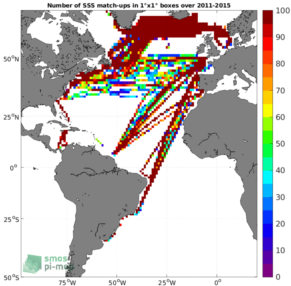
Figure 4: Number of SSS match-ups between TSG (LEGOS-DM) SSS and the Aquarius SSS L3 OR v5 - Monthly - Rain mask (NASA-GSFC) SSS product for the Atlantic Ocean Pi-MEP region over 1°x1° boxes and for the full satellite product period.
