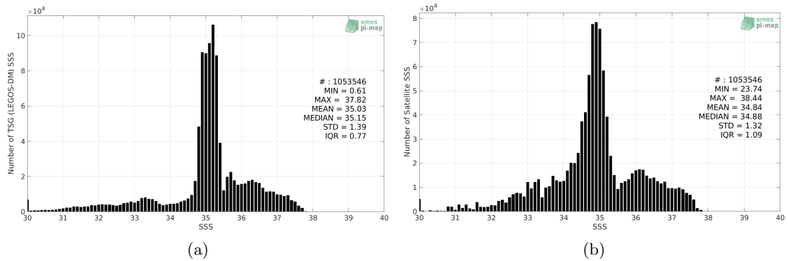
Figure 2: Histograms of SSS from TSG (LEGOS-DM) (a) and Aquarius SSS L3 OR v5 - Monthly - Rain mask (NASA-GSFC) (b) considering all match-up pairs per bins of 0.1 over the Atlantic Ocean Pi-MEP region and for the full satellite product period.
