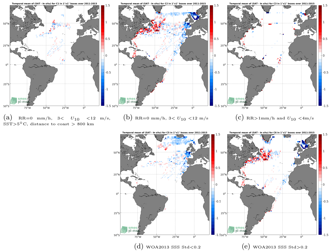
Figure 12: Temporal mean gridded over spatial boxes of size 1^\circ \times 1^\circ of \Delta\text{SSS} (Aquarius SSS L3 OR v5 - Monthly - Rain mask (NASA-GSFC) - TSG (LEGOS-DM)) for 5 different subdatasets corresponding to:RR=0 mm/h, 3 < U_{10} < 12 m/s, SST >5^\circ\text{C} , distance to coast > 800 km (a), RR=0 mm/h, 3 < U_{10} < 12 m/s (b), RR >1 mm/h and U_{10} < 4 m/s (c), WOA2013 SSS Std <0.2 (d), WOA2013 SSS Std >0.2 (e).
