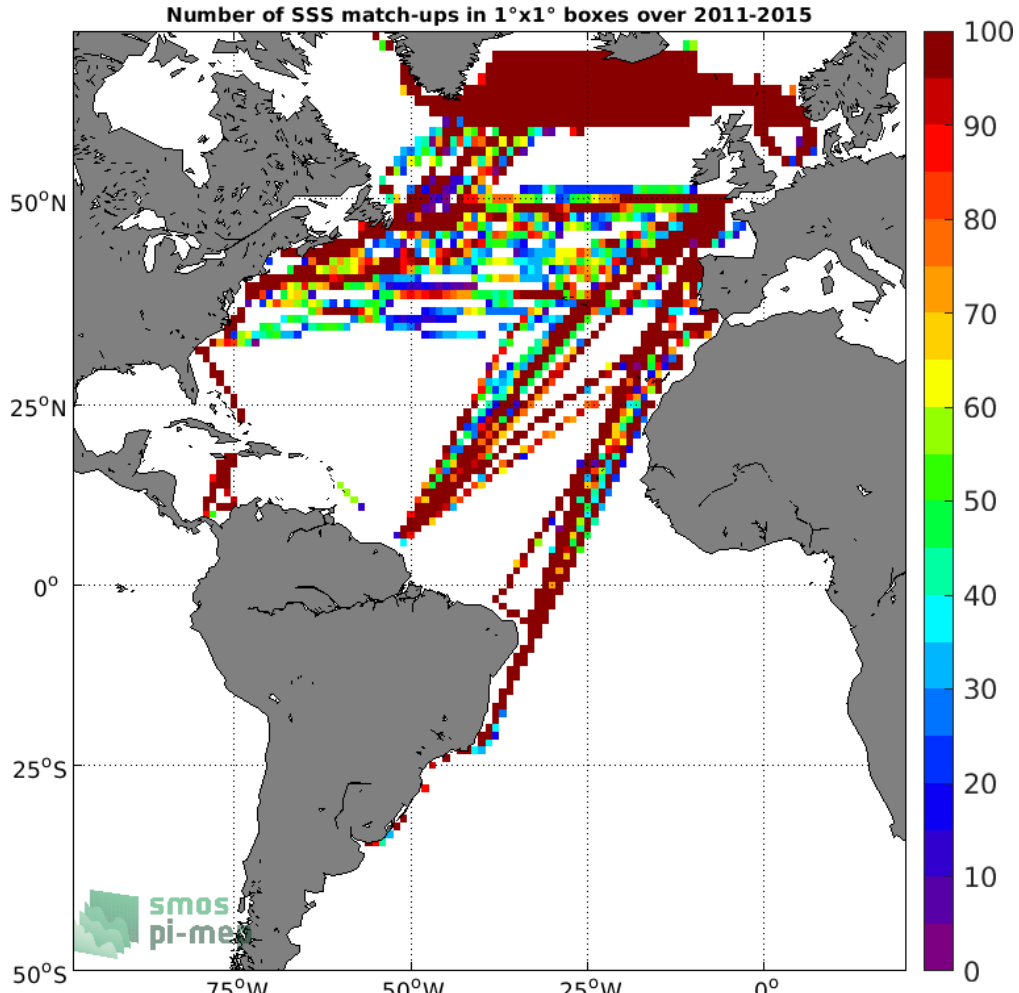
Figure 4: Number of SSS match-ups between TSG (LEGOS-DM) SSS and the Aquarius SSS L3 OR v5 - Monthly - Rain mask (NASA-GSFC) SSS product for the Atlantic Ocean Pi-MEP region over 1^\circ \times 1^\circ boxes and for the full satellite product period.
