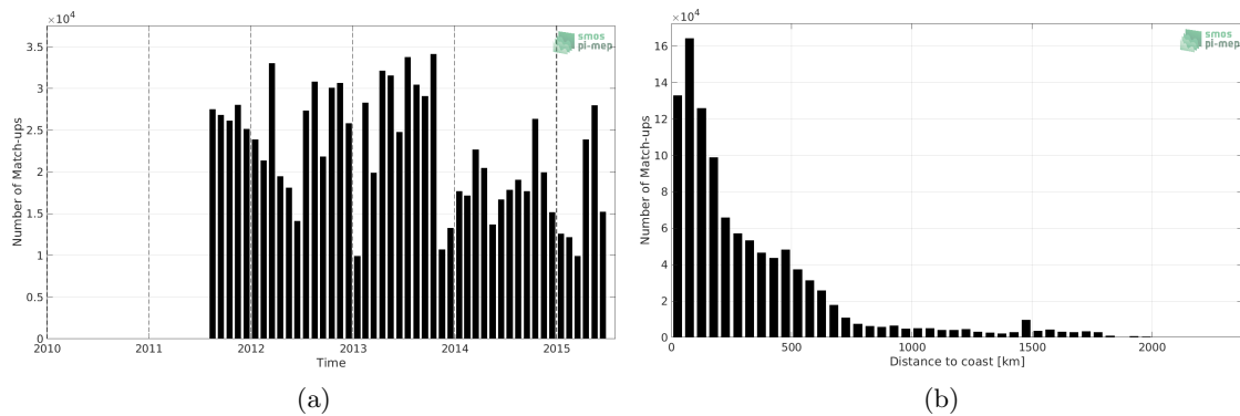
Figure 1: Number of match-ups between TSG (LEGOS-DM) and Aquarius SSS L3 OR v5 - Monthly - Rain mask (NASA-GSFC) SSS as a function of time (a) and as function of the distance to coast (b) over the Atlantic Ocean Pi-MEP region and for the full satellite product period.
