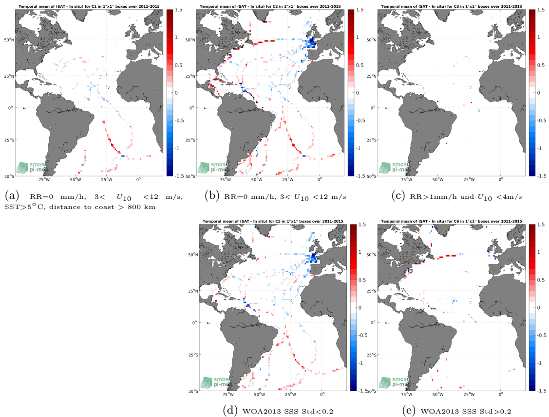
Figure 12: Temporal mean gridded over spatial boxes of size 1^\circ \times 1^\circ of \Delta SSS (Aquarius SSS L3 OR v5 - Monthly - Rain mask (NASA-GSFC) - TSG (GOSUD-Sailing-ship)) for 5 different subdatasets corresponding to:RR=0 mm/h, 3 < U_{10} < 12 m/s, SST>5°C, distance to coast > 800 km (a), RR=0 mm/h, 3 < U_{10} < 12 m/s (b), RR>1mm/h and U_{10} < 4 m/s (c), WOA2013 SSS Std<0.2 (d), WOA2013 SSS Std>0.2 (e).
