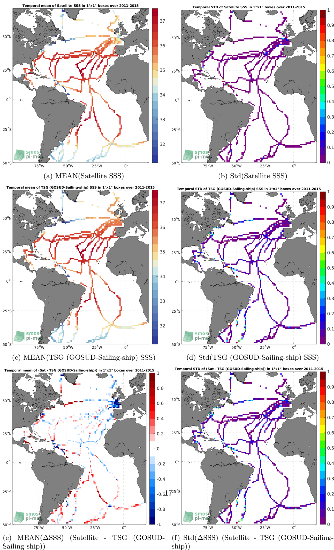
Figure 6: Temporal mean (left) and Std (right) of SSS from Aquarius SSS L3 OR v5 - Monthly - Rain mask (NASA-GSFC) (top), TSG (GOSUD-Sailing-ship) (middle), and of \Delta SSS (Satellite - TSG (GOSUD-Sailing-ship)). Only match-up pairs are used to generate these maps.
