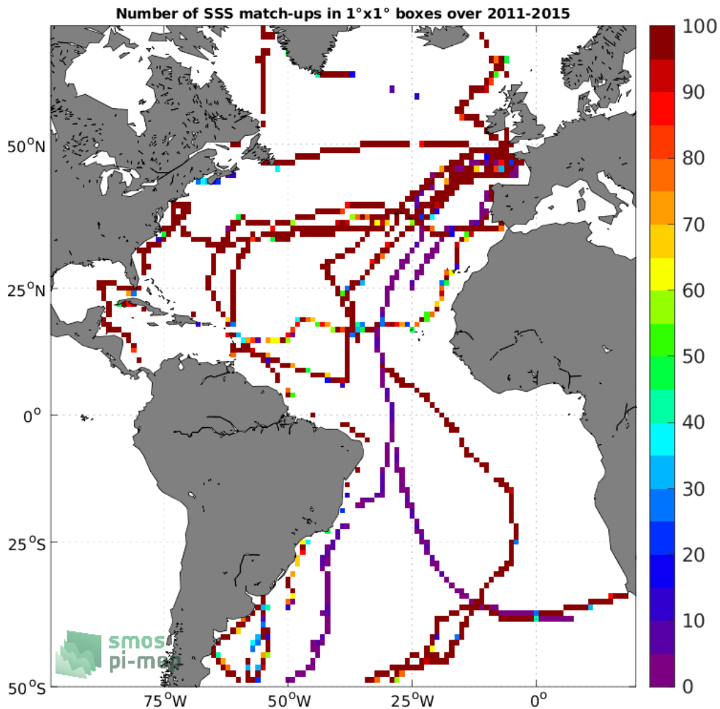
Figure 4: Number of SSS match-ups between TSG (GOSUD-Sailing-ship) SSS and the Aquarius SSS L3 OR v5 - Monthly - Rain mask (NASA-GSFC) SSS product for the Atlantic Ocean Pi-MEP region over 1°x1° boxes and for the full satellite product period.
