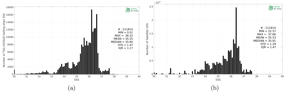
Figure 2: Histograms of SSS from TSG (GOSUD-Sailing-ship) (a) and Aquarius SSS L3 OR v5 - Monthly - Rain mask (NASA-GSFC) (b) considering all match-up pairs per bins of 0.1 over the Atlantic Ocean Pi-MEP region and for the full satellite product period.
