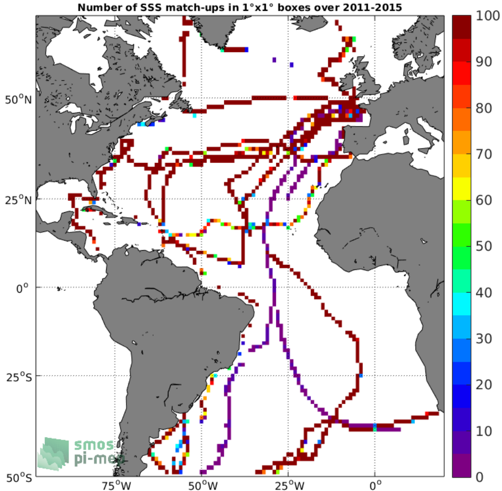
Figure 4: Number of SSS match-ups between TSG (GOSUD-Sailing-ship) SSS and the Aquarius SSS L3 OR v5 - Monthly - Rain mask (NASA-GSFC) SSS product for the Atlantic Ocean Pi-MEP region over 1^\circ \times 1^\circ boxes and for the full satellite product period.
