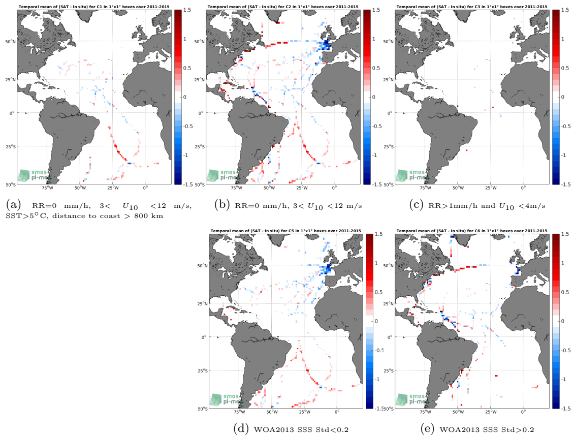
Figure 12: Temporal mean gridded over spatial boxes of size 1^\circ \times 1^\circ of \Delta\text{SSS} (Aquarius SSS L3 OR v5 - Monthly - Rain mask (NASA-GSFC) - TSG (GOSUD-Sailing-ship)) for 5 different subdatasets corresponding to:RR=0 mm/h, 3 < U_{10} < 12 m/s, SST>5°C, distance to coast > 800 km (a), RR=0 mm/h, 3 < U_{10} < 12 m/s (b), RR>1mm/h and U_{10} < 4 m/s (c), WOA2013 SSS Std<0.2 (d), WOA2013 SSS Std>0.2 (e).
