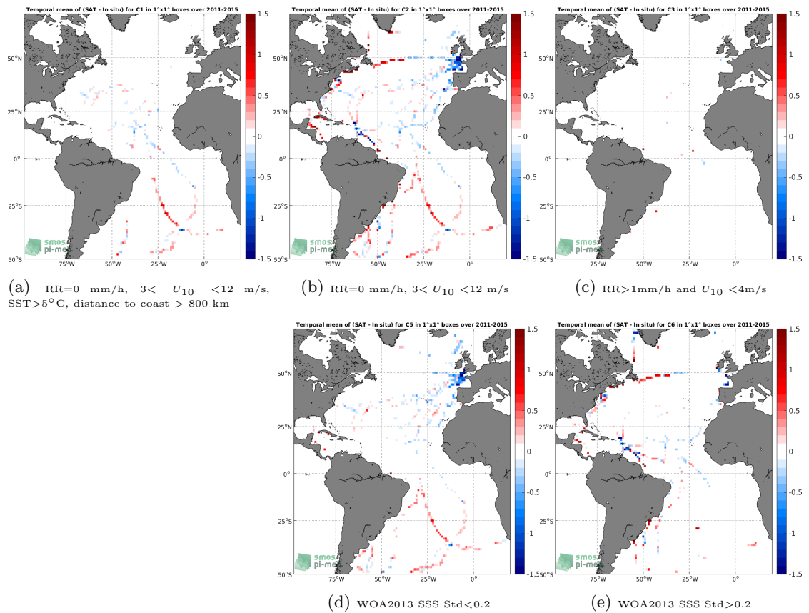
Figure 12: Temporal mean gridded over spatial boxes of size 1^\circ \times 1^\circ of \Delta\text{SSS} (Aquarius-L3-OR-V5-MONTHLY-RAIN-MASK-1DEG - TSG-GOSUD-Sailing-ship) for 5 different subdatasets corresponding to:RR=0 mm/h, 3 < U_{10} < 12 m/s, SST>5°C, distance to coast > 800 km (a), RR=0 mm/h, 3 < U_{10} < 12 m/s (b), RR>1mm/h and U_{10} < 4 m/s (c), WOA2013 SSS Std<0.2 (d), WOA2013 SSS Std>0.2 (e).
