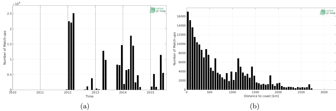
Figure 1: Number of match-ups between TSG-GOSUD-Sailing-ship and Aquarius-L3-OR-V5-MONTHLY-RAIN-MASK-1DEG SSS as a function of time (a) and as function of the distance to coast (b) over the Atlantic Ocean Pi-MEP region and for the full satellite product period.
