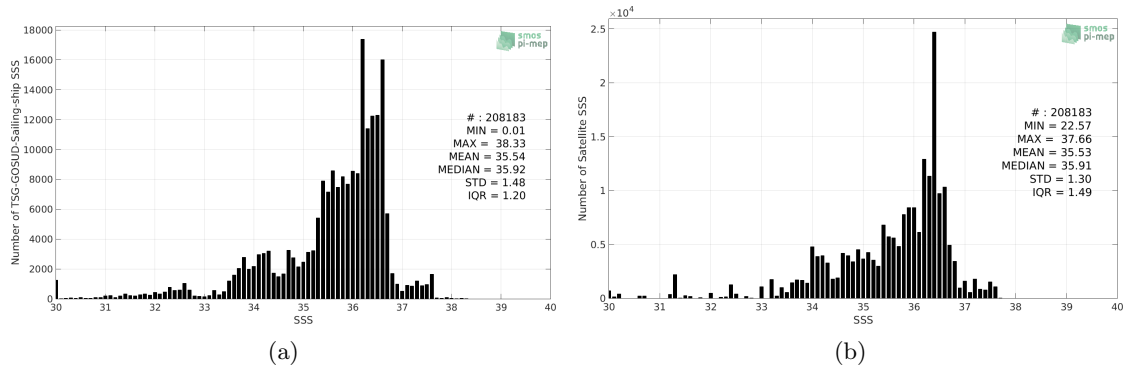
Figure 2: Histograms of SSS from TSG-GOSUD-Sailing-ship (a) and Aquarius-L3-OR-V5-MONTHLY-RAIN-MASK-1DEG (b) considering all match-up pairs per bins of 0.1 over the Atlantic Ocean Pi-MEP region and for the full satellite product period.
