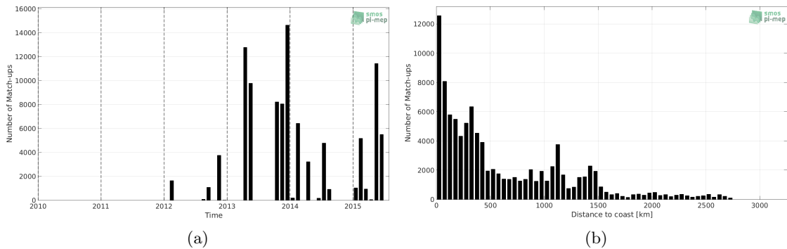
Figure 1: Number of match-ups between TSG-GOSUD-Sailing-ship and Aquarius-L3-OR-V5-MONTHLY-RAIN-MASK-1DEG SSS as a function of time (a) and as function of the distance to coast (b) over the Atlantic Ocean Pi-MEP region and for the full satellite product period.
