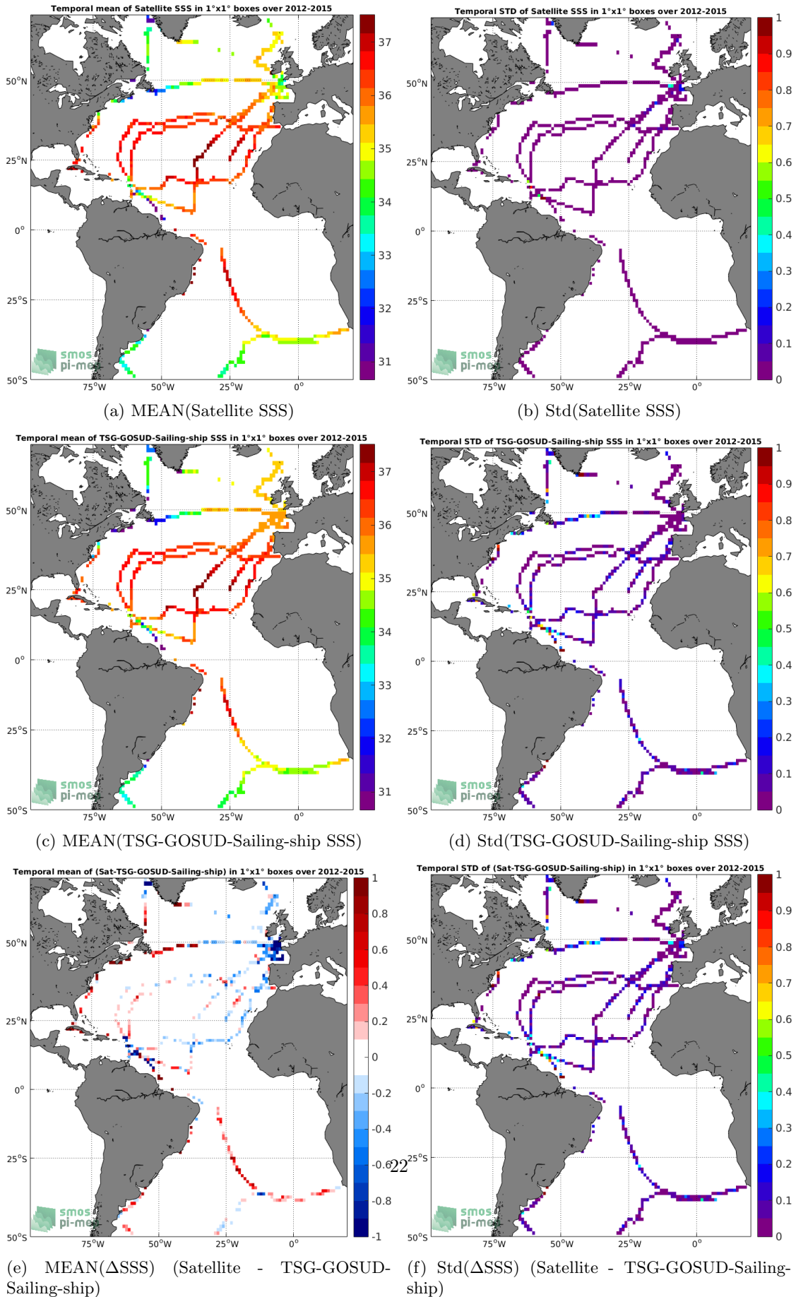
Figure 6: Temporal mean (left) and Std (right) of SSS from Aquarius-L3-OR-V5-MONTHLY-RAIN-MASK-1DEG (top), TSG-GOSUD-Sailing-ship (middle), and of \Delta SSS (Satellite - TSG-GOSUD-Sailing-ship). Only match-up pairs are used to generate these maps.
