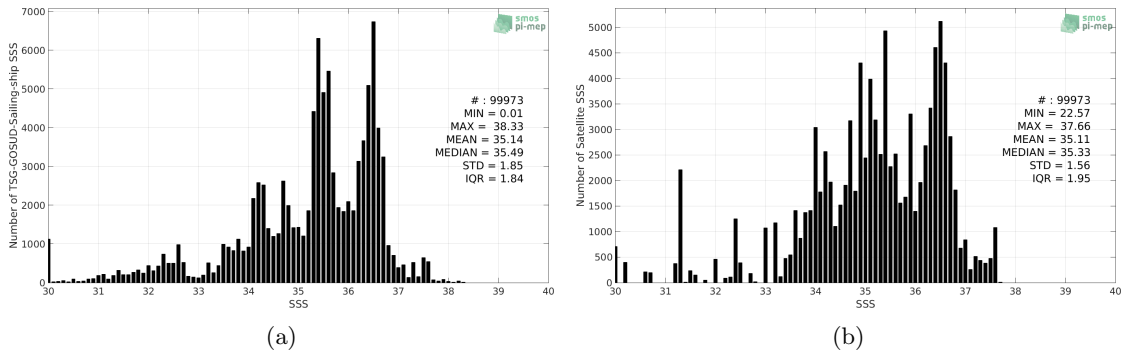
Figure 2: Histograms of SSS from TSG-GOSUD-Sailing-ship (a) and Aquarius-L3-OR-V5-MONTHLY-RAIN-MASK-1DEG (b) considering all match-up pairs per bins of 0.1 over the Atlantic Ocean Pi-MEP region and for the full satellite product period.
