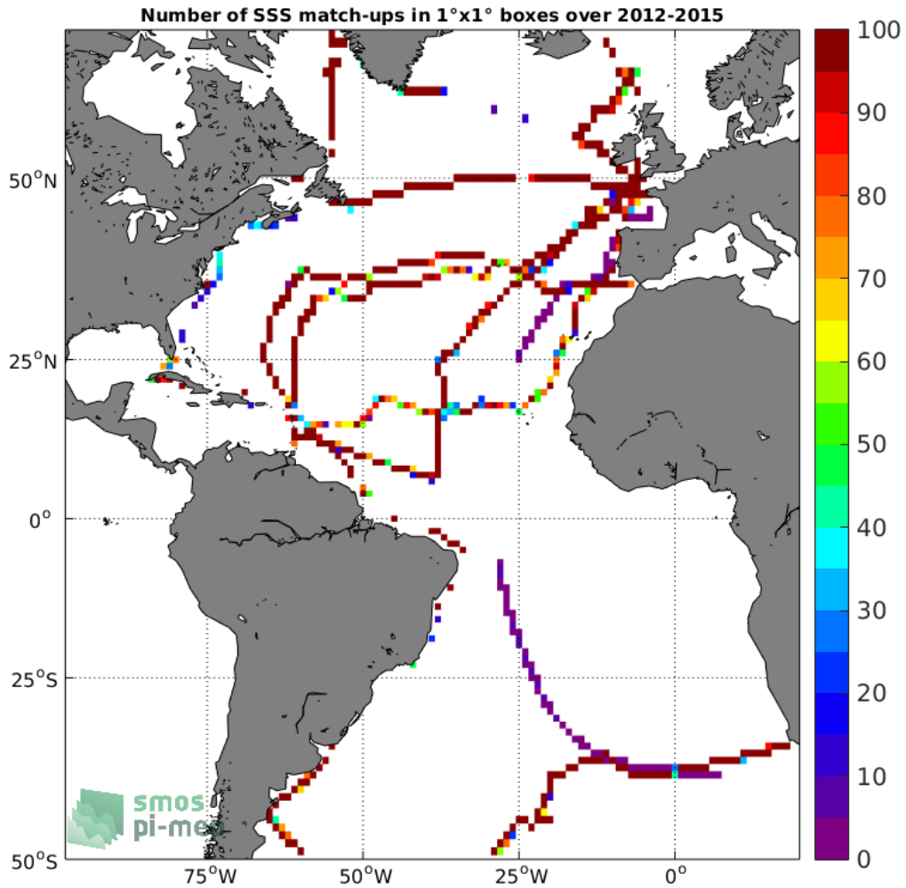
Figure 4: Number of SSS match-ups between TSG-GOSUD-Sailing-ship SSS and the Aquarius-L3-OR-V5-MONTHLY-RAIN-MASK-1DEG SSS product for the Atlantic Ocean Pi-MEP region over 1°x1° boxes and for the full satellite product period.
