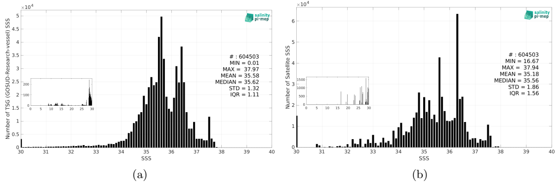
Figure 3: Histograms of SSS from TSG (GOSUD-Research-vessel) (a) and Aquarius SSS L3 OR v5 - Monthly - Rain mask (NASA-GSFC) (b) considering all match-up pairs per bins of 0.1 over the Atlantic Ocean Pi-MEP region and for the full satellite product period.
