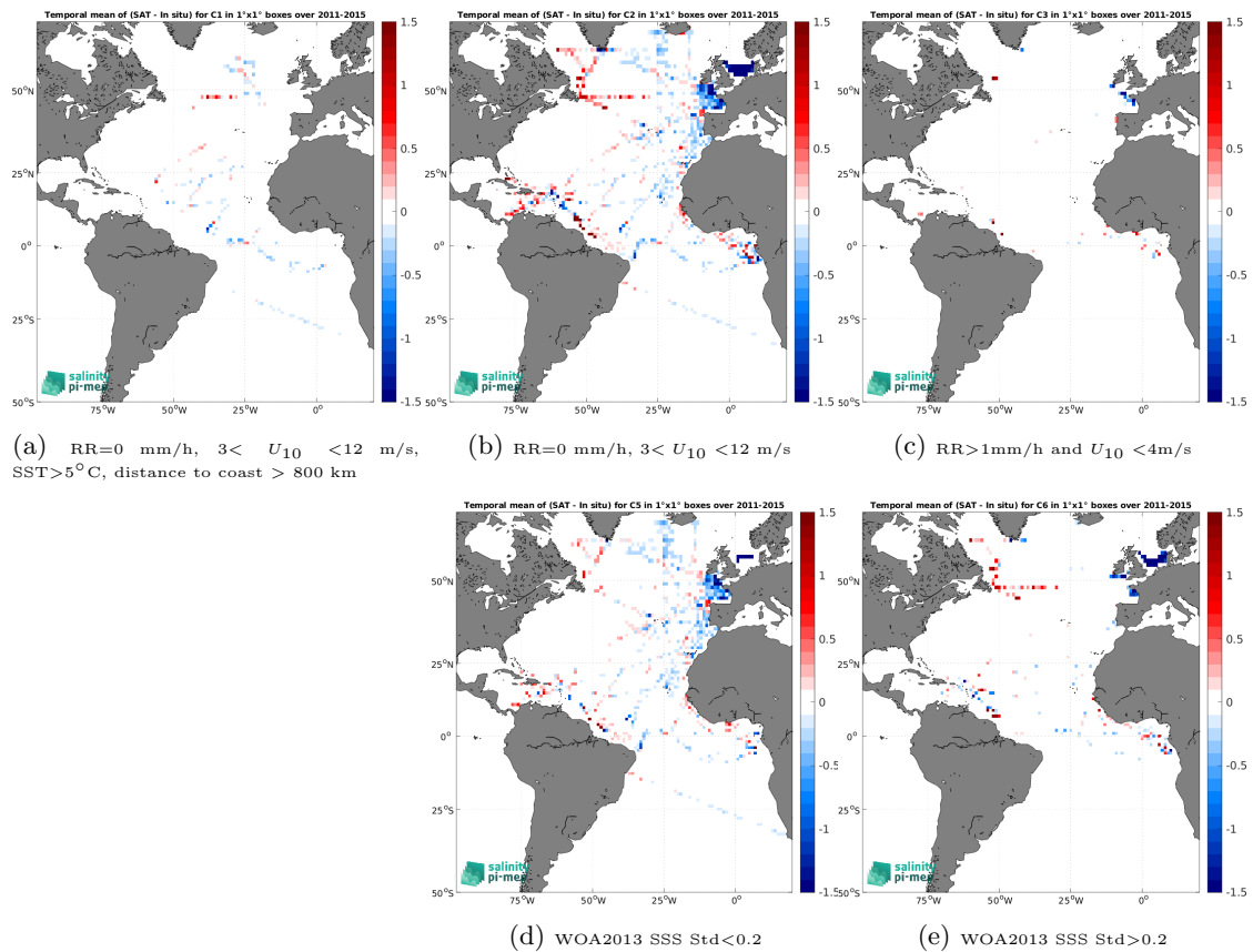
Figure 14: Temporal mean gridded over spatial boxes of size 1^\circ \times 1^\circ of \Delta\text{SSS} (Aquarius SSS L3 OR v5 - Monthly - Rain mask (NASA-GSFC) - TSG (GOSUD-Research-vessel)) for 5 different subdatasets corresponding to:RR=0 mm/h, 3 < U_{10} < 12 m/s, SST >5^\circ\text{C} , distance to coast > 800 km (a), RR=0 mm/h, 3 < U_{10} < 12 m/s (b), RR >1 mm/h and U_{10} < 4 m/s (c), WOA2013 SSS Std <0.2 (d), WOA2013 SSS Std >0.2 (e).
