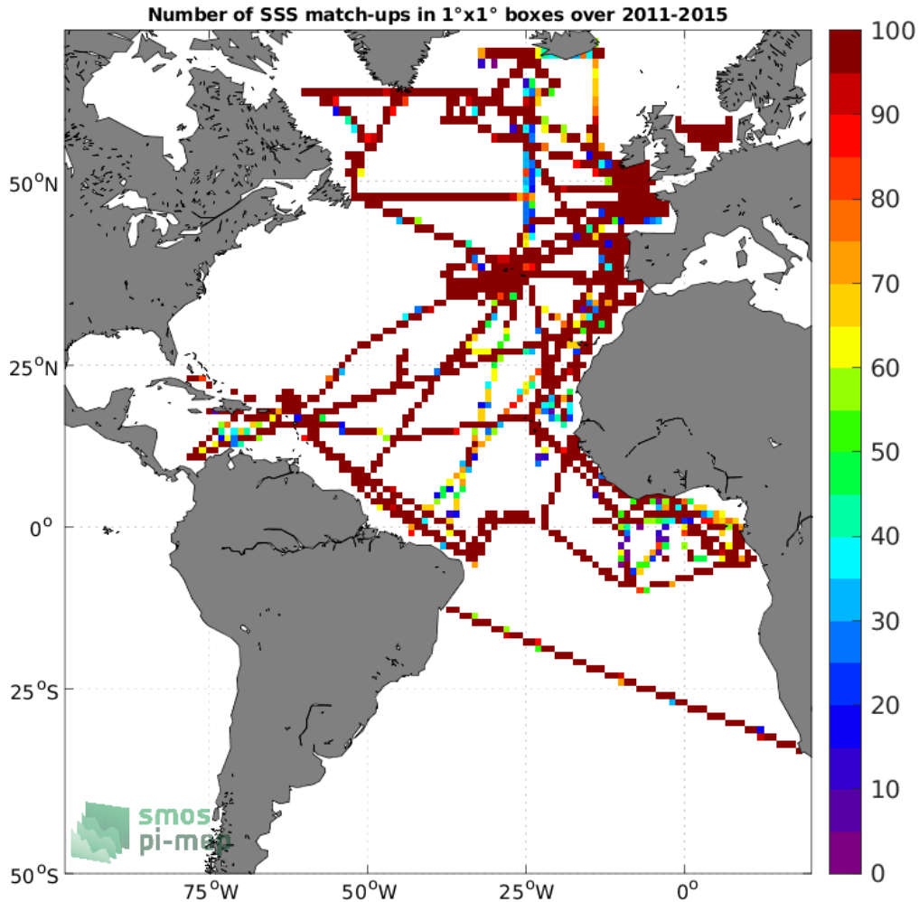
Figure 4: Number of SSS match-ups between TSG (GOSUD-Research-vessel) SSS and the Aquarius SSS L3 OR v5 - Monthly - Rain mask (NASA-GSFC) SSS product for the Atlantic Ocean Pi-MEP region over 1°x1° boxes and for the full satellite product period.
