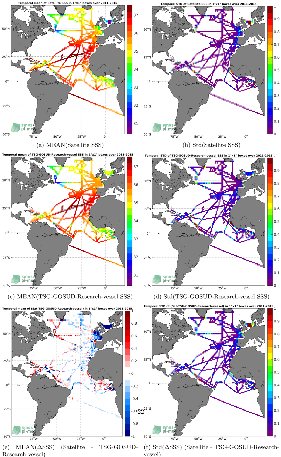
Figure 6: Temporal mean (left) and Std (right) of SSS from Aquarius-L3-OR-V5-MONTHLY-RAIN-MASK-1DEG (top), TSG-GOSUD-Research-vessel (middle), and of ΔSSS (Satellite - TSG-GOSUD-Research-vessel). Only match-up pairs are used to generate these maps.
