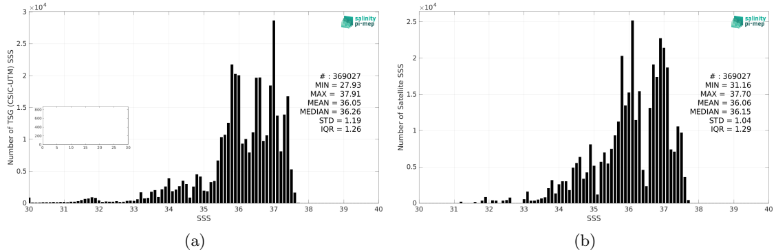
Figure 2: Histograms of SSS from TSG (CSIC-UTM) (a) and Aquarius SSS L3 OR v5 - Monthly - Rain mask (NASA-GSFC) (b) considering all match-up pairs per bins of 0.1 over the Atlantic Ocean Pi-MEP region and for the full satellite product period.
