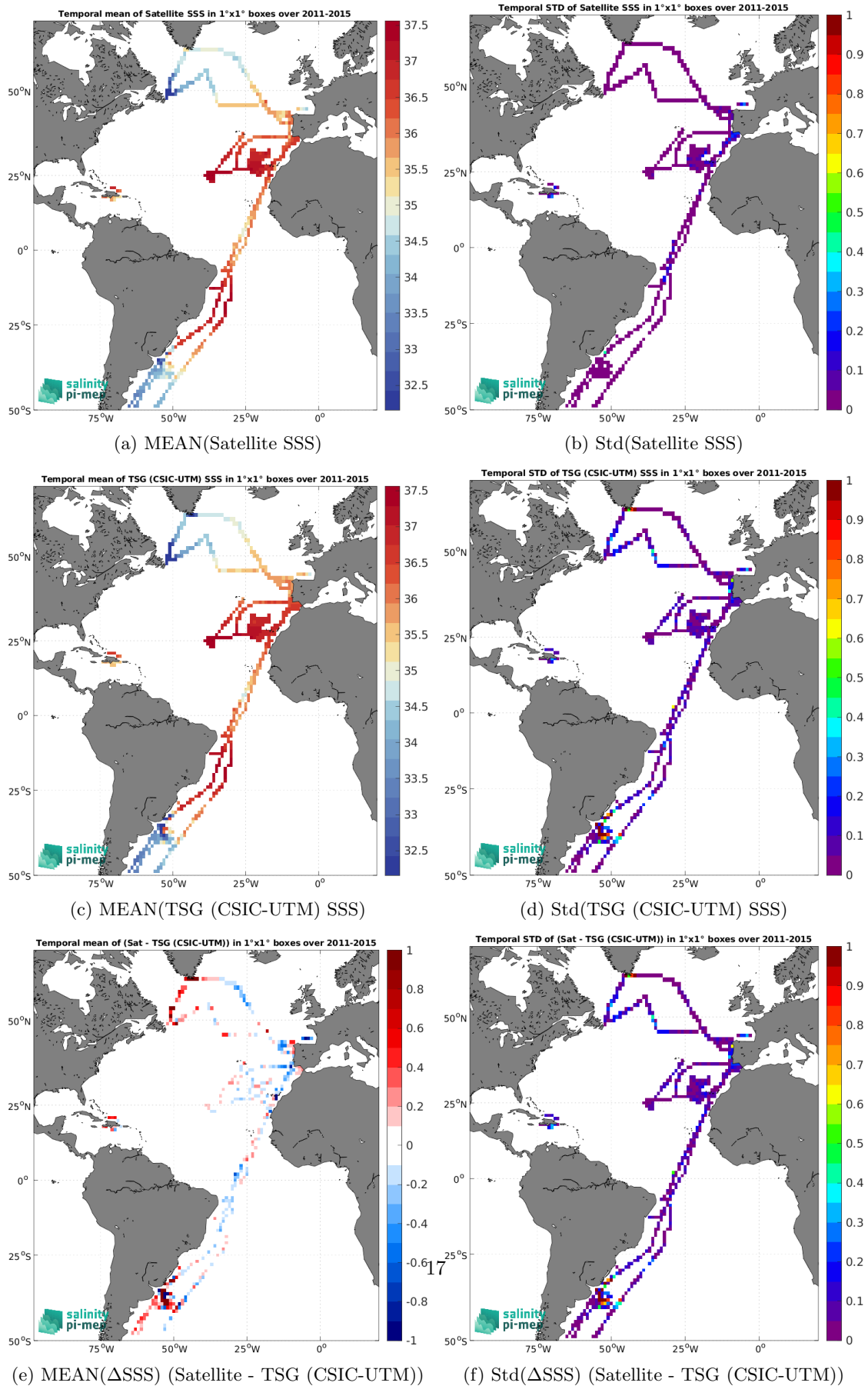
Figure 6: Temporal mean (left) and Std (right) of SSS from Aquarius SSS L3 OR v5 - Monthly - Rain mask (NASA-GSFC) (top), TSG (CSIC-UTM) (middle), and of \Delta SSS (Satellite - TSG (CSIC-UTM)). Only match-up pairs are used to generate these maps.
