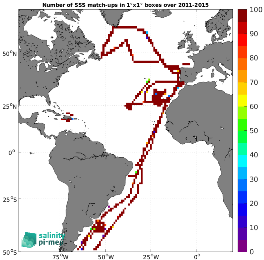
Figure 4: Number of SSS match-ups between TSG (CSIC-UTM) SSS and the Aquarius SSS L3 OR v5 - Monthly - Rain mask (NASA-GSFC) SSS product for the Atlantic Ocean Pi-MEP region over 1^\circ \times 1^\circ boxes and for the full satellite product period.
