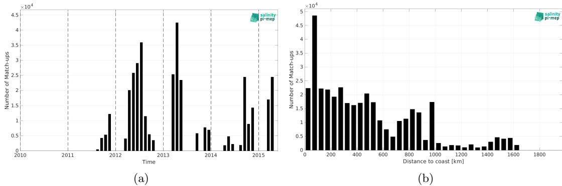
Figure 1: Number of match-ups between TSG (CSIC-UTM) and Aquarius SSS L3 OR v5 - Monthly - Rain mask (NASA-GSFC) SSS as a function of time (a) and as function of the distance to coast (b) over the Atlantic Ocean Pi-MEP region and for the full satellite product period.
