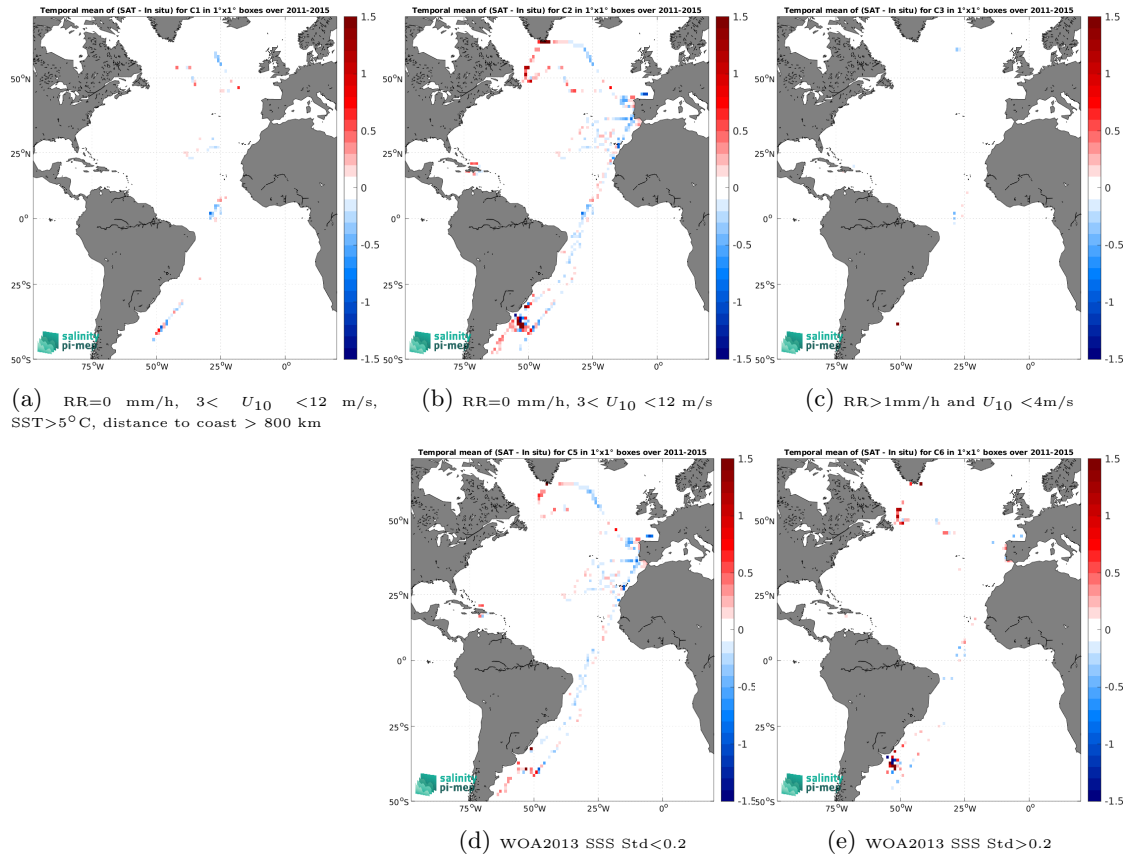
Figure 12: Temporal mean gridded over spatial boxes of size 1^\circ \times 1^\circ of \Delta SSS (Aquarius SSS L3 OR v5 - Monthly - Rain mask (NASA-GSFC) - TSG (CSIC-UTM)) for 5 different subdatasets corresponding to:RR=0 mm/h, 3 < U_{10} < 12 m/s, SST >5^\circ\text{C} , distance to coast > 800 km (a), RR=0 mm/h, 3 < U_{10} < 12 m/s (b), RR >1 mm/h and U_{10} < 4 m/s (c), WOA2013 SSS Std <0.2 (d), WOA2013 SSS Std >0.2 (e).
