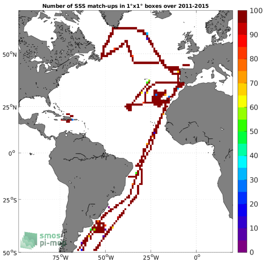
Figure 4: Number of SSS match-ups between TSG (CSIC-UTM) SSS and the Aquarius SSS L3 OR v5 - Monthly - Rain mask (NASA-GSFC) SSS product for the Atlantic Ocean Pi-MEP region over 1°x1° boxes and for the full satellite product period.
