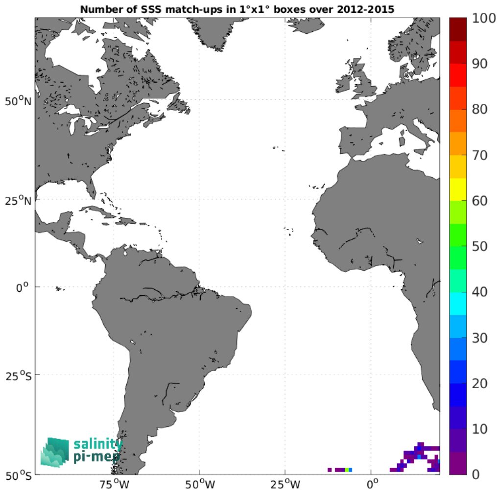
Figure 4: Number of SSS match-ups between Marine mammals SSS and the Aquarius SSS L3 OR v5 - Monthly - Rain mask (NASA-GSFC) SSS product for the Atlantic Ocean Pi-MEP region over 1^{\circ} \times 1^{\circ} boxes and for the full satellite product period.
