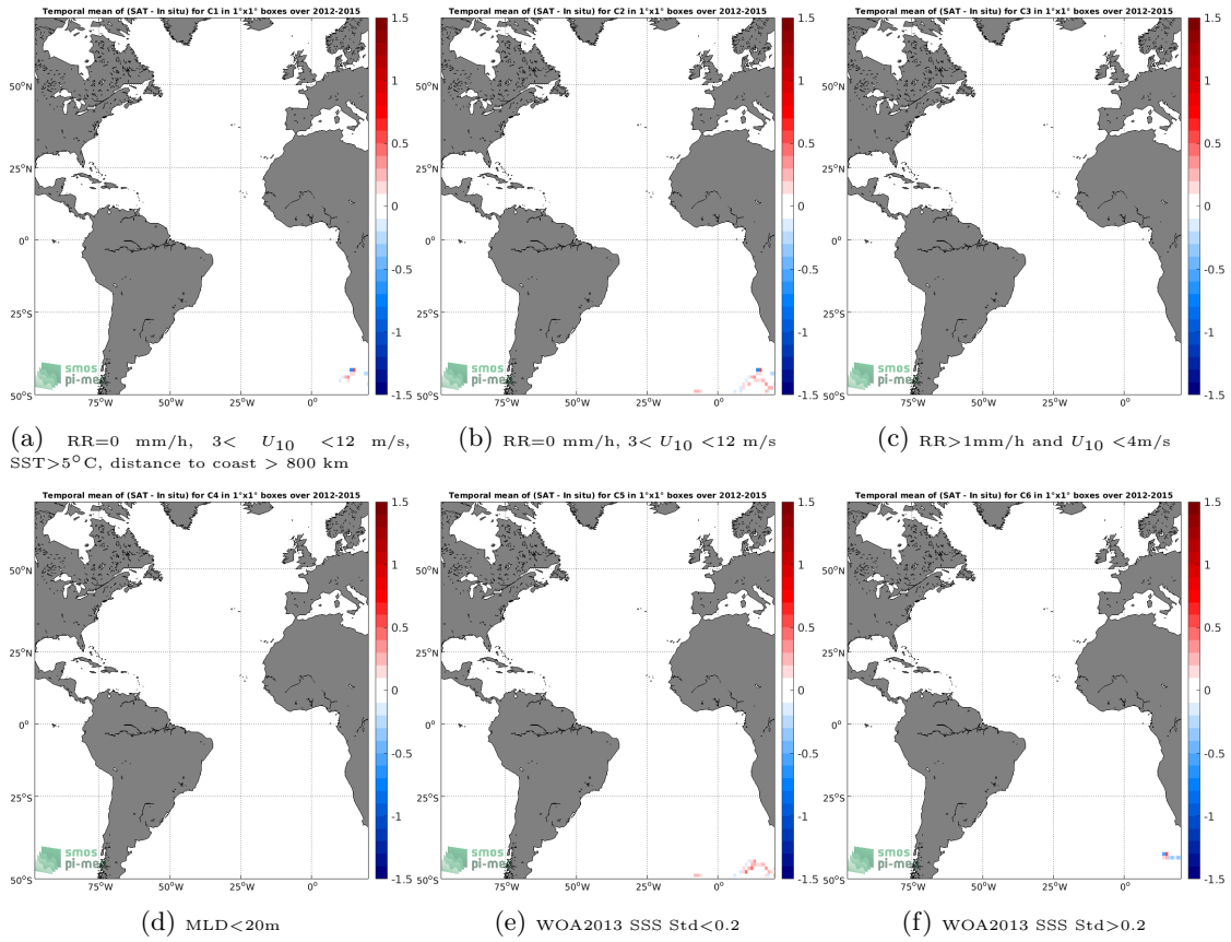
Figure 12: Temporal mean gridded over spatial boxes of size 1^\circ \times 1^\circ of \Delta\text{SSS} (Aquarius SSS L3 OR v5 - Monthly - Rain mask (NASA-GSFC) - Marine mammals) for 6 different subdatasets corresponding to: RR=0 mm/h, 3 < U_{10} < 12 m/s, SST > 5^\circ\text{C} , distance to coast > 800 km (a), RR=0 mm/h, 3 < U_{10} < 12 m/s (b), RR > 1 mm/h and U_{10} < 4 m/s (c), MLD < 20 m (d), WOA2013 SSS Std < 0.2 (e), WOA2013 SSS Std > 0.2 (f).
