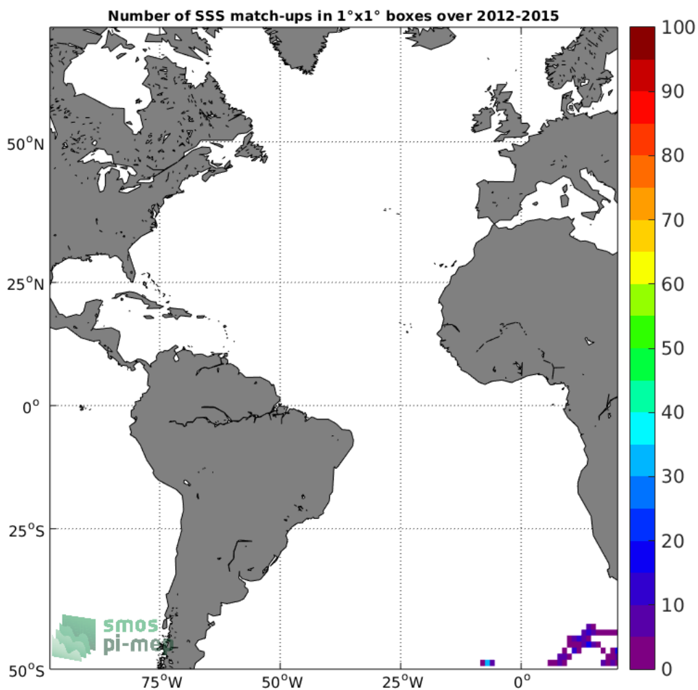
Figure 4: Number of SSS match-ups between Sea mammals SSS and the Aquarius-L3-OR-V5-MONTHLY-RAIN-MASK-1DEG SSS product for the Atlantic Ocean Pi-MEP region over 1°x1° boxes and for the full satellite product period.
