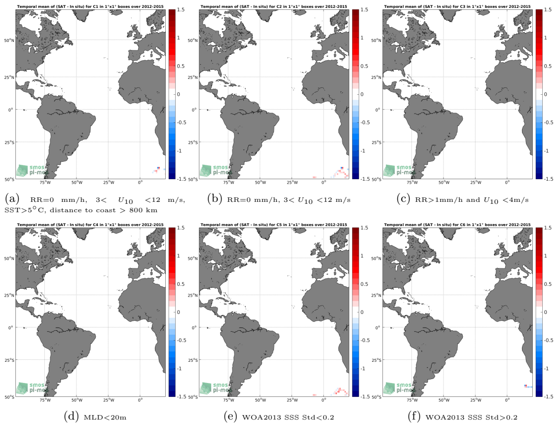
Figure 12: Temporal mean gridded over spatial boxes of size 1°x1° of \Delta SSS (Aquarius-L3-OR-V5-MONTHLY-RAIN-MASK-1DEG - Sea mammals) for 6 different subdatasets corresponding to:RR=0 mm/h, 3 < U_{10} < 12 m/s, SST>5°C, distance to coast > 800 km (a), RR=0 mm/h, 3 < U_{10} < 12 m/s (b), RR>1mm/h and U_{10} < 4 m/s (c),MLD<20m (d),WOA2013 SSS Std<0.2 (e),WOA2013 SSS Std>0.2 (f).
