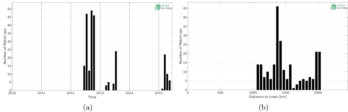
Figure 1: Number of match-ups between Sea mammals and Aquarius-L3-OR-V5-MONTHLY-RAIN-MASK-1DEG SSS as a function of time (a) and as function of the distance to coast (b) over the Atlantic Ocean Pi-MEP region and for the full satellite product period.
