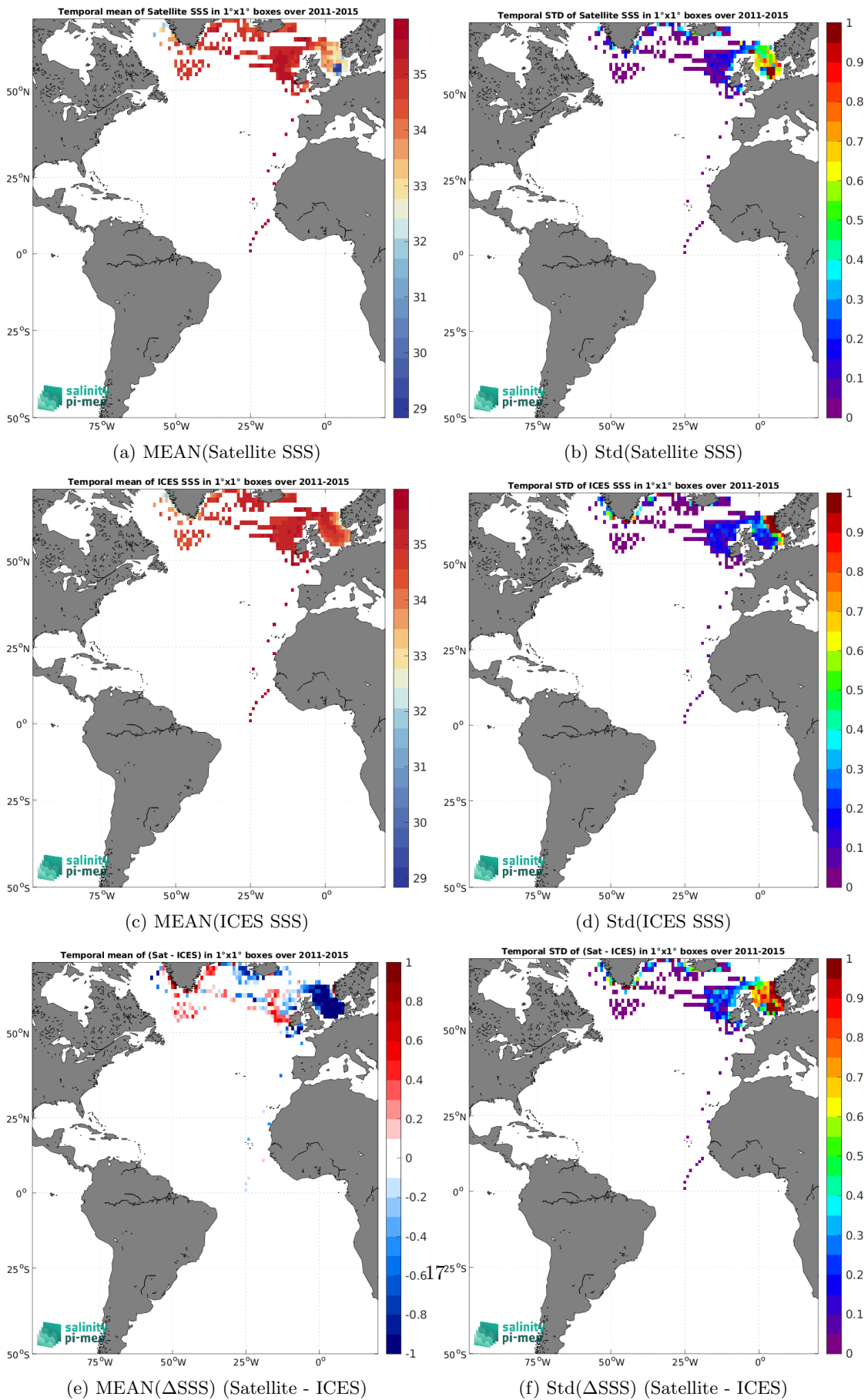
Figure 7: Temporal mean (left) and Std (right) of SSS from Aquarius SSS L3 OR v5 - Monthly - Rain mask (NASA-GSFC) (top), ICES (middle), and of \Delta SSS (Satellite - ICES). Only match-up pairs are used to generate these maps.
