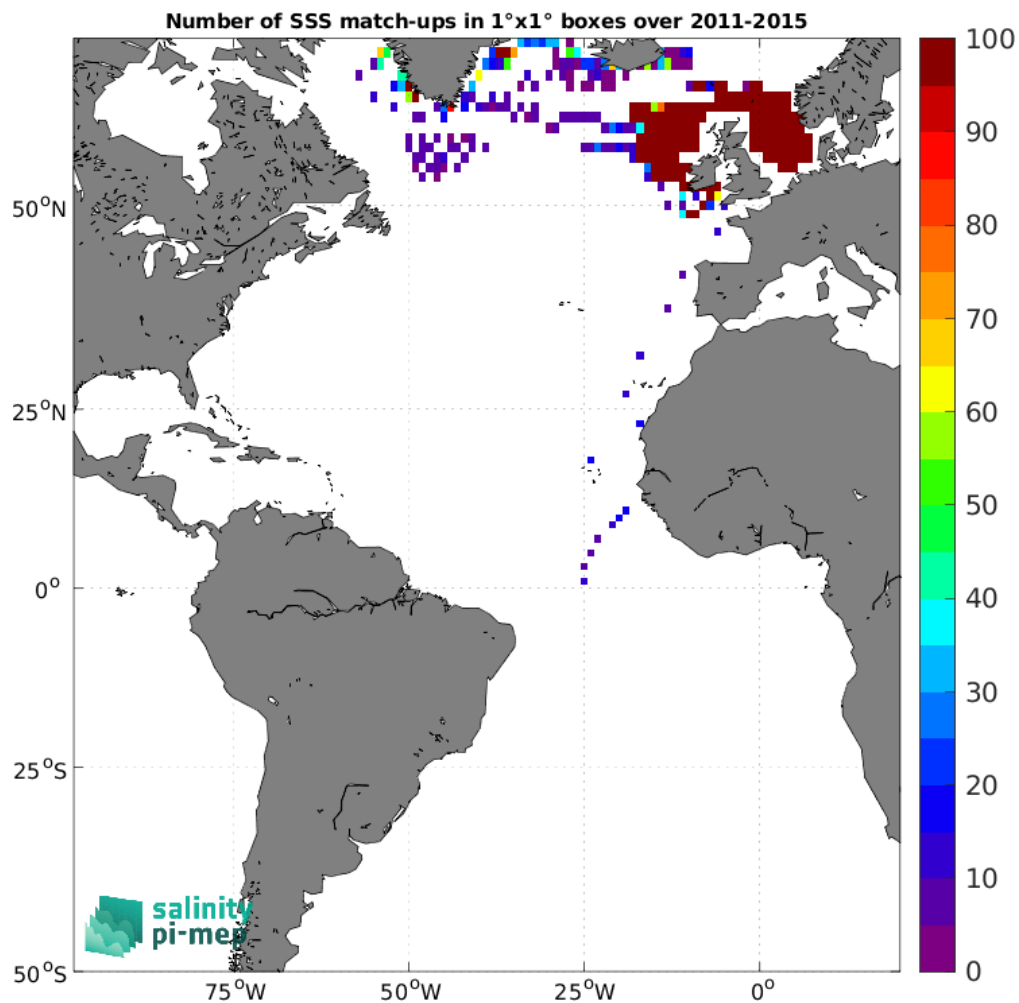
Figure 5: Number of SSS match-ups between ICES SSS and the Aquarius SSS L3 OR v5 - Monthly - Rain mask (NASA-GSFC) SSS product for the Atlantic Ocean Pi-MEP region over 1°×1° boxes and for the full satellite product period.
