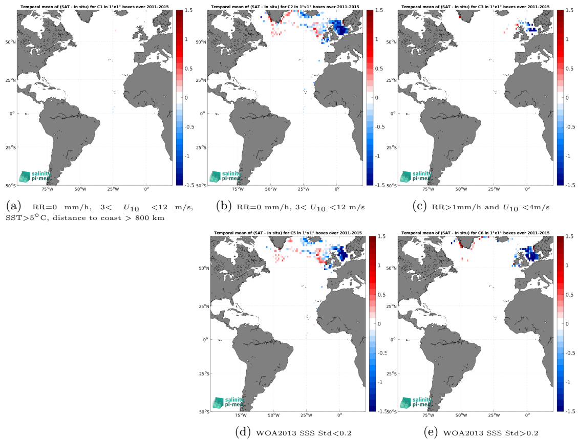
Figure 14: Temporal mean gridded over spatial boxes of size 1^\circ \times 1^\circ of \Delta\text{SSS} (Aquarius SSS L3 OR v5 - Monthly - Rain mask (NASA-GSFC) - ICES) for 5 different subdatasets corresponding to:RR=0 mm/h, 3 < U_{10} < 12 m/s, SST>5°C, distance to coast > 800 km (a), RR=0 mm/h, 3 < U_{10} < 12 m/s (b), RR>1mm/h and U_{10} < 4 m/s (c), WOA2013 SSS Std<0.2 (d), WOA2013 SSS Std>0.2 (e).
