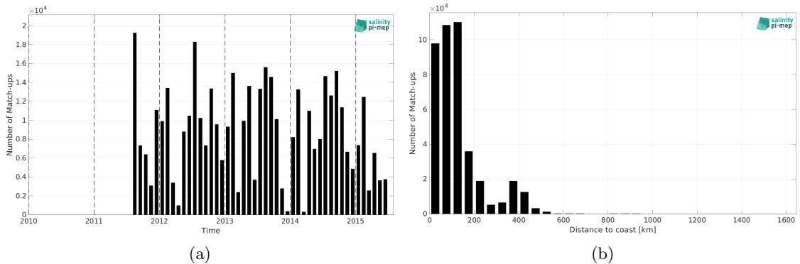
Figure 2: Number of match-ups between ICES and Aquarius SSS L3 OR v5 - Monthly - Rain mask (NASA-GSFC) SSS as a function of time (a) and as function of the distance to coast (b) over the Atlantic Ocean Pi-MEP region and for the full satellite product period.
